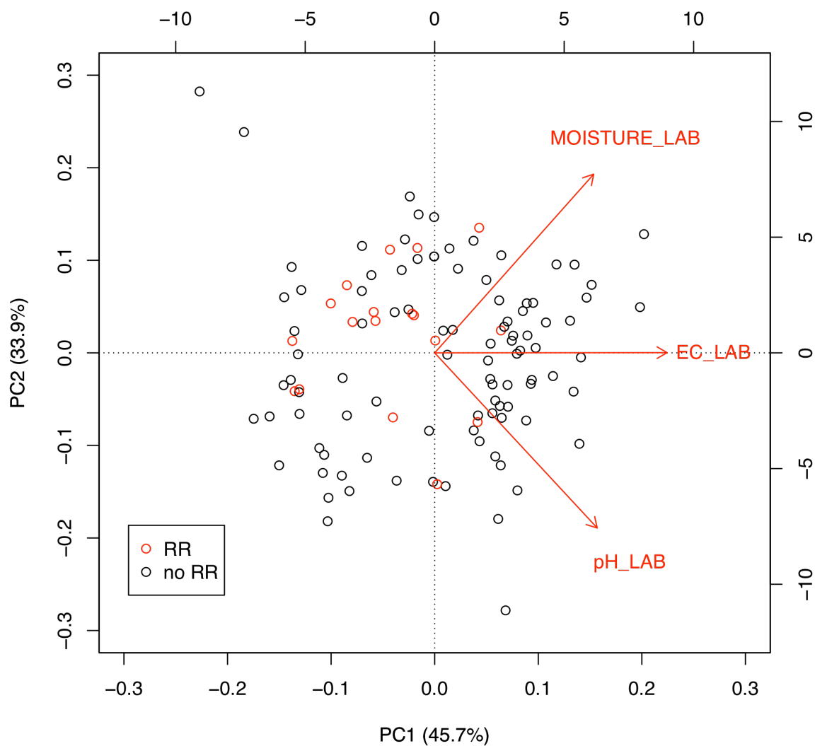
Figure 2.10. Principle Components Analysis of abiotic factors. Plot shows sampling sites plotted on PC1 and PC2. Sites where lhásem ( F. camschatcensis ) RR (riceroot) was found in the Squamish Estuary are shown in red and sites where it was not present are shown in black. Red arrows show the loading of abiotic factors at each PC in connection to the presence and absence data for lhásem .
