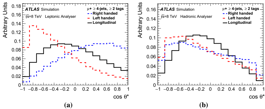
Fig. 3 Templates of the \cos \theta^* distributions for the individual helicity fractions in the \mu + jets channel with \geq 2 b -tags for the a leptonic and b hadronic analyser
