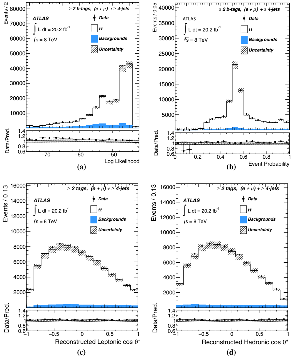
Fig. 2 Measured and predicted distributions of a likelihood and b event probability from the kinematic fit and reconstructed \cos \theta^* distribution using c the leptonic and d the hadronic analysers with \geq 2 b -tags. The displayed uncertainties represent the Monte Carlo statistical uncertainty as well as the background normalisation uncertainties
