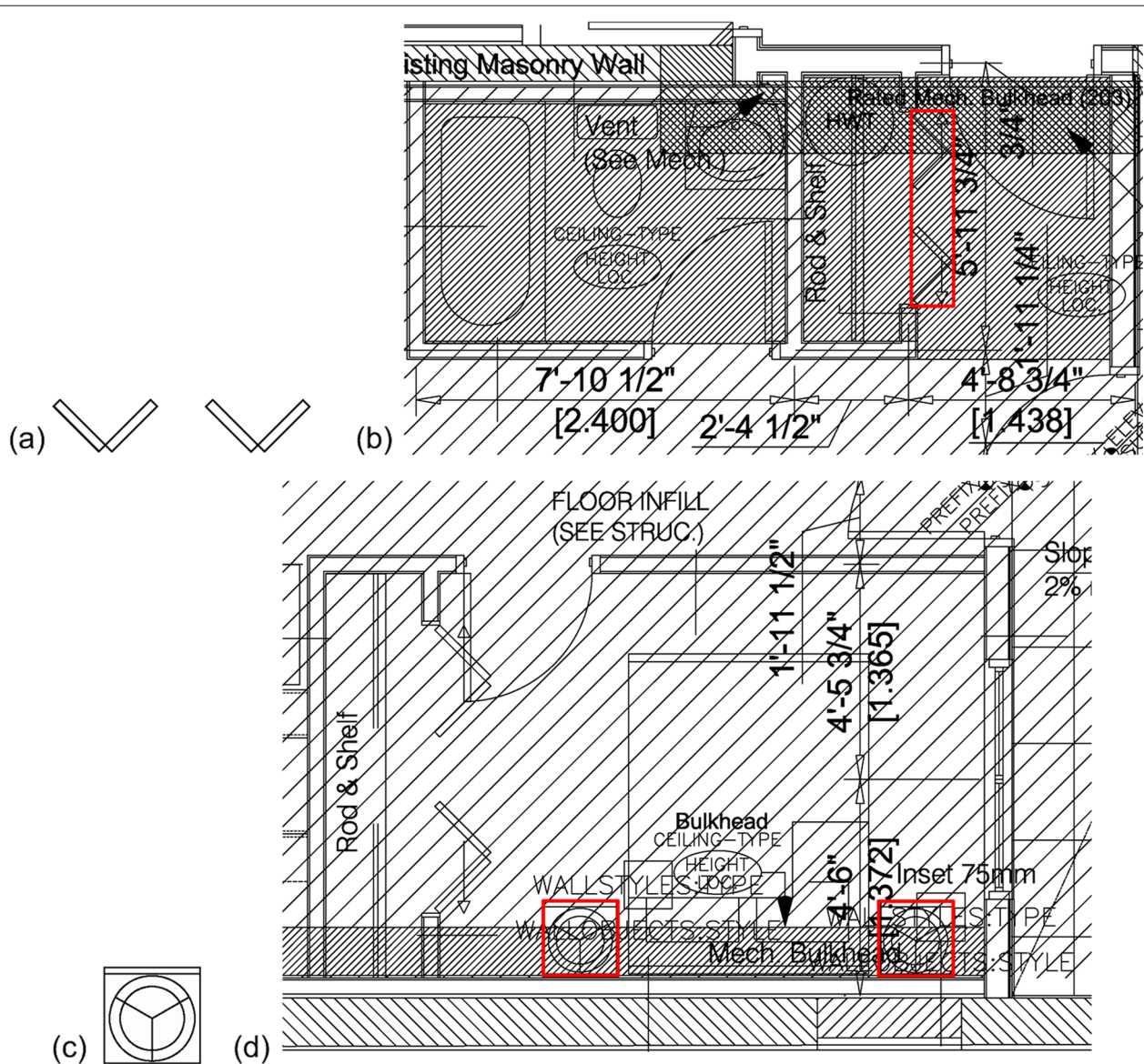
Fig. 11 Sample visual results on real-life architectural drawings, part 2. Sample visual results of the proposed symbol spotting approach on real-life, cluttered architectural drawings from a renovation project of an old heritage building: bi-fold closet doors (a) and nightstand (c) query symbols, and corresponding architectural drawings with spotted instances (b, d)
