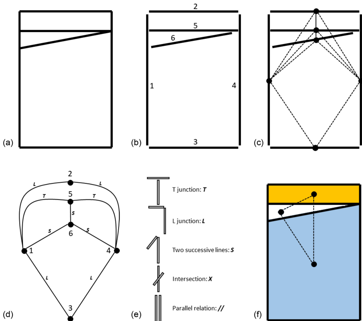
Fig. 4 Graph-based descriptions of a bed symbol. Bed symbol from SESYD (a), vectorized image (b), Fully Visibility Graph (FVG) (c), Attributed Relational Graph (ARG) (d), intersection types used for ARG (e), and Region Adjacency Graph (RAG) (f)
