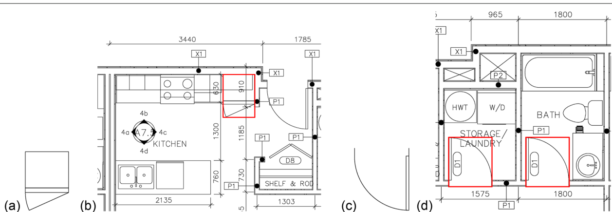
Fig. 10 Sample visual results on real-life architectural drawings, part 1. Sample visual results of the proposed symbol spotting approach on real-life, cluttered architectural drawings from a new construction project: refrigerator (a) and door (c) query symbols, and corresponding architectural drawings with spotted instances (b, d)
