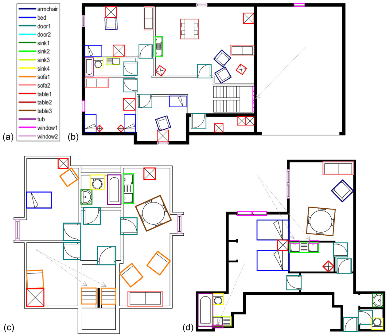
Fig. 8 Sample visual results on GREC contest dataset, part 2. Sample visual results of the proposed symbol spotting approach on the GREC contest dataset [5], ideal case, for a correlation threshold TH = 0.875 . Color legend (a) and spotted symbols on images 1 (b), 8 (c), and 19 (d). In all examples, all symbols were correctly detected, along with six (b), two (c), and three (d) false positives, shown by dashed gray arrows
