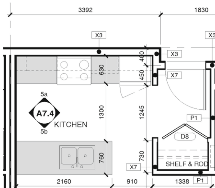
Fig. 1 Architectural floor plan example. Part of an architectural floor plan (kitchen and foyer areas of a residential dwelling unit)
