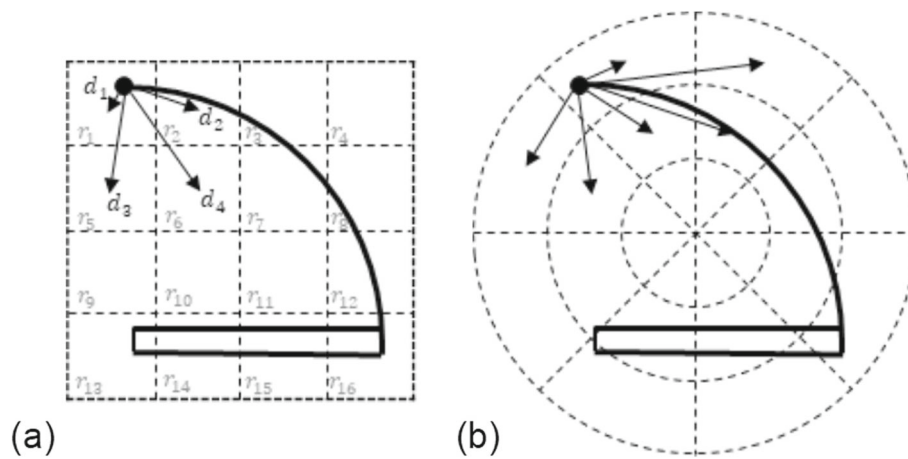
Fig. 3 Pixel-based descriptors. Grid structures of BSM (a) and CBSM (correlogram) (b) for describing a door symbol. Each boundary pixel votes based on its distance to the adjacent points
