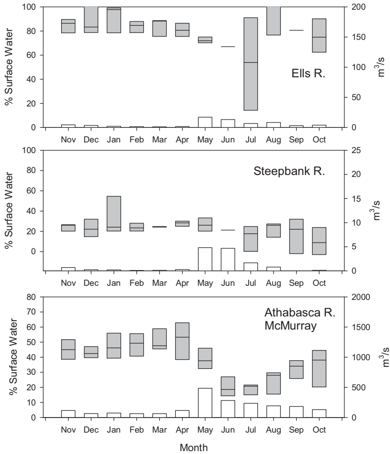
Fig. 11. Partitioning results for % surface water and surface water flow ( \text{m}^3/\text{s} ) showing inter-annual variability by month. Ells R. and Steepbank R. are examples of surface- and groundwater-dominated tributaries, respectively. While comparatively meaningful proportions below 0% and above 100% suggest limitations with our quantitative mixing model.
