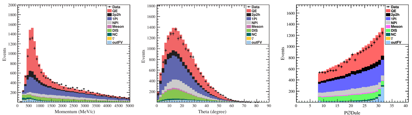
FIG. 3. FHC beam CCINC \nu_\mu event candidate distributions of the \mu^- momentum in MeV/c (left), the muon \theta_\mu angle in degrees (middle), and interaction vertex position by P \emptyset Dule (right). Note backgrounds in the CCINC sample are the NC (dark green), \bar{\nu}_\mu induced events (yellow) and the out of fiducial volume events (light blue). There are negligible \bar{\nu}_\mu backgrounds (yellow) in the FHC sample.
