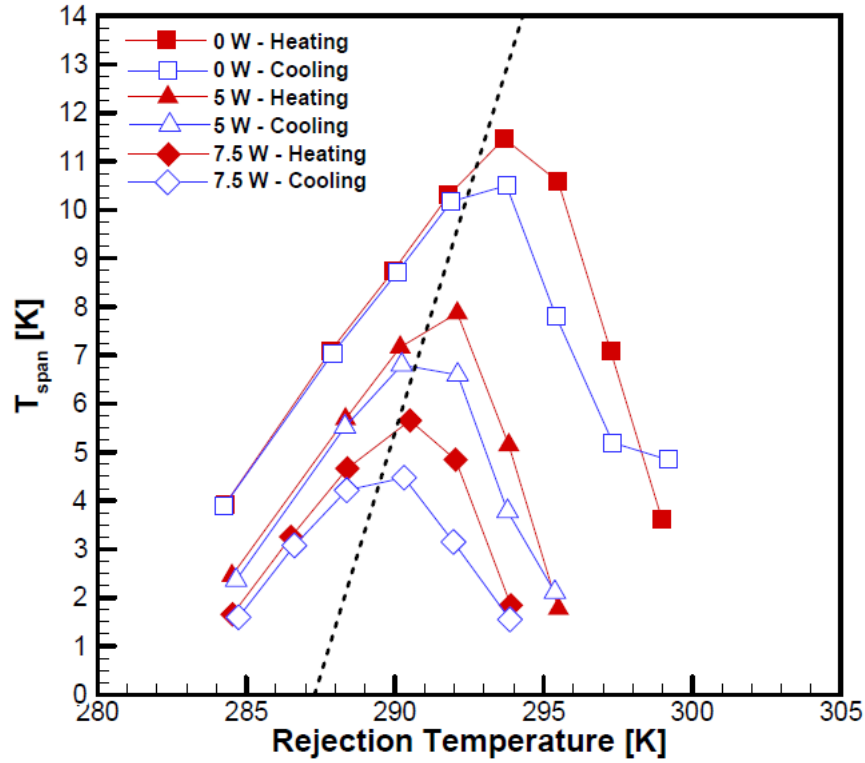
Fig. 24 T_{span} as a function of the rejection temperature and applied load for 3-layer regenerator with lower \Delta T_{ad} intermediate layer.
