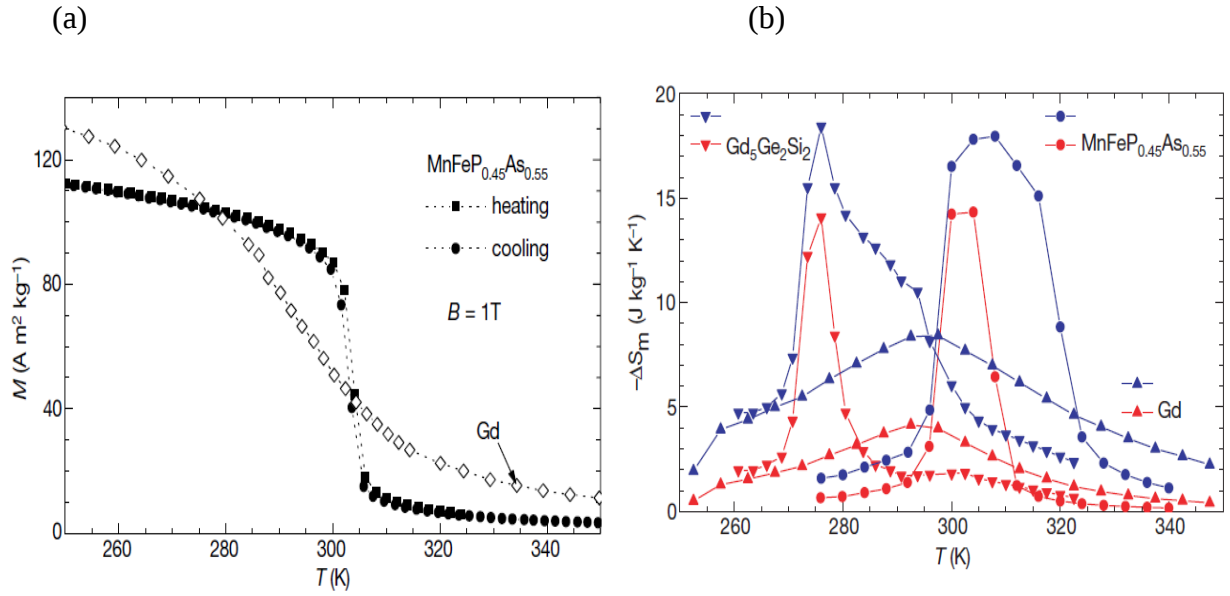
Fig. 8 SOM and FOM properties: (a) Magnetization as a function of the temperature, for a magnetic field variation of 1 T [29]; (b) Magnetic entropy change as a function of the temperature at magnetic field change of 0 to 2 T and 0 to 5 T [29].
