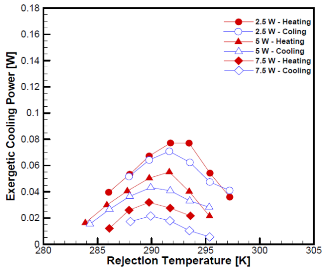
Fig. 26 \dot{E}x_Q as a function of the rejection temperature and applied load for the 2-layer regenerator.
