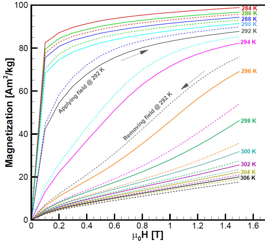
Fig. 14 Magnetization as a function of the magnetic field at different temperatures. The solid lines stands to applying field process and the dashed lines to removing field process.
