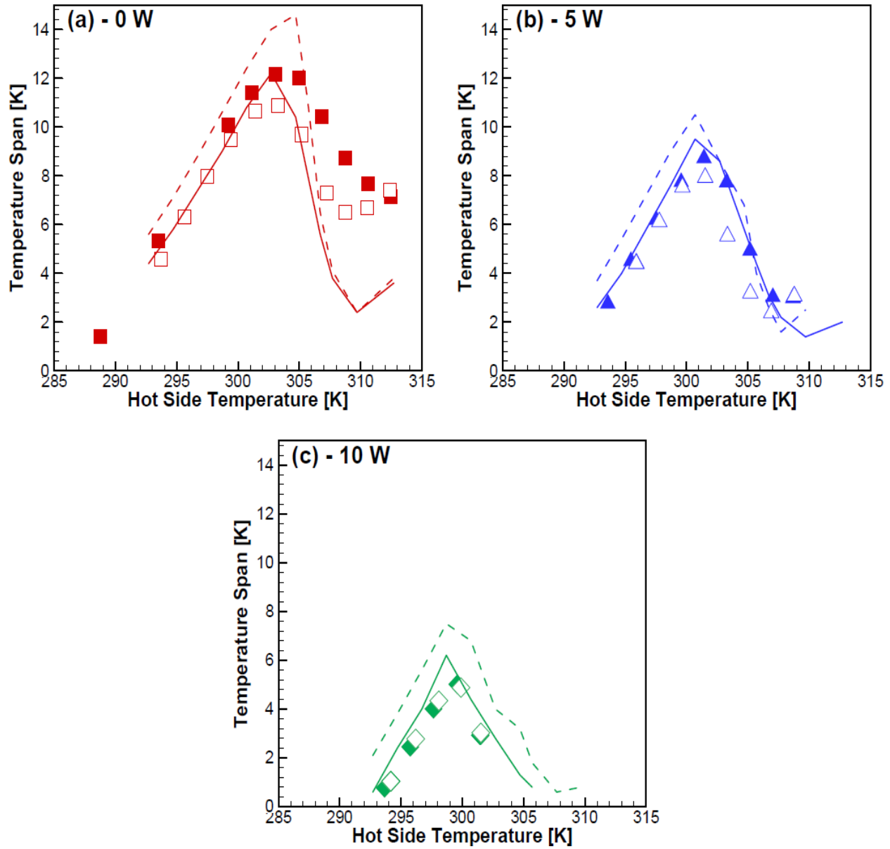
Fig. 42 Comparison between experimental (symbols) and numerical (line) results for \text{MnFeP}_{1-x}\text{Si}_x FOM. The solid line stands for heating-cooling MCE implementation, and the dashed for the average implementation. Different loads conditions are used: (a) no-load condition (0 W); (b) 5 W; (c) 10 W.
