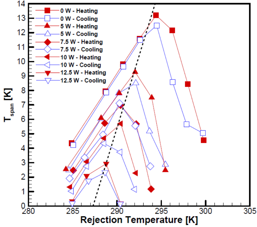
Fig.25 T_{span} as a function of the rejection temperature and applied load for 3-layer regenerator with higher \Delta T_{ad} intermediate layer.
