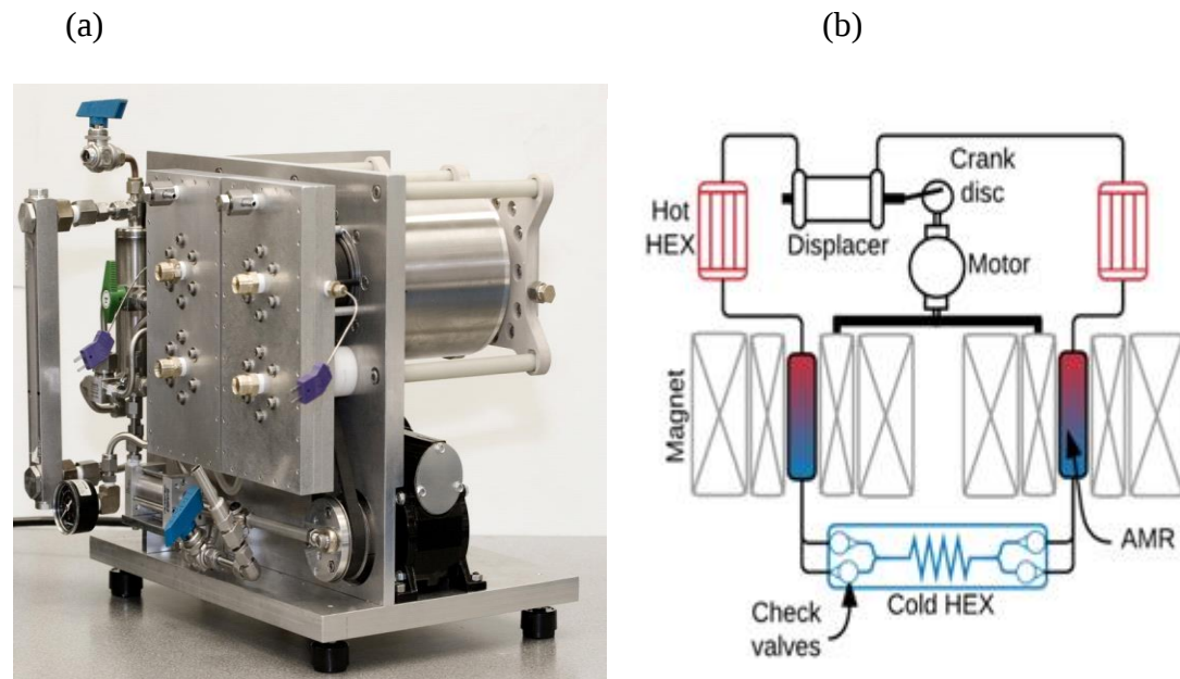
Fig. 10 (a) Photograph of PM I and (b) Schematic diagram of PM I.
