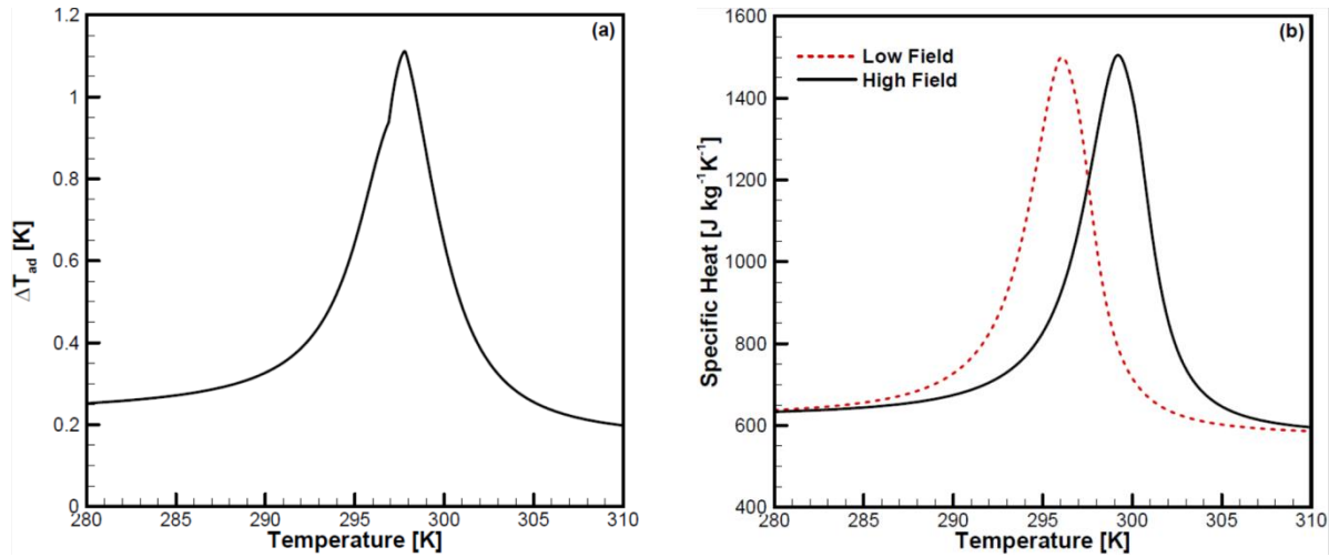
Fig. 39 Simulated a) adiabatic temperature change, b) specific heat of the MnFeP 1-x Si x samples for magnetic field variation of 1.1 T.
