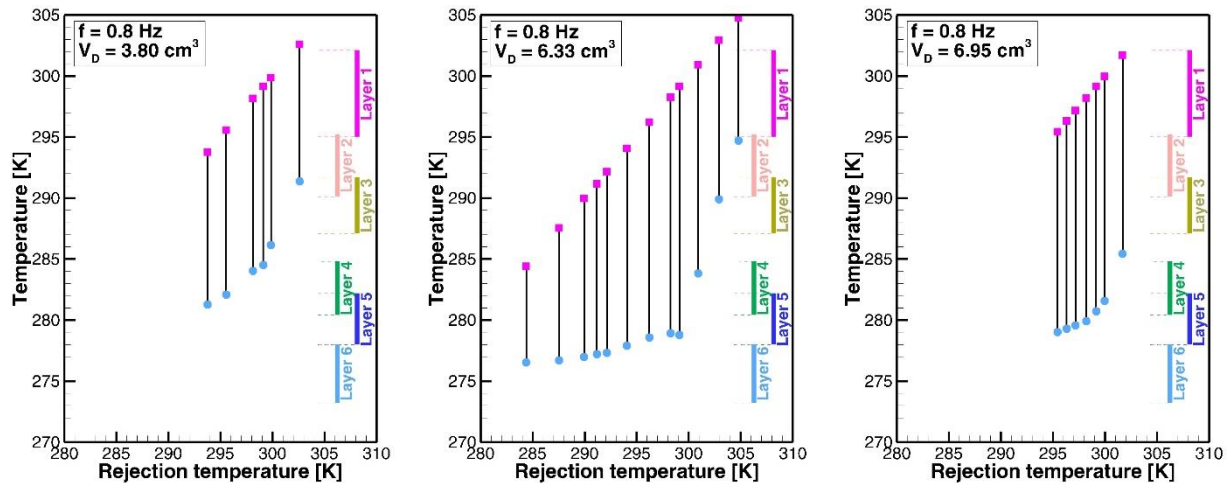
Fig. 36 Six-layer operating temperature range as a function of the rejection temperature for f = 0.8 \text{ Hz} , and V_d = 3.80 \text{ cm}^3 , 6.33 \text{ cm}^3 , and 6.95 \text{ cm}^3 .
