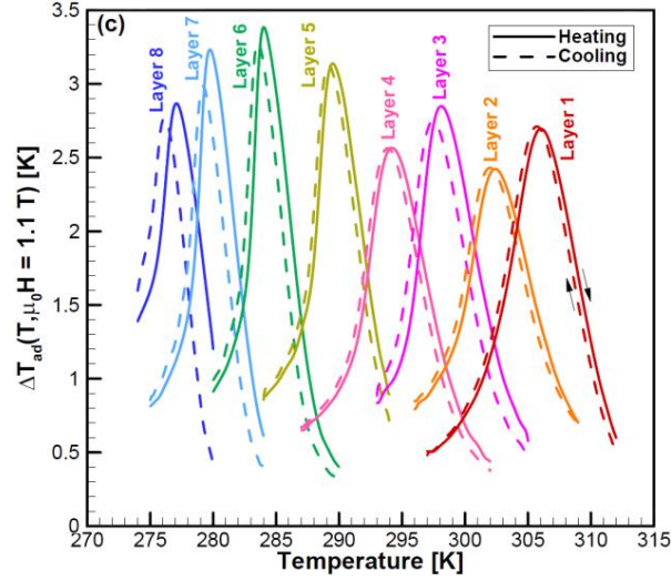
Fig. 31 Direct measured \Delta T_{ad} as a function of the temperature for the three FOM regenerators: (a) 3-layer; (b) 6-layer; (c) 8-layer. The direct measurements are performed for heating and cooling protocols with a magnetic field variation of 0-1.1 T
