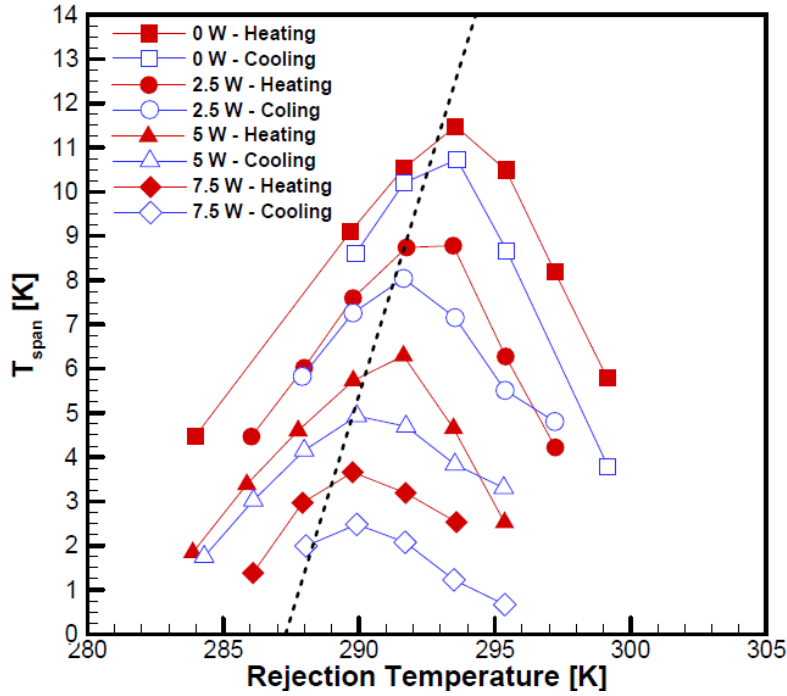
Fig. 23 T_{span} as a function of the rejection and applied load for 2-layers regenerator.
