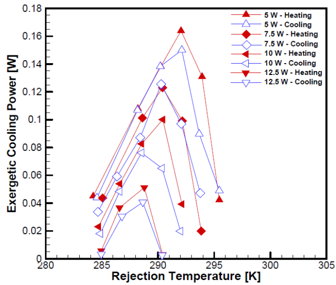
Fig. 28 \dot{Ex}_Q as a function of the rejection temperature and applied load for the 3-layer regenerator with higher \Delta T_{ad} intermediate layer.
