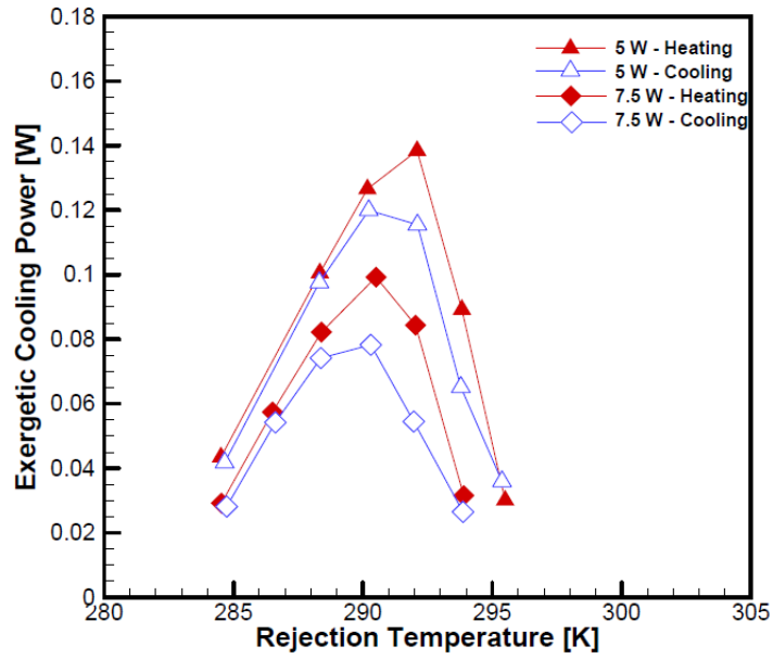
Fig. 27 \dot{Ex}_Q as a function of the rejection temperature and applied load for the 3-layer regenerator with lower \Delta T_{ad} intermediate layer.
