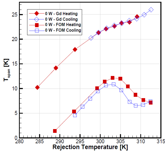
Fig. 20 A comparison of the maximum temperature span as a function of the rejection temperature for the Gd and \text{MnFeP}_{1-x}\text{Si}_x beds at no heat load conditions.
