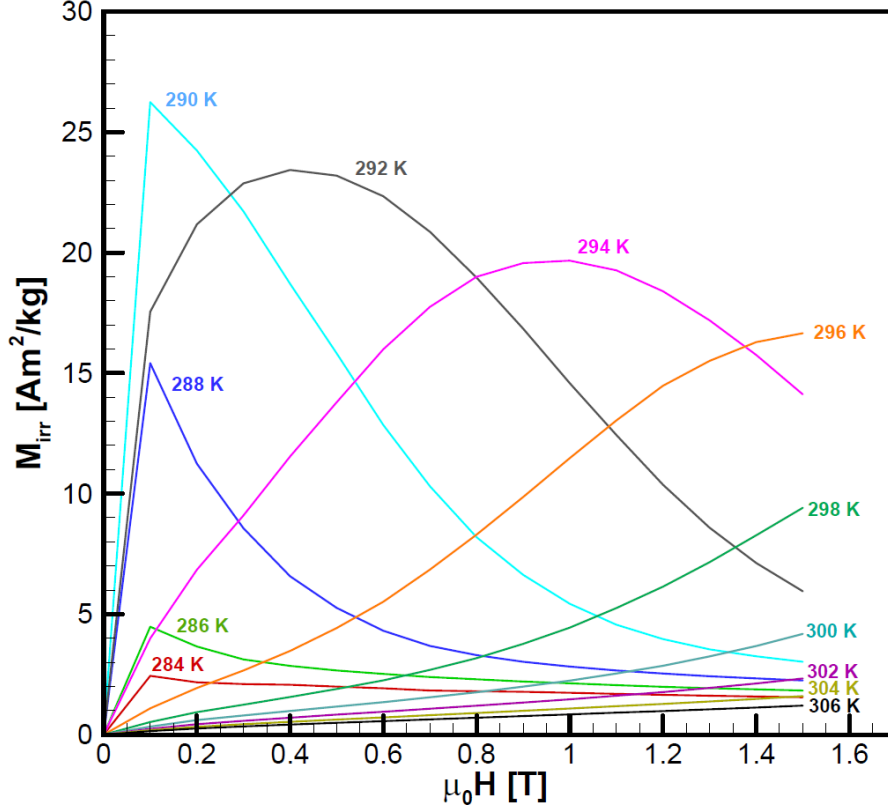
Fig. 15 Irreversible magnetization as a function of the magnetic field at different temperatures.
