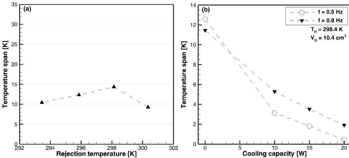
Fig. 32 Three-layer results. (a) No-load temperature span as a function of the rejection temperature for f = 0.8 Hz and V_d = 10.4 cm 3 ; (b) Temperature span as a function of the cooling capacity for V_d = 10.4 cm 3 , T_H = 298.4 K, and f = 0.5 Hz and 0.8 Hz.
