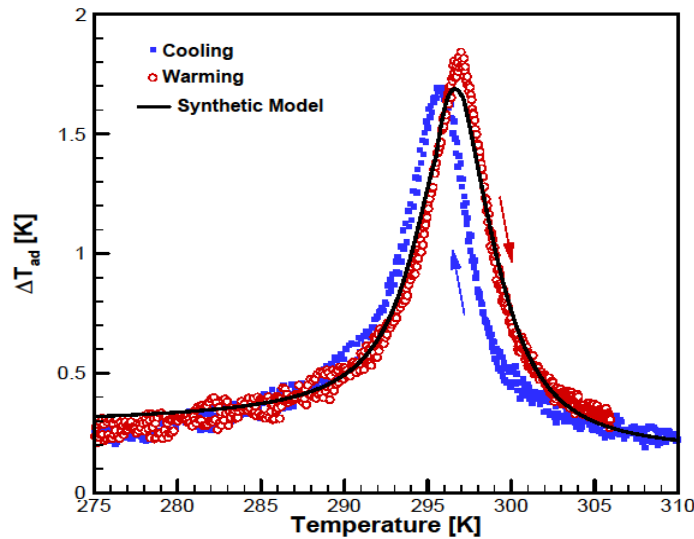
Fig. 38 Direct measured adiabatic temperature change as a function of the temperature, for the \text{MnFeP}_{1-x}\text{Si}_x AMR are performed for heating and cooling protocols with properties magnetic field variation of 1.1 T.
