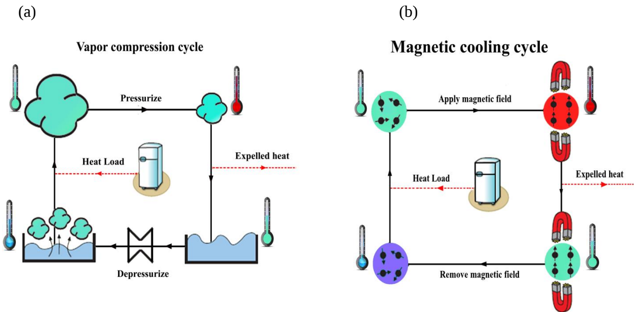
Fig. 1 Cooling cycles. (a) The Conventional vapor compression cycle and (b) Magnetic cooling cycle. Adapted from Ichiro Takeuchi and Karl Sandeman [14].
