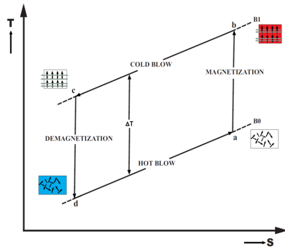
Fig. 5 Schematic T-S diagram of AMR cycle.
