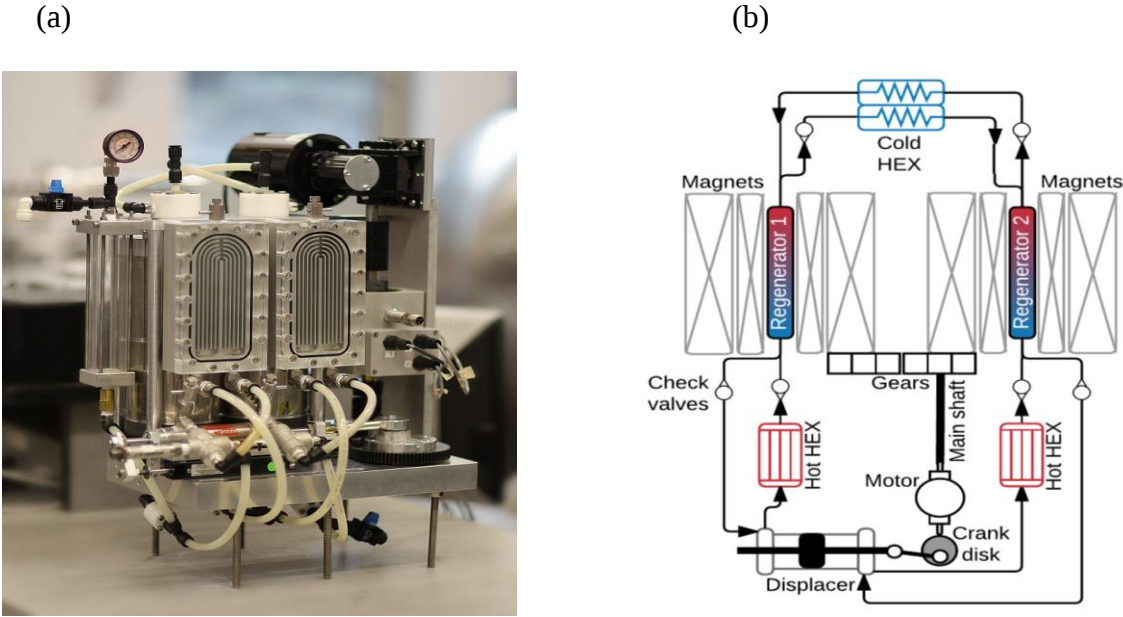
Fig. 11 (a) Photograph of PM II and (b) Schematic diagram of PM II.
