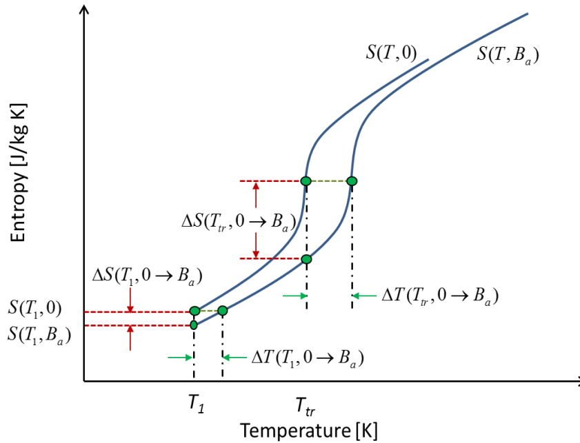
Fig. 7 Entropy variation with field and temperature for a FOM. Isothermal entropy change and adiabatic temperature change depend upon temperature and the magnitude of the change in applied magnetic field, B_a = \mu_0 H_a . Maximum values are found near the transition temperature, T_{tr} .
