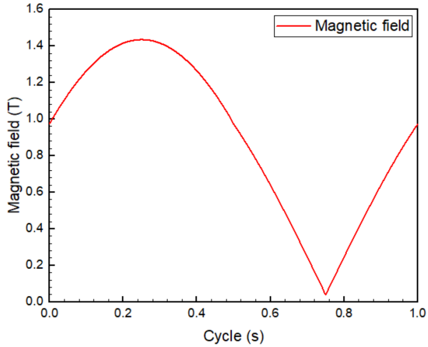
Fig. 17 Sinusoidal experimental field profile with the PM1 device for the high and low field values as a function of time.
