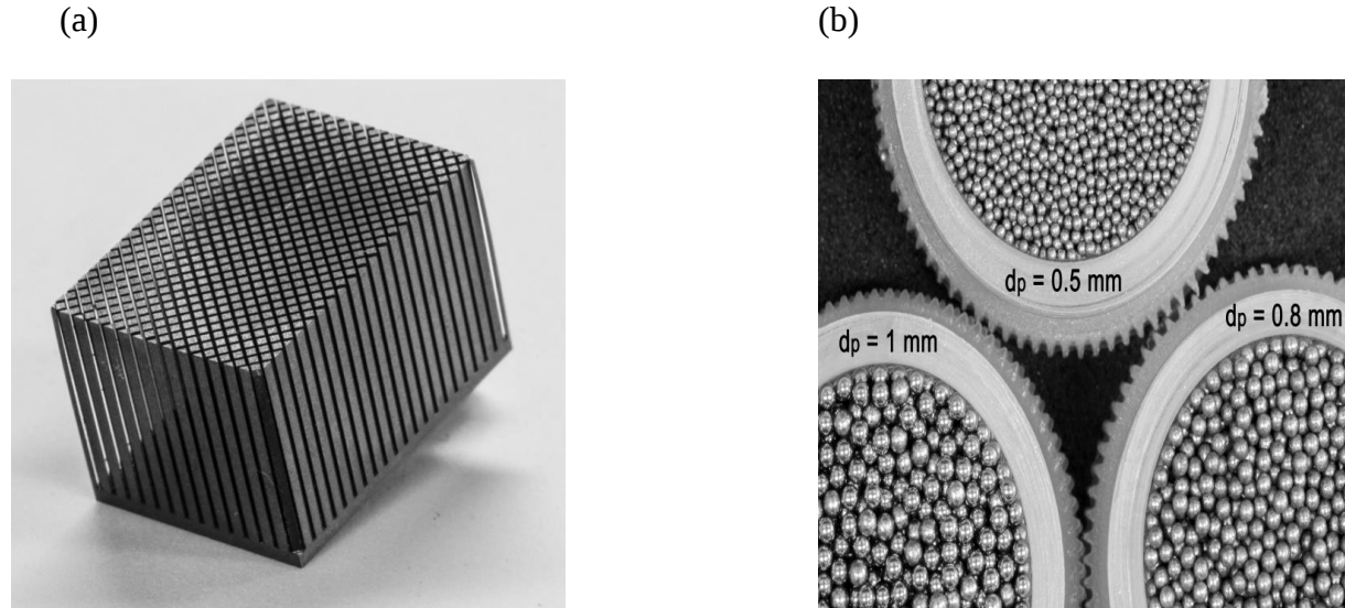
Fig. 3 (a) Pin array and (b) Packed sphere regenerator matrices [27].
