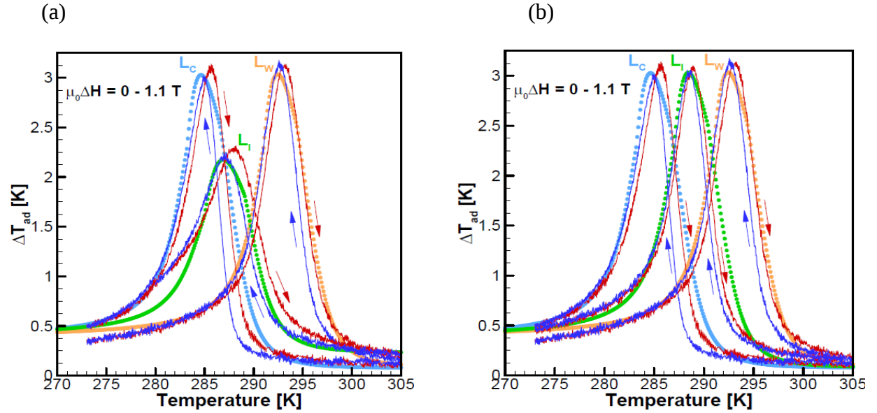
Fig. 22 Adiabatic temperature change as a function of temperature for MnFeP1-xAsx (a) directly measured \Delta T_{ad} data for the case where the intermediate layer has a lower \Delta T_{ad} ; (b) directly measured \Delta T_{ad} data for the case where the intermediate layer has a higher \Delta T_{ad} . The magnetic field changes from 0 to 1.1 T, and heating (red) and cooling (blue) measurements are shown. Solid lines are model data.
