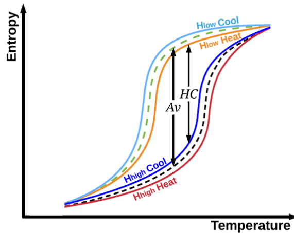
Fig. 16 Schematic drawing showing the two different implementations of the MCE for FOM: using the an average curve (dashed lines) between the cooling and heating curves; using the low field heating and the high field cooling curves.
