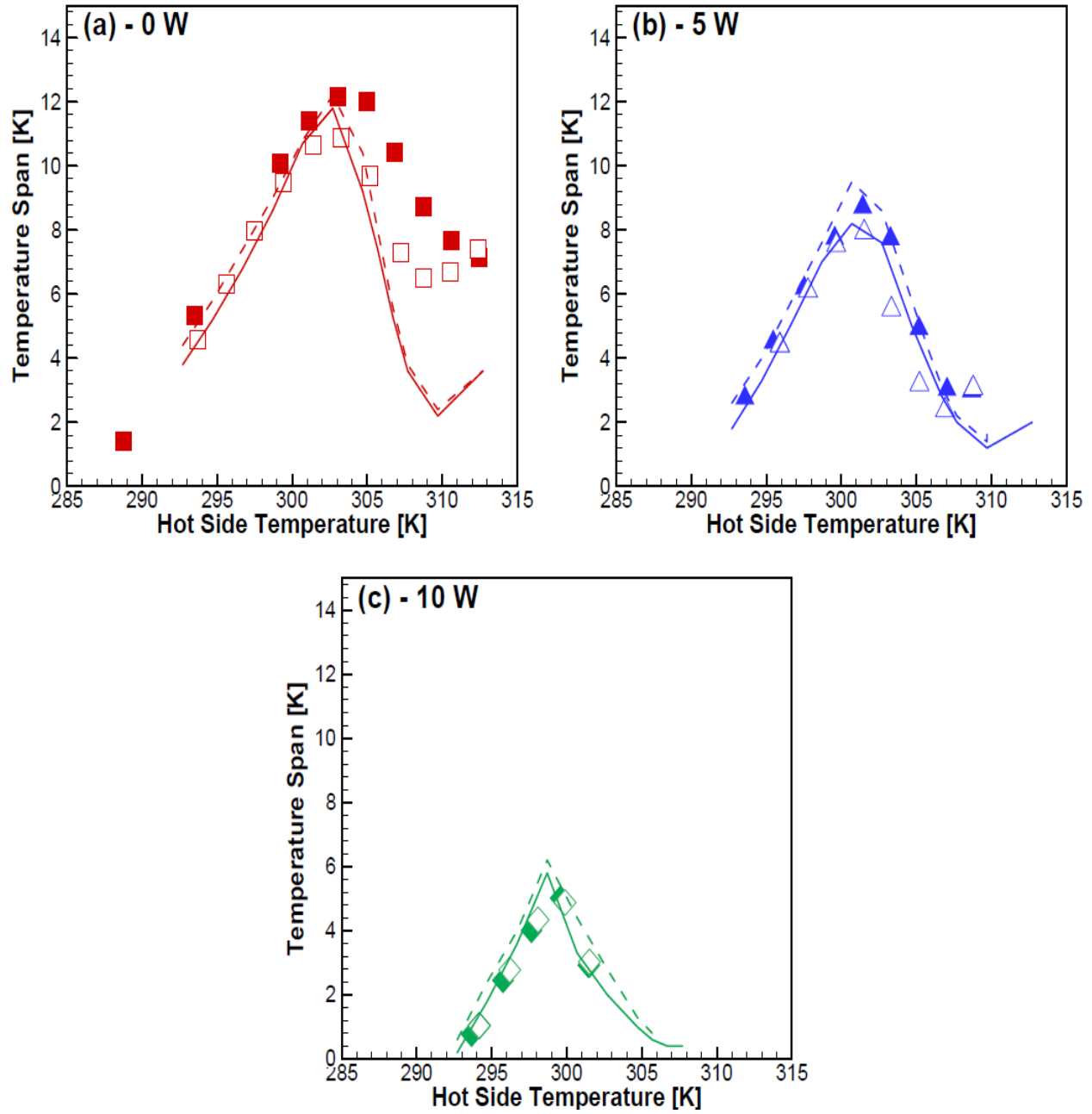
Fig. 43 Comparison between experimental (symbols) and numerical (line) results for MnFeP1-xSix FOM. The solid lines stands for simulations with magnetic hysteresis, and the dashed for simulations without magnetic hysteresis. Different loads conditions are used: (a) no-load condition (0 W); (b) 5 W; (c) 10 W.
