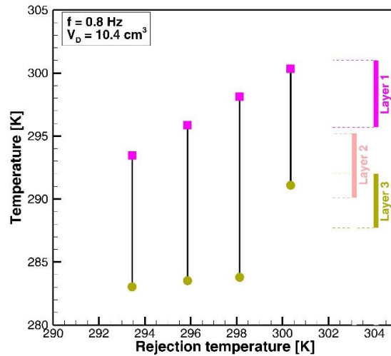
Fig. 35 Regenerator operating temperature range as a function of the rejection temperature for the 3-layer regenerators at a fixed operating condition.
