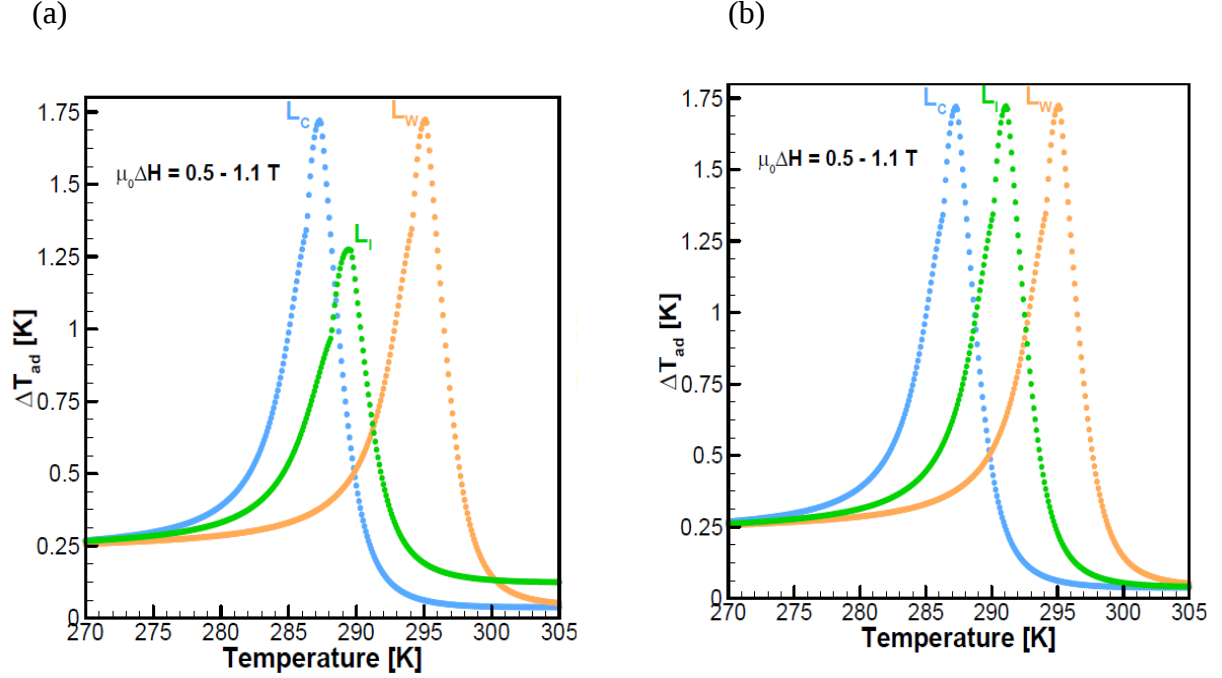
Fig. 29 Adiabatic temperature change as a function of temperature for MnFeP 1-x As x for a magnetic field change from 0.5 T to 1.1 T. (a) low \Delta T_{ad} middle layer (b) high \Delta T_{ad} middle layer.
