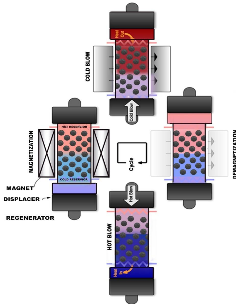
Fig. 4 Schematic representation of AMR cycle consists of four processes. Adapted from P.V.Trevizoli [27].
