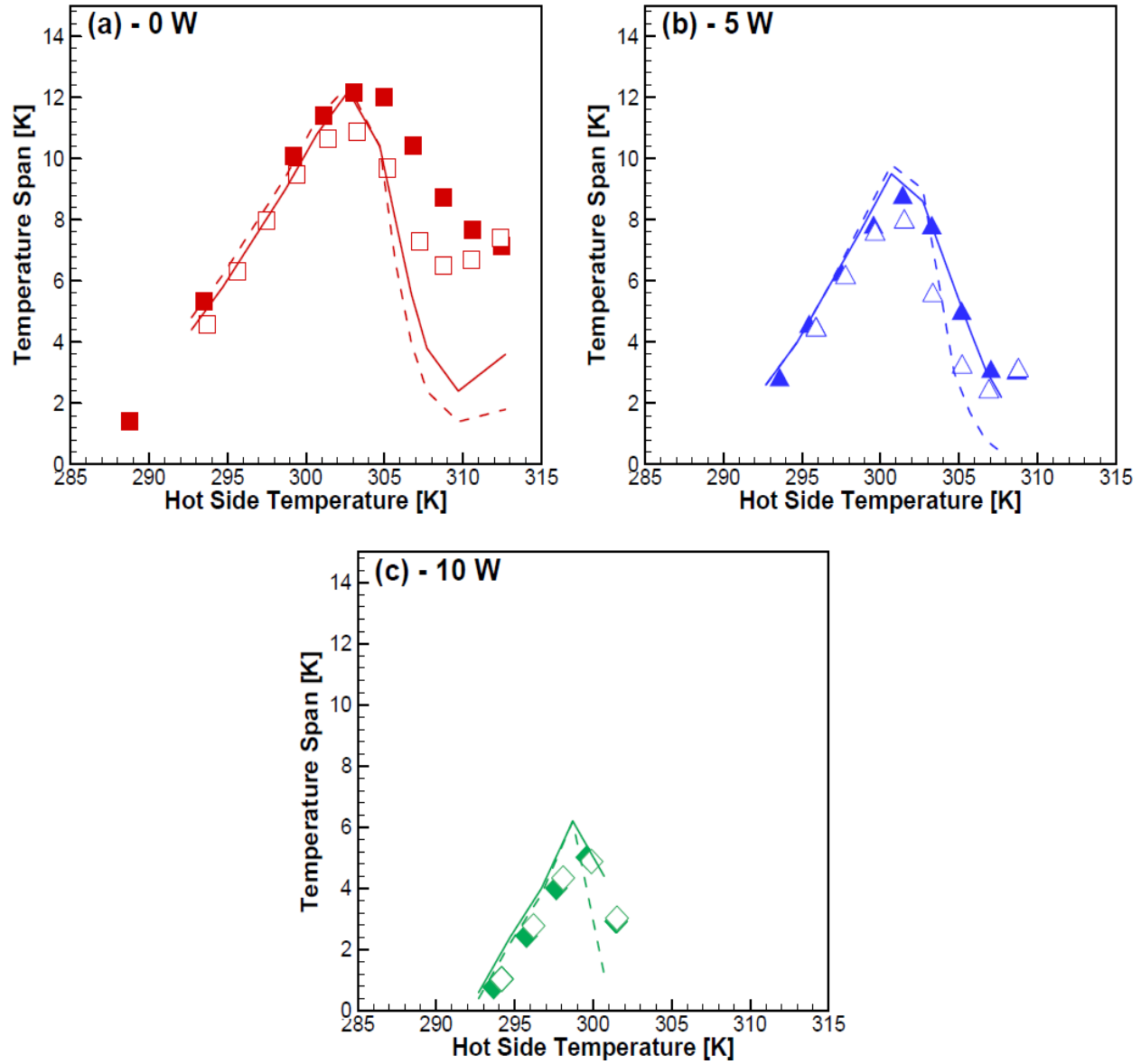
Fig. 41 Comparison between experimental (symbols) and numerical (line) results for MnFeP 1-x Si x FOM. The solid line stands for with heat leaks and the dashed lines without heat leaks. Different loads conditions are used: (a) no-load condition (0 W); (b) 5 W; (c) 10 W.
