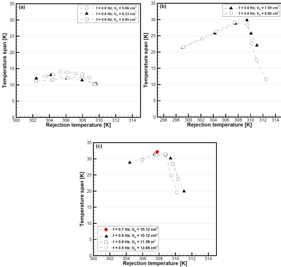
Fig. 34 Zero-load temperature span as a function of the rejection temperature for: (a) short bed - f = 0.8 Hz, and V_d = 5.06 cm 3 , 6.33 cm 3 , and 6.95 cm 3 ; (b) medium bed - f = 0.8 Hz, and V_d = 7.59 cm 3 , and 8.86 cm 3 ; (c) long bed - f = 0.5 and 0.7 Hz, and V_d = 10.12 cm 3 , 11.39 cm 3 , and 12.65 cm 3 .
