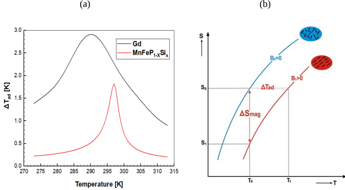
Fig. 2 Gd and MnFeP 1-x Si x properties: (a) Direct measured adiabatic temperature change as a function of the temperature, for a magnetic field variation of 1.1 T; (b) a schematic representation of adiabatic temperature change and magnetic entropy change in the entropy-temperature state space.
