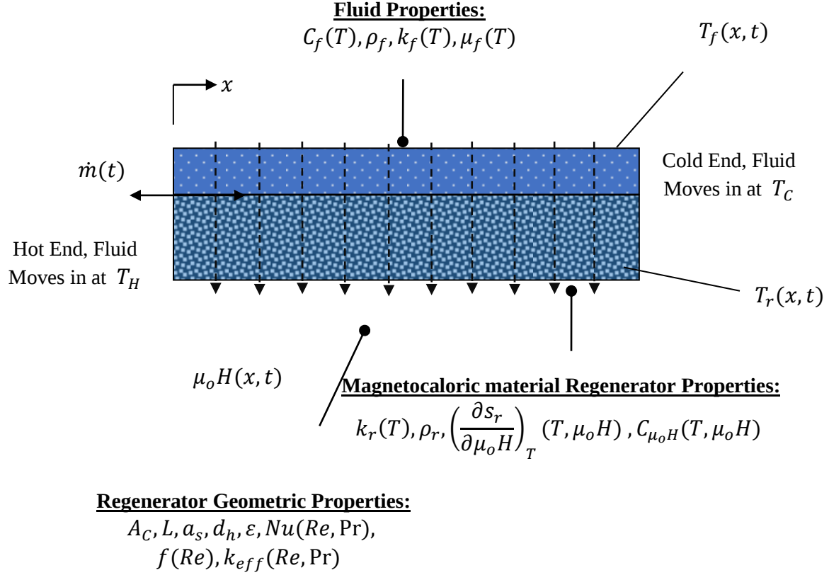
Fig. 13 Schematic diagram of 1-D AMR model with input parameters for both the fluid and the regenerator.
