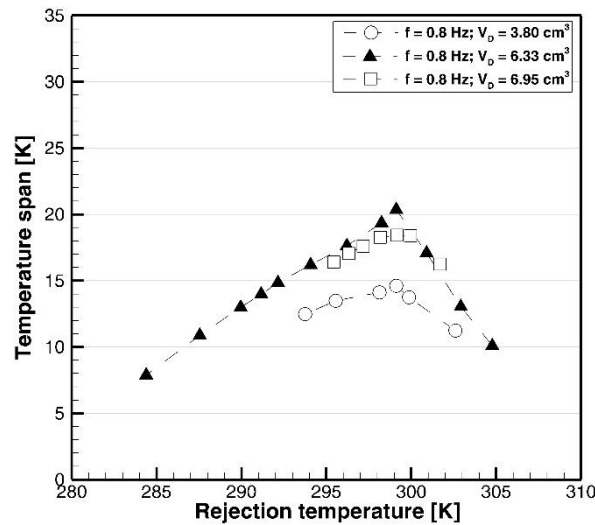
Fig. 33 Six-layer zero-load temperature span as a function of the rejection temperature for f = 0.8 Hz, and V_d = 3.80 \text{ cm}^3 , 6.33 \text{ cm}^3 , and 6.95 \text{ cm}^3 .
