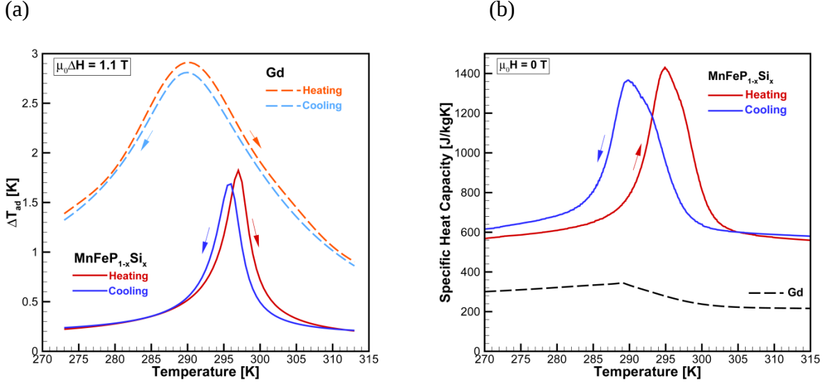
Fig. 19 (a) Direct measured adiabatic temperature change as a function of temperature for Gd and MnFeP 1-x Si x , for an applied field change of 1.1 T; (b) Specific heat capacity as a function of the temperature at 0 T, for MnFeP 1-x Si x alloy and Gd. In both cases the thermal hysteresis is characterized via heating and cooling curves.
