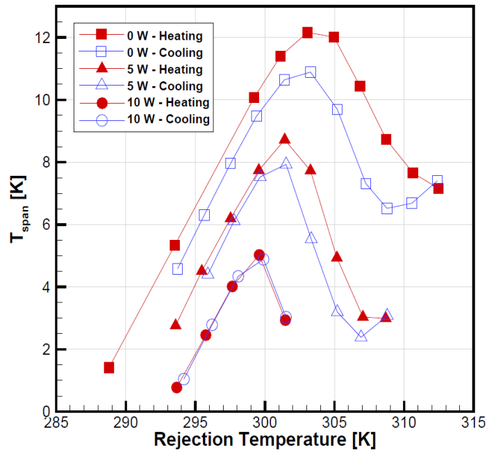
Fig. 21 A comparison of the maximum temperature span as a function of the rejection temperature for the MnFeP 1-x Si x regenerator at 0 W, 5 W and 10 W load conditions.
