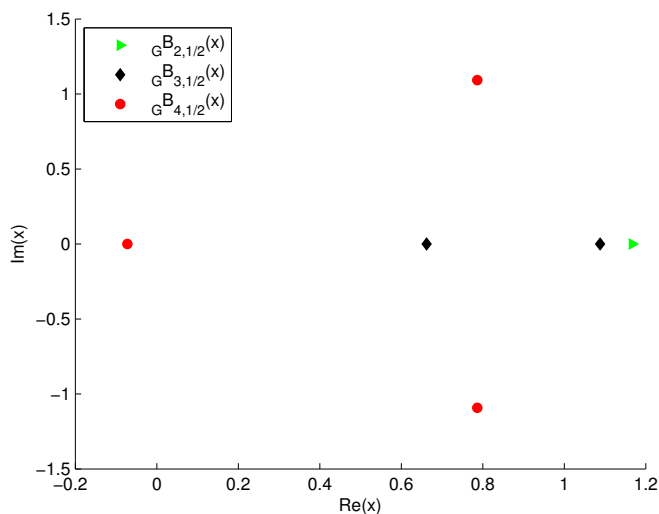
Figure 6. Zeros of G^B_{m,1/2}(x) .
