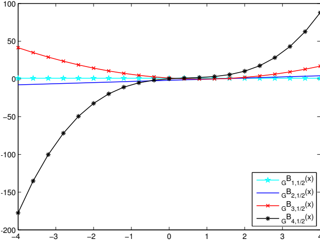
Figure 2. Shape of \mathcal{G}\mathfrak{B}_{m, \frac{1}{2}}(x) .
