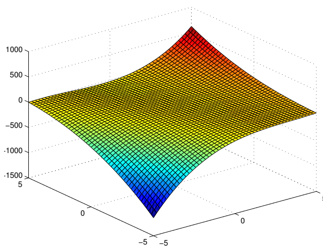
Figure 4. Surface plot of g\mathfrak{B}_{4,\frac{1}{2}}(x_1, x_2) .
