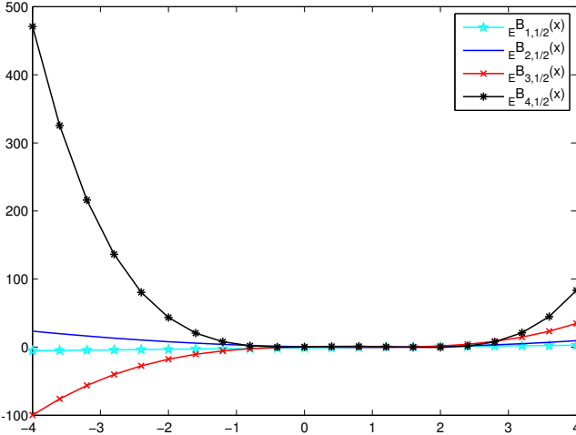
Figure 1. Shape of \mathcal{E}\mathfrak{B}_{m, \frac{1}{2}}(x) .
