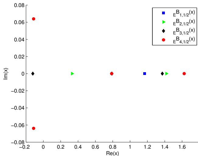
Figure 5. Zeros of E^B_{m,1/2}(x) .
