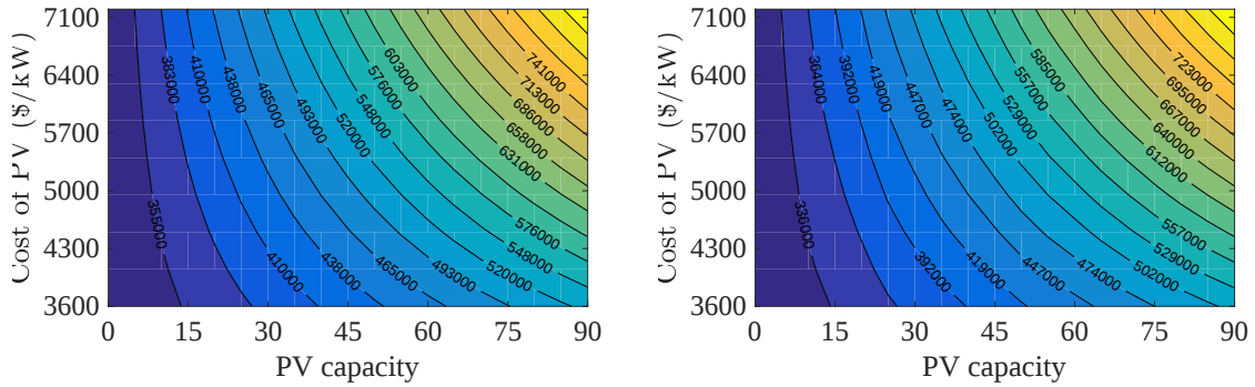
(a) NPC for uncoordinated charging for variable PV capacities and variable PV car port prices in Victoria, BC. (b) NPC for coordinated charging for variable PV capacities and variable PV car port prices in Victoria, BC.
