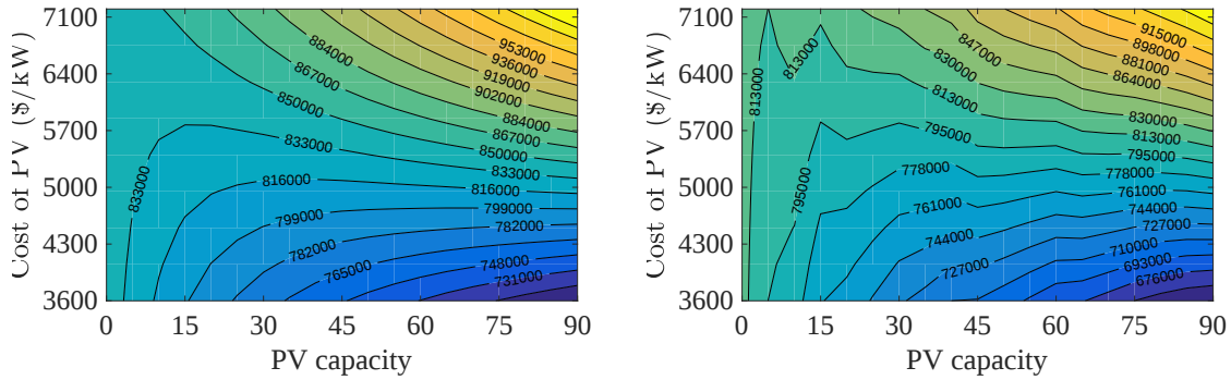
(a) NPC for uncoordinated charging for variable PV capacities and variable PV car port prices in Los Angeles, CA. (b) NPC for coordinated charging for variable PV capacities and variable PV car port prices in Los Angeles, CA.
