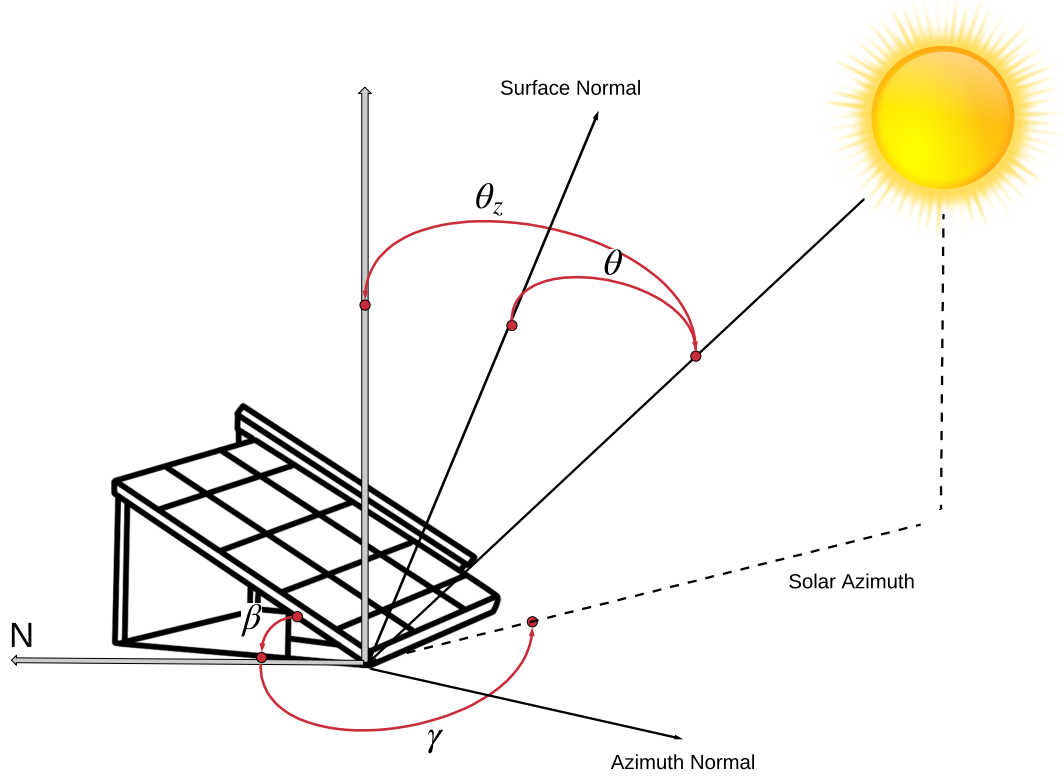
Figure 2.1: Solar panel with terrain and solar angles.
