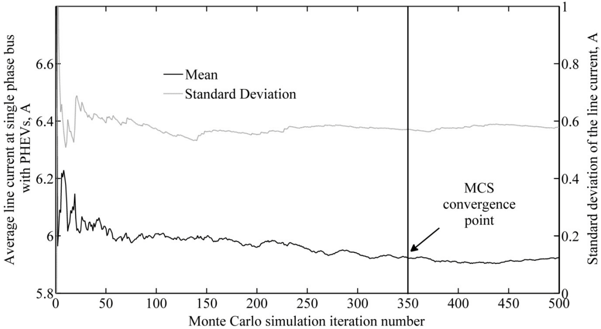
Figure 5.1. Convergence of the mean and standard deviation for the load at a residential single phase bus with PHEVs at 18:00 hours.
