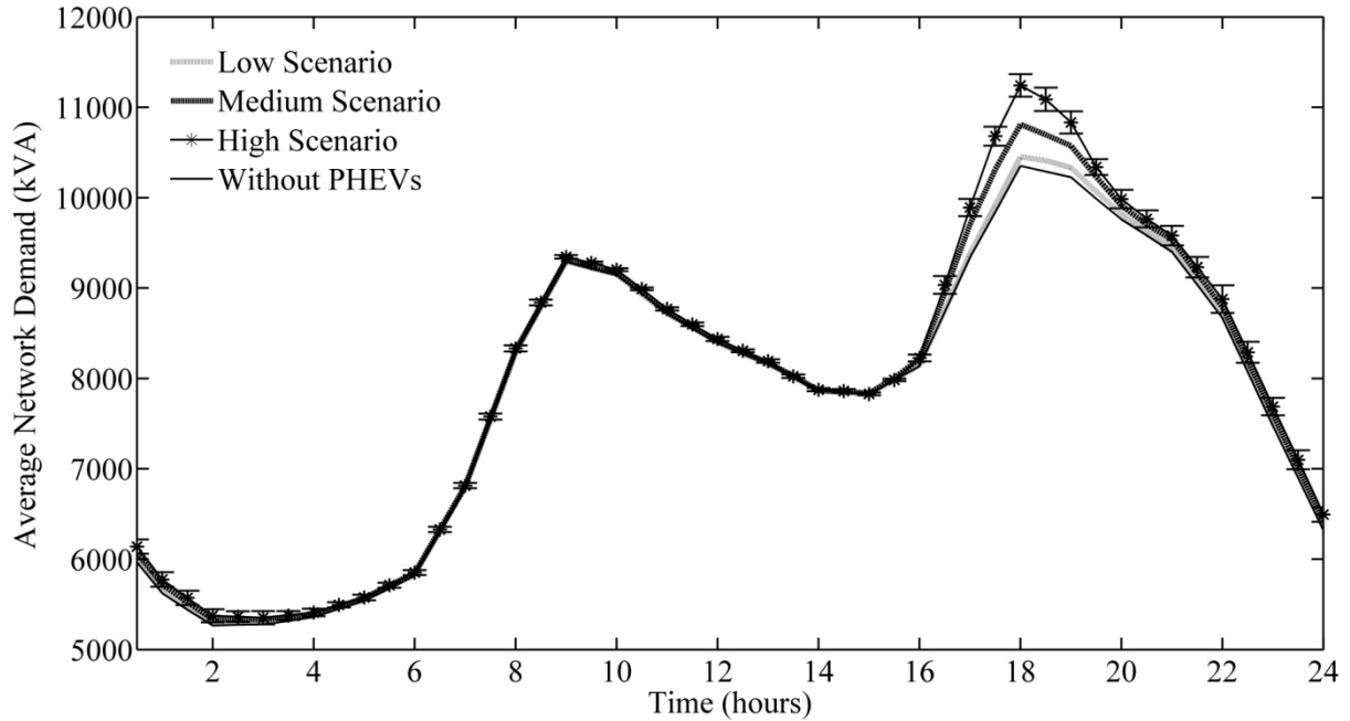
Figure 5.5. Average network demand for the suburban network. Error bars show the maximum and minimum values for the high scenario.
