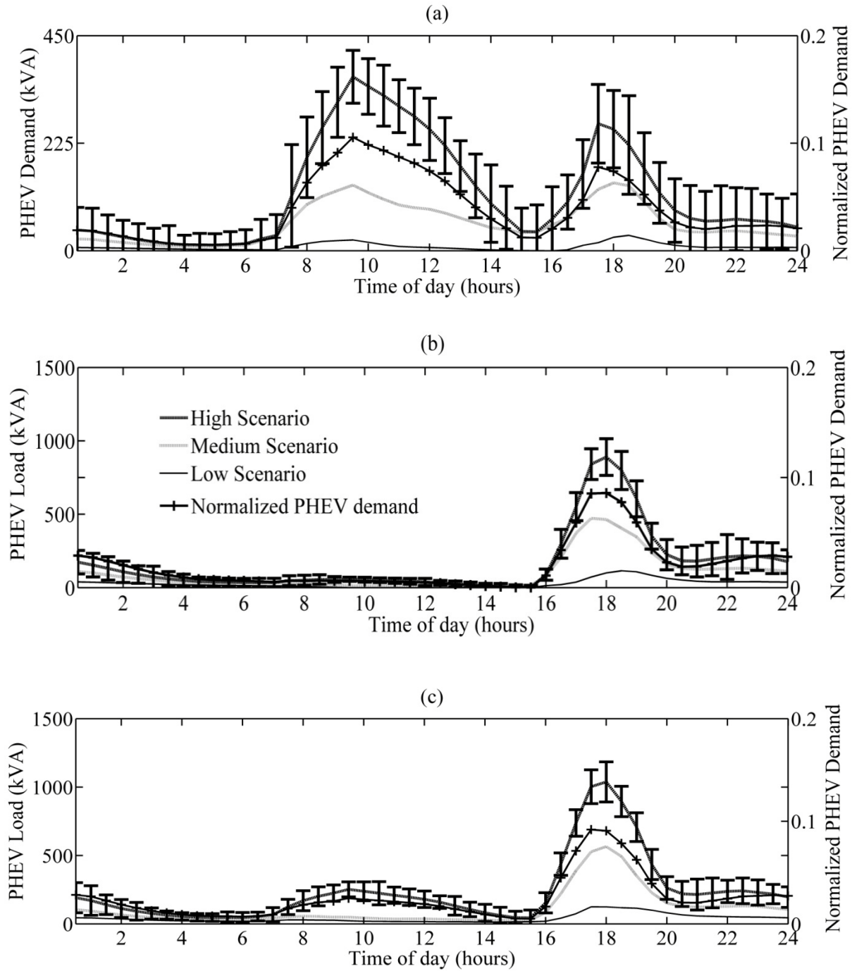
Figure 5.2. Average PHEV demand for each scenario on (a) urban, (b) suburban and (c) rural networks at each time interval. Error bars show the extreme values of maximum and minimum PHEV demand for the high scenario.
