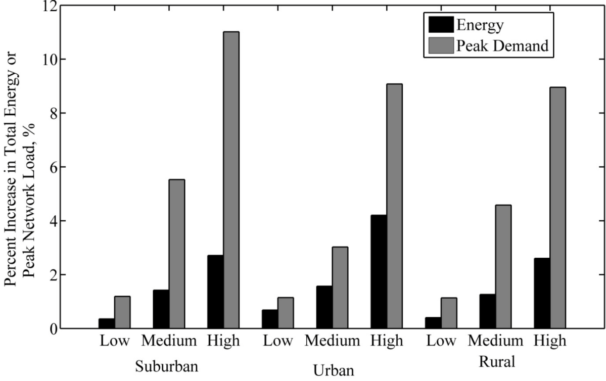
Figure 5.7. Percentage increases in energy and peak demand for all three networks in all scenarios
