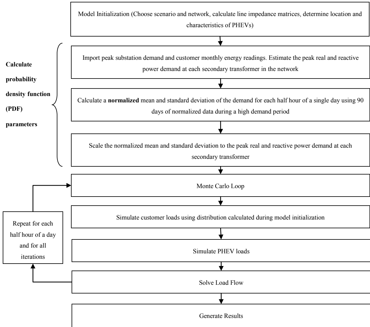
Figure 3.4. PLF model logic flow chart showing process to calculate probability density function parameters for customer load generation
