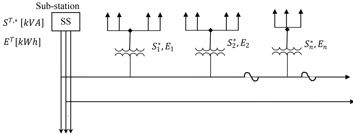
Figure 3.5. Allocation of peak substation demand to secondary transformers
