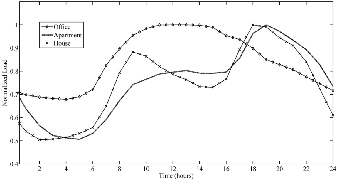
Figure 3.6. Normalized load profiles for apartment, house and office
