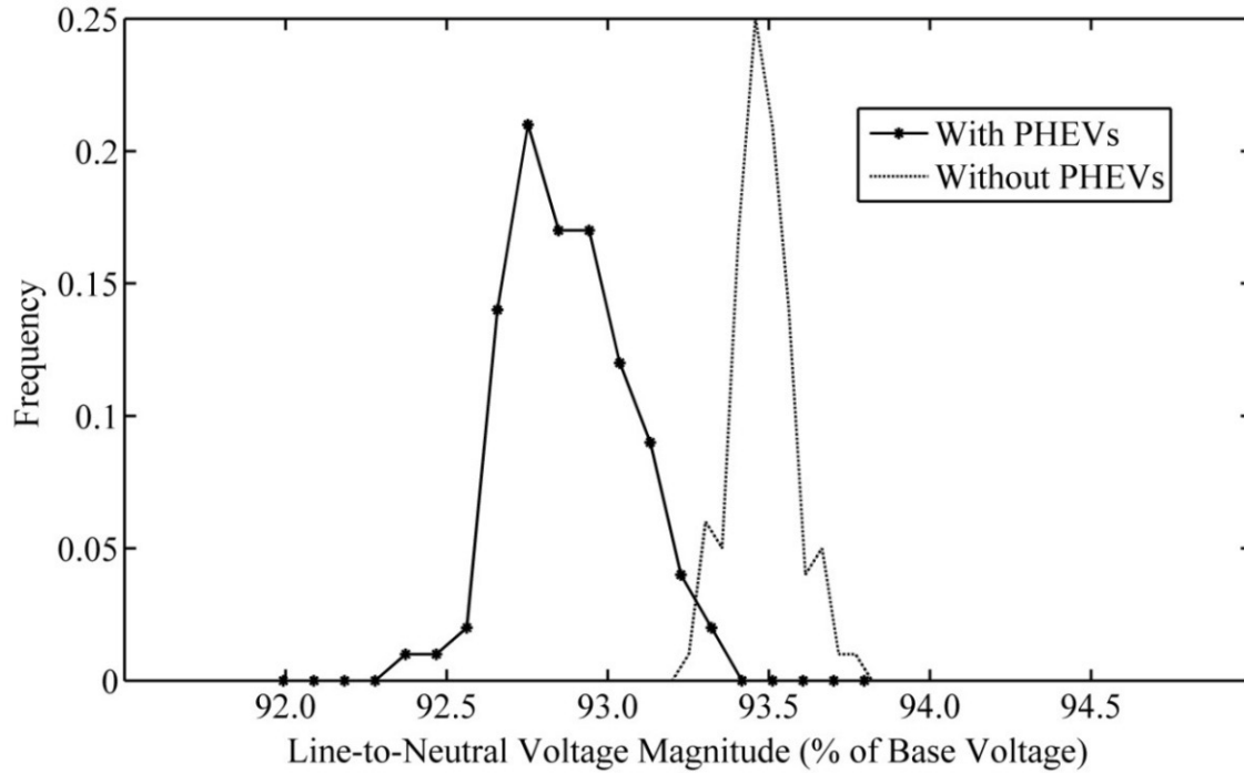
Figure 5.11. Bus voltage distribution for lowest single phase bus voltage on the rural network at 18:00 hours.
