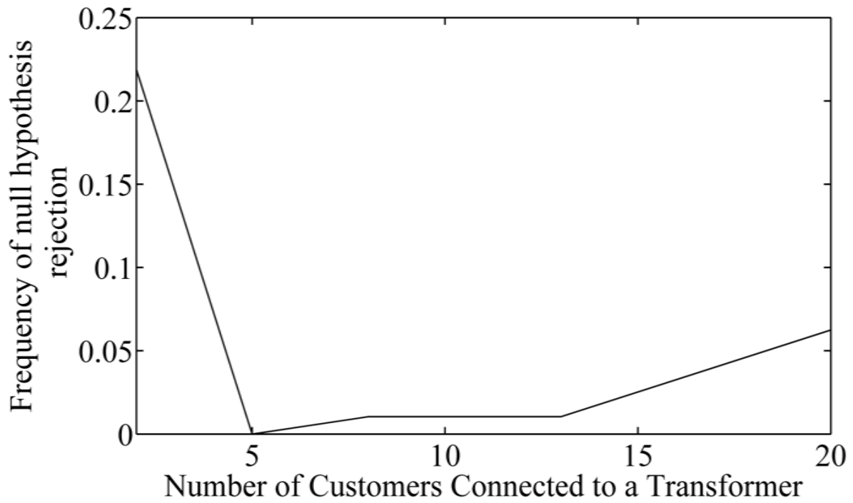
Figure C.1. Frequency of chi-square test null hypothesis rejection for various sized groups of residential customers, 95% confidence level
