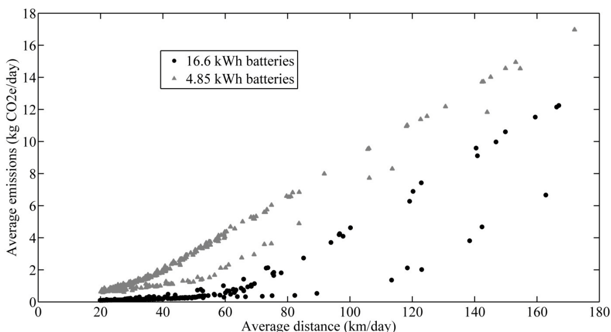
Figure 5.17. Scatter plot of average emissions versus the average daily distance.
