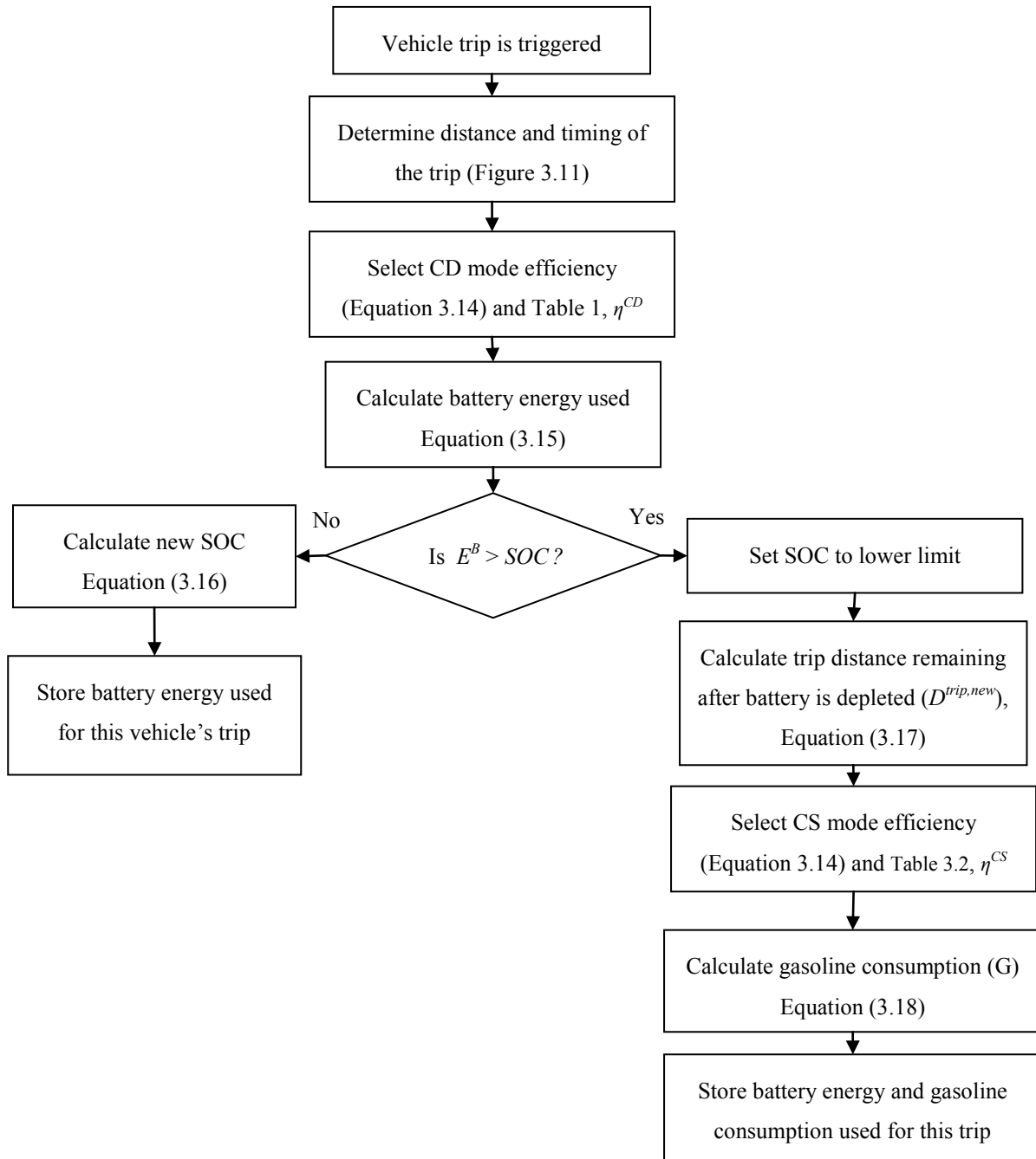
Figure 3.12. Process to calculate gasoline and battery energy used for each vehicle trip
