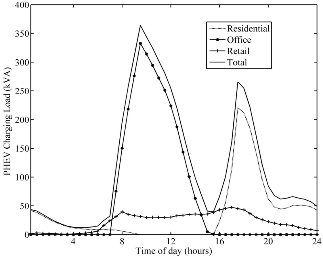
Figure 5.3. Average PHEV demand for scenario 3 on the urban network showing residential, office, retail and total PHEV demand.
