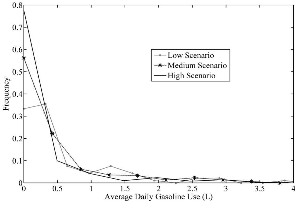
Figure 5.15. Distribution of average gasoline consumption per day for all vehicles in the rural network
