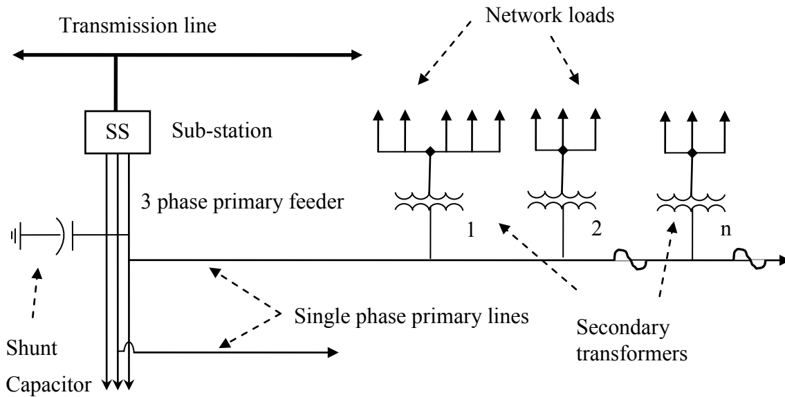
Figure 3.1 Simplified one line diagram of a three phase distribution network
