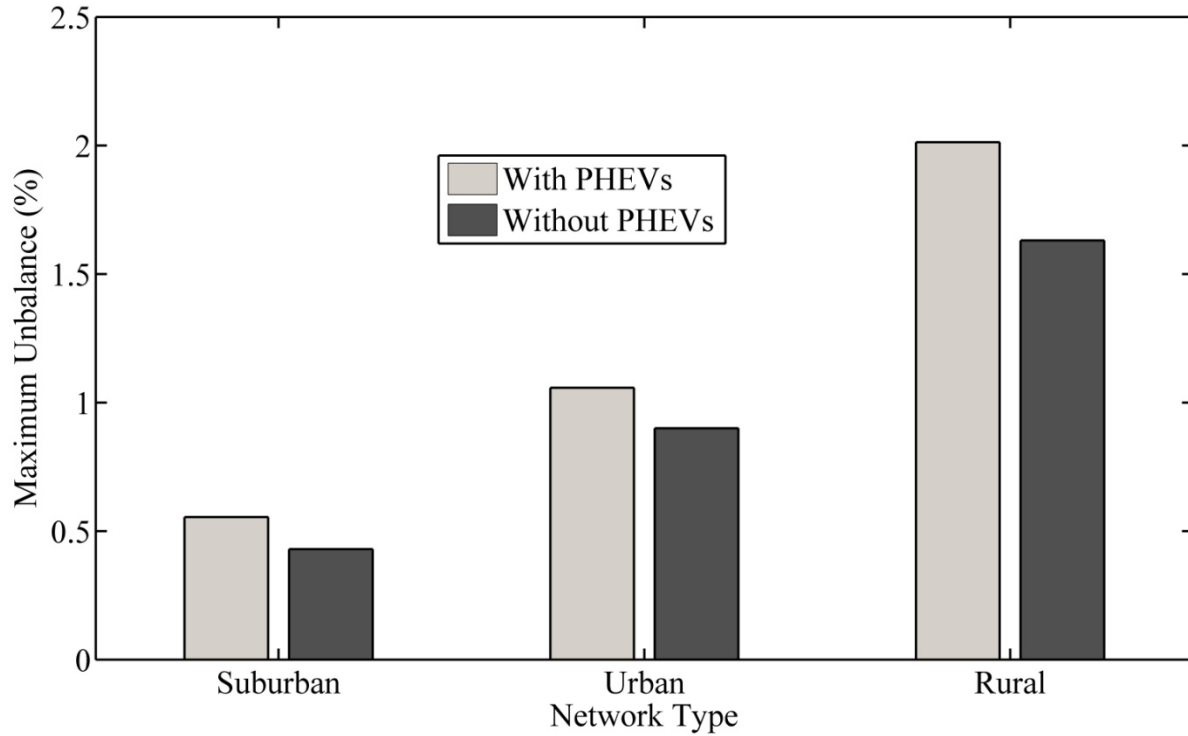
Figure 5.12. Maximum percent voltage unbalance for a three phase bus on each network
