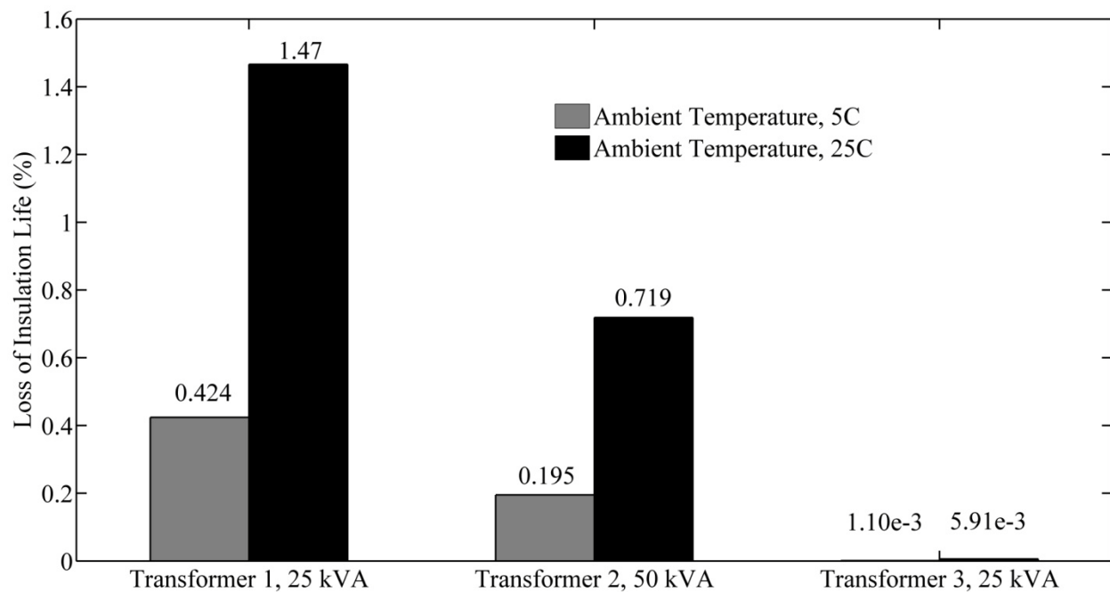
Figure 5.14. Average percent loss of life for one day considering three secondary transformers from the suburban network at 5°C and 25°C ambient temperature. Values are shown above the bars.
