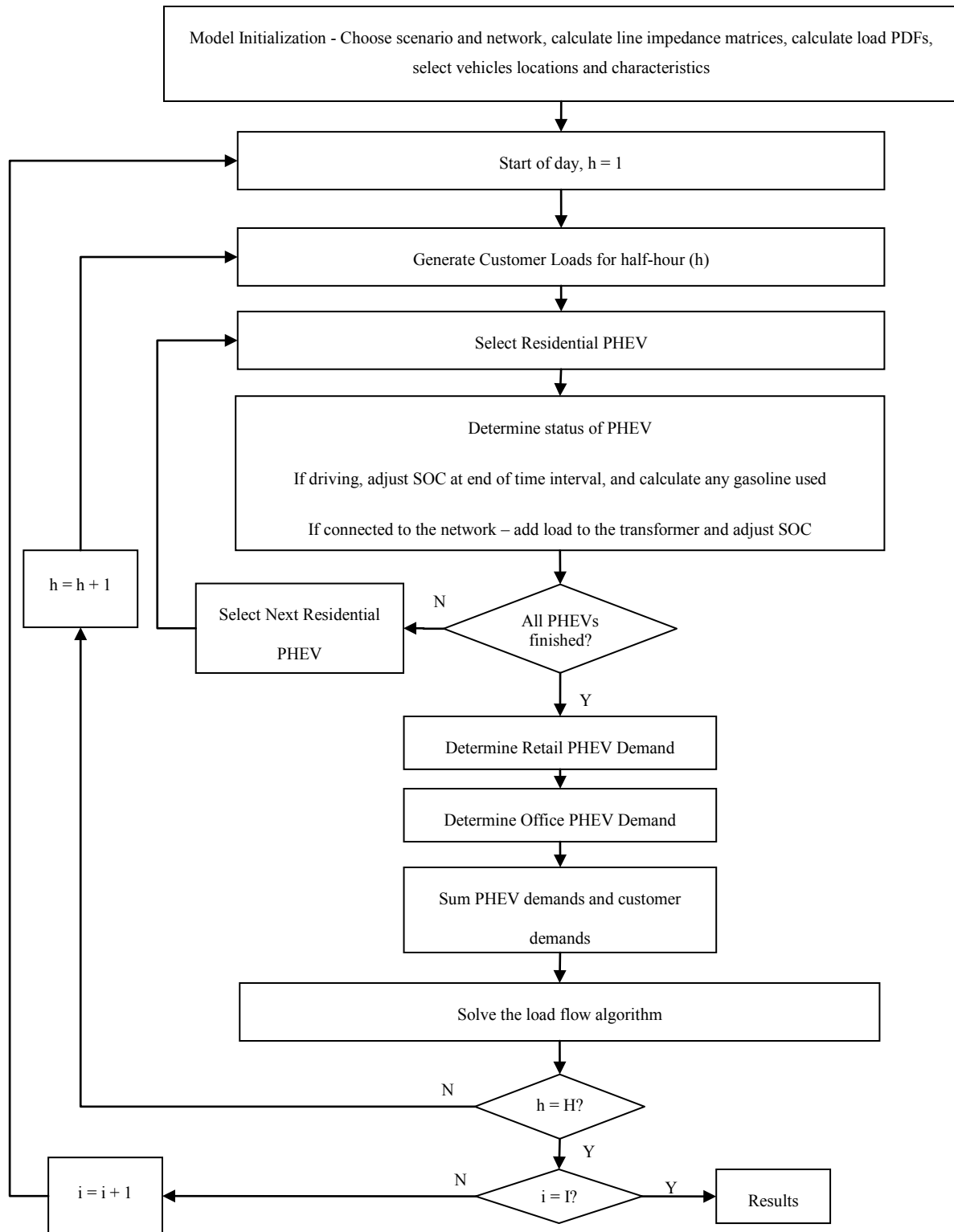
Figure 3.10 Model logic flow chart showing process for determining vehicle charging demand at residential and commercial locations
