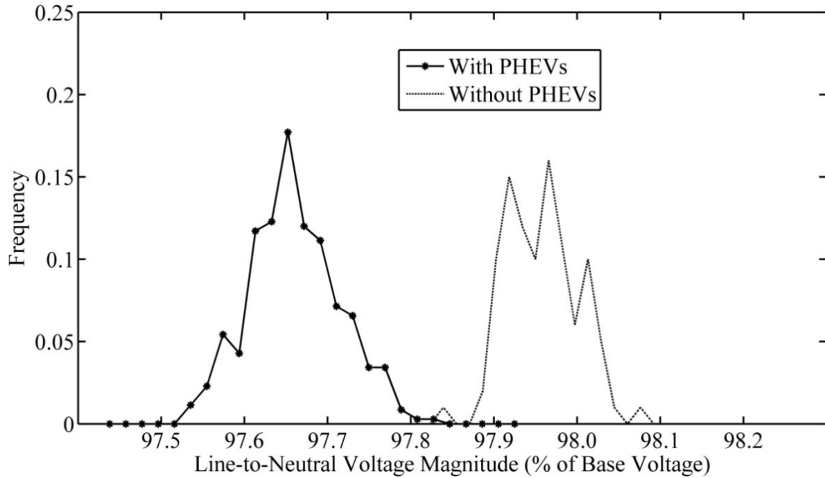
Figure 5.9. Bus voltage distribution for lowest single phase bus voltage on the suburban network at 18:00 hours
