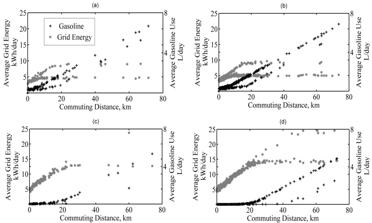
Figure 5.16. Average daily energy and gasoline usage verses commuting distance for combinations of battery sizes and charging rates. (a) 4.85 kWh batteries, 1.44 kW charge rate, (b) 4.85 kWh batteries, 7.6 kW charge rate, (c) 16.6 kWh batteries, 1.44 kW charge rate and (d) 16.6 kWh batteries, 7.6 kW charge rate.
