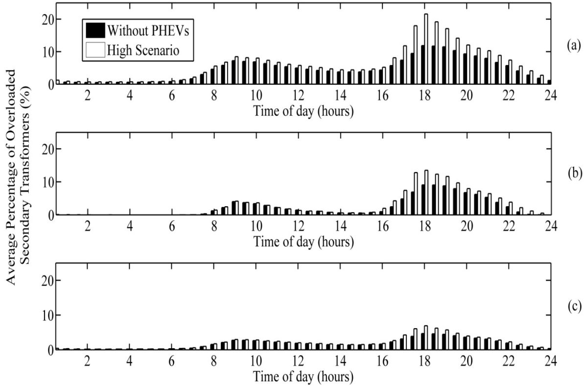
Figure 5.13. Average percentage of overloaded secondary transformers with and without PHEV charging for (a) suburban, (b) urban and (c) rural networks for the high scenario
