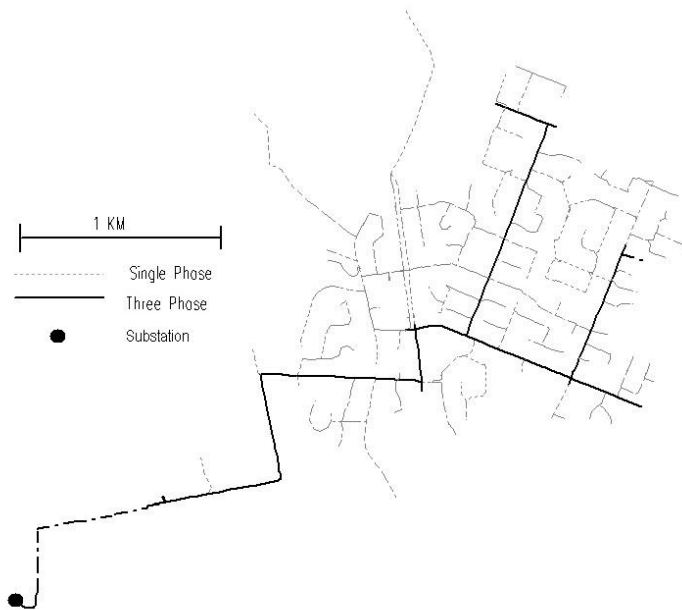
Figure D. 1. Suburban Network (BCHydro code: GTP2546)
