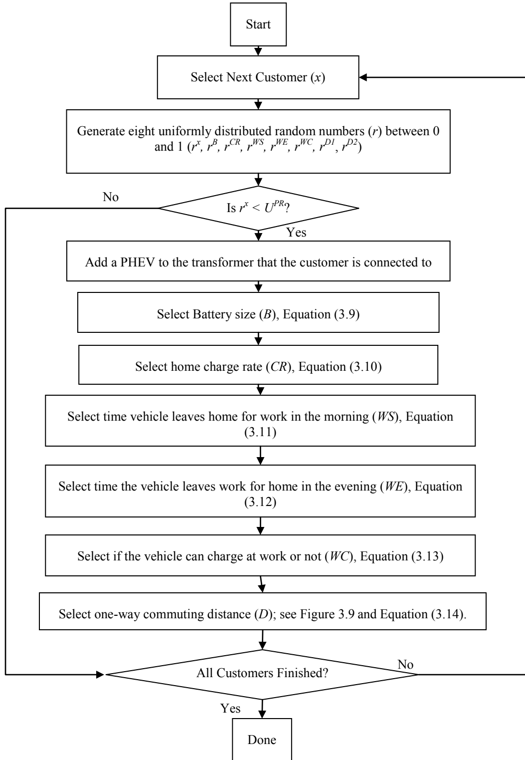
Figure 3.8. Flow chart for probabilistic selection of individual residential vehicle characteristics. U is a probability value. The superscripts are: x – customer number, PR – penetration rate, B – battery size, CR – charge rate, WS – Work start time, WE – work end time, WC – Work Charging, D – commuting distance.
