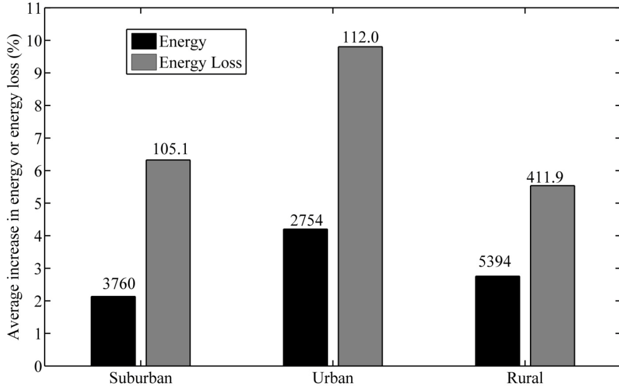
Figure 5.8. Average percent increase in energy and energy loss for the high scenario compared to the base case without PHEV charging. Absolute changes in energy values are shown above each bar in kWh.
