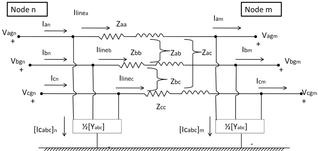
Figure A. 1. Generic Three Phase Line
