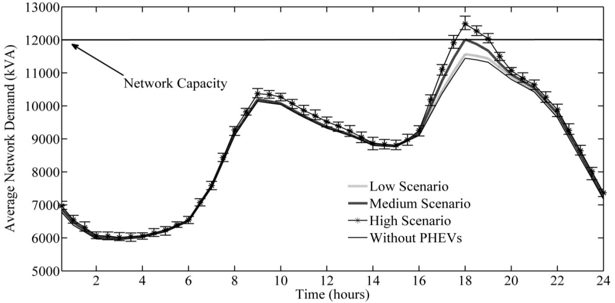
Figure 5.6. Average network demand on the rural network showing exceedance of the network capacity. Error bars show the maximum and minimum values for the high scenario.
