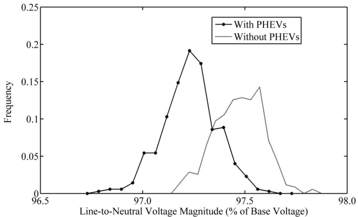
Figure 5.10. Bus voltage distribution for lowest single phase bus voltage on the urban network at 10:00 hours.
