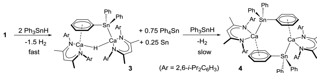
Scheme 2 Synthesis of compounds 3 and 4 and the calcium-centred dismutation of \text{Ph}_3\text{SnH} .
