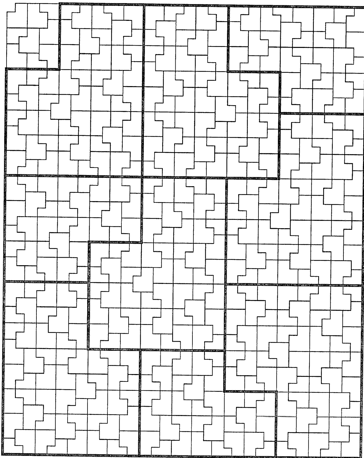
Figure 3: An Ammann Tiling
