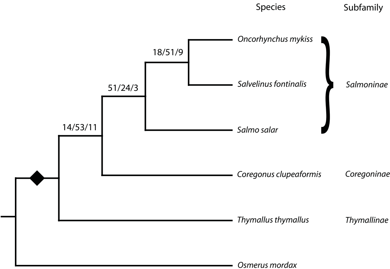
Figure 3 Summary of 78 gene set consensus (70%) trees depicting the relationships among the major groups of Salmonidae. Each branch shows the number of consensus trees supporting the branch, the number of trees providing no information and the number of trees contradicting the branch. The diamond at the base of the Salmonidae cladogram indicates the position where the majority of gene duplications were identified. The individual gene trees that pertain to each branch position are indicated in Table 4.
