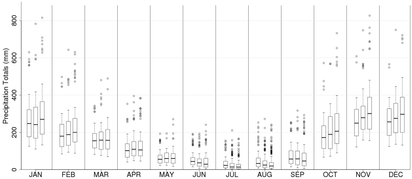
Figure 7: Monthly Total Precipitation – Past, 2050s, and 2080s
