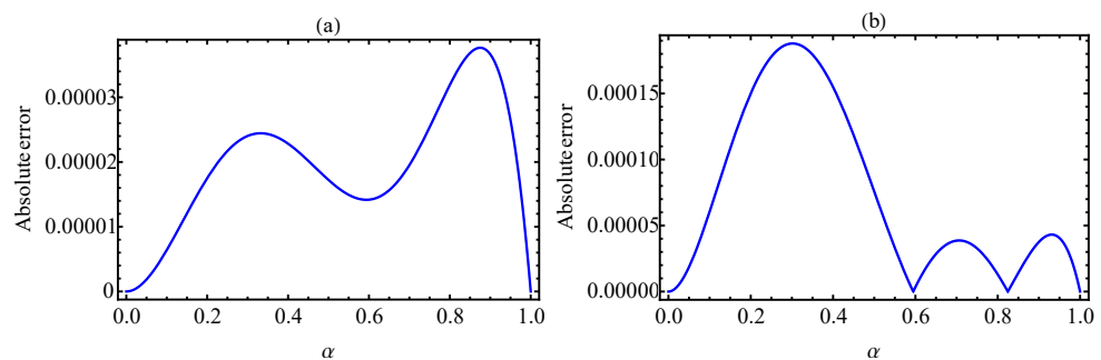
Figure 8. In the case of the ABC-derivative, a graph of the absolute error of (40) in (a) and (41) in (b) for \nu_1 = 2.8, \nu_2 = 0.8, c = 1, \mu_1 = 7, \mu_2 = -6, and a = 1.
