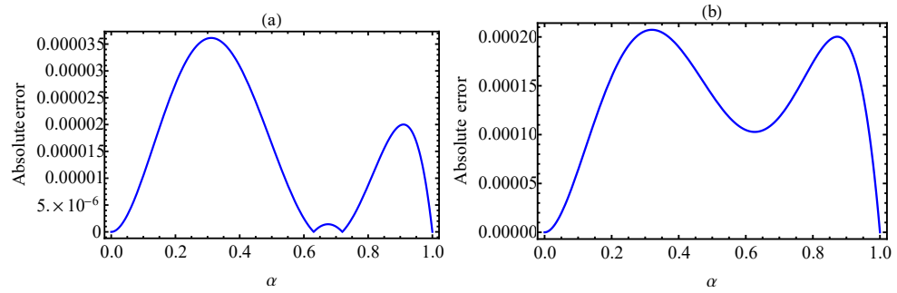
Figure 5. In the case of the CF-derivative, a graph, of the absolute error of (25) in (a) and (26) in (b) for \nu_1 = 2.8, \nu_2 = 0.8, c = 1, \mu_1 = 7, \mu_2 = -6, and a = 1.
