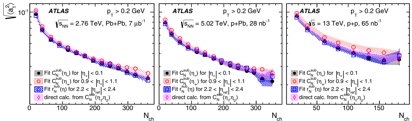
FIG. 13. The \langle a_1^2 \rangle^{1/2} as a function of N_{\text{ch}} from four different methods, fit C_N^{\text{sub}}(\eta_-) (solid circles), fit C_N^{\text{sub}}(\eta_+) (open circles), fit r_N^{\text{sub}}(\eta) (open squares), and Legendre expansion of C_N^{\text{sub}}(\eta_1, \eta_2) (open diamonds), in Pb+Pb (left panel), p + \text{Pb} (middle panel), and pp (right panel) collisions. The error bars and shaded bands represent the statistical and systematic uncertainties, respectively.
