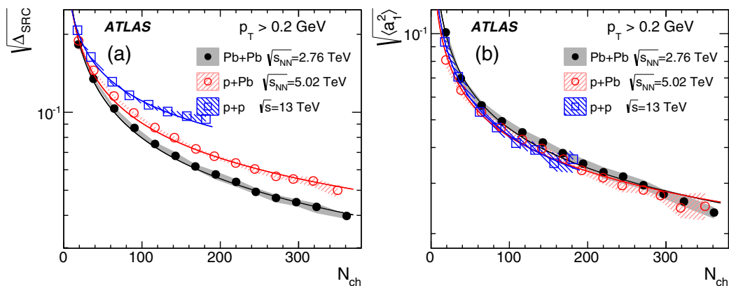
FIG. 15. The estimated magnitude of the short-range component \sqrt{\Delta_{\text{SRC}}} (left panel) and (a_1^2)^{1/2} (right panel) values as a function of N_{\text{ch}} for all-charge pairs in Pb+Pb (solid circles), p + \text{Pb} (open circles), and pp (open squares) collisions. The shaded bands represent the systematic uncertainties, and the statistical uncertainties are smaller than the symbols.
