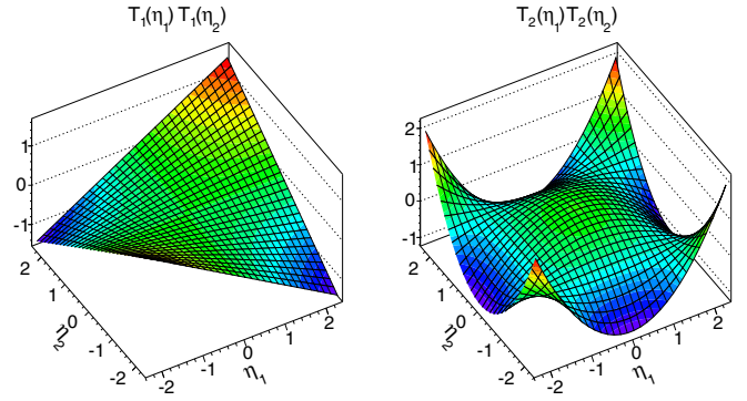
FIG. 7. The first two Legendre basis functions associated with a_{1,1} and a_{2,2} in the two-particle correlation function.
