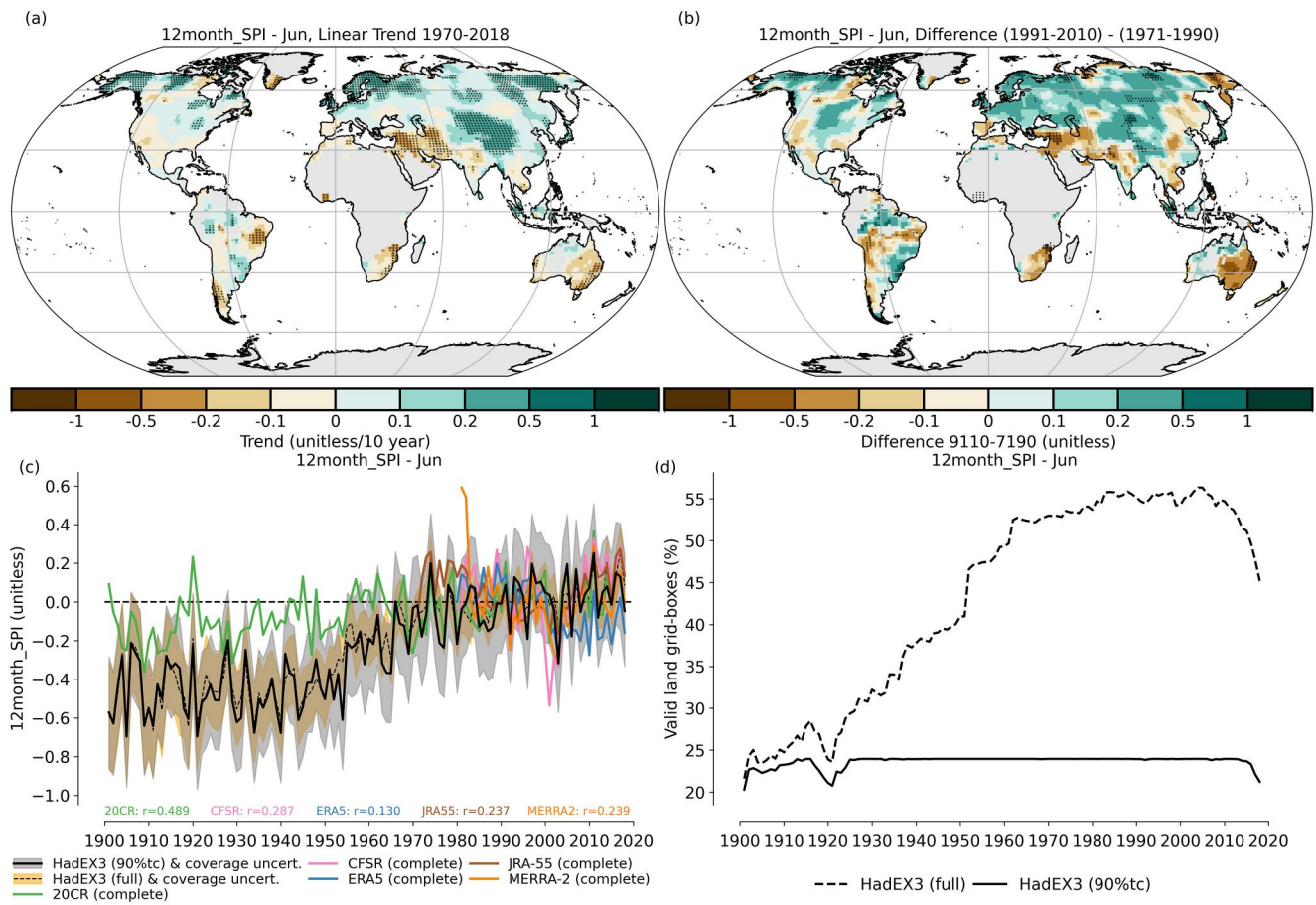
Figure 8. Maps of trends and differences, and time series of the global average anomalies and coverage for annual 12 month-SPI (using 1981–2010 as the reference period). In panel (d) we show the coverage of the full data set as well as from the grid boxes which form the 90% temporally complete (90%tc) subset used for the timeseries in (c). No annual values for SPI are calculated, so we show values for June.
