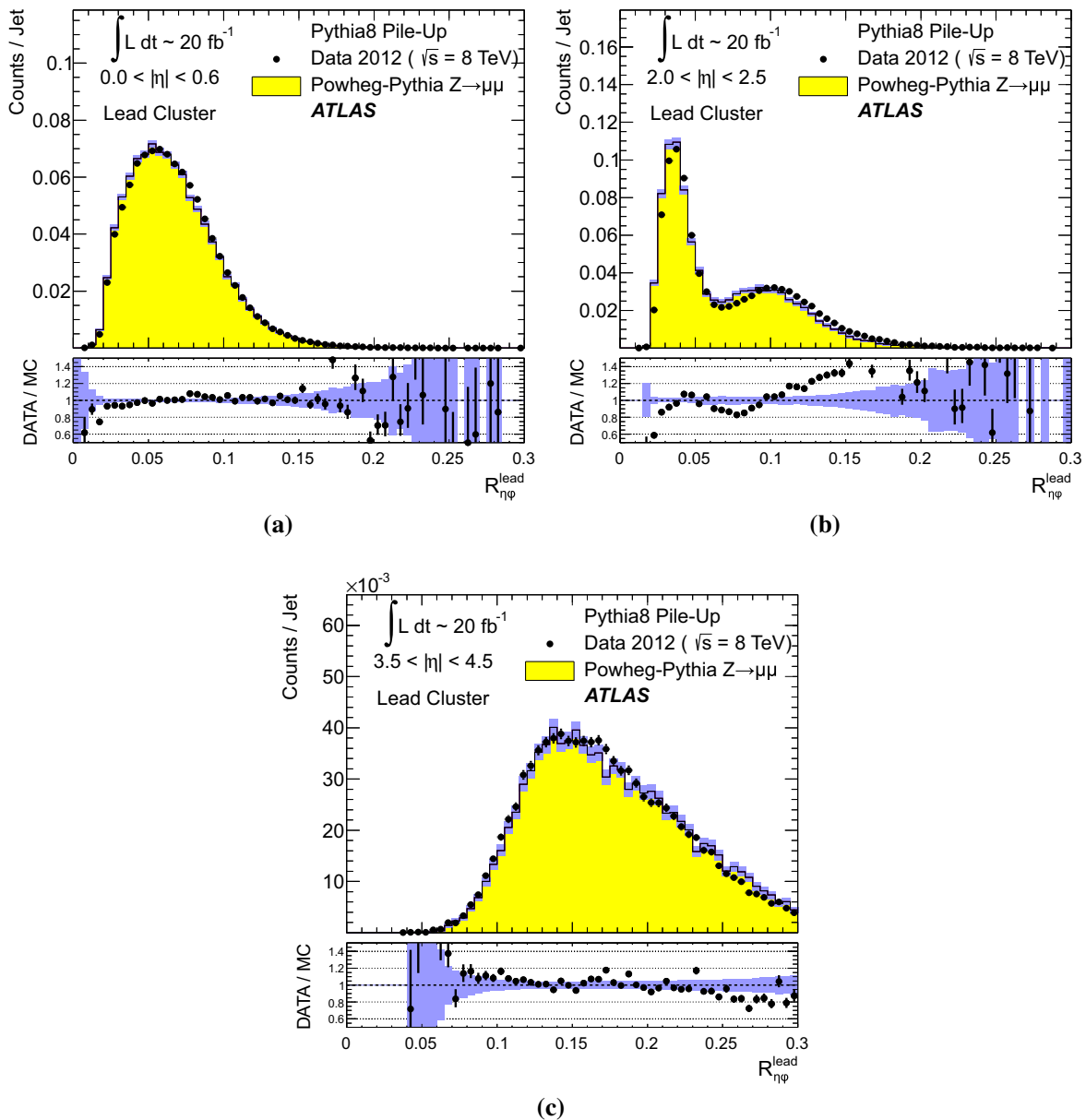
Fig. 43 The size R_{\eta\phi}^{\text{lead}} of the leading topo-cluster in (\eta, \phi) space, measured using Eq. (20), in anti- k_r jets reconstructed with R = 0.4 and with 30 \text{ GeV} < p_{T,\text{jet}}^{\text{LCW+JES}} < 40 \text{ GeV} in Z \rightarrow \mu\mu events in 2012 data and MC simulations with fully simulated pile-up. Distributions are shown for jets in the a central ( |\eta| < 0.6 ), the b end-cap ( 2.0 < |\eta| < 2.5 ), and
