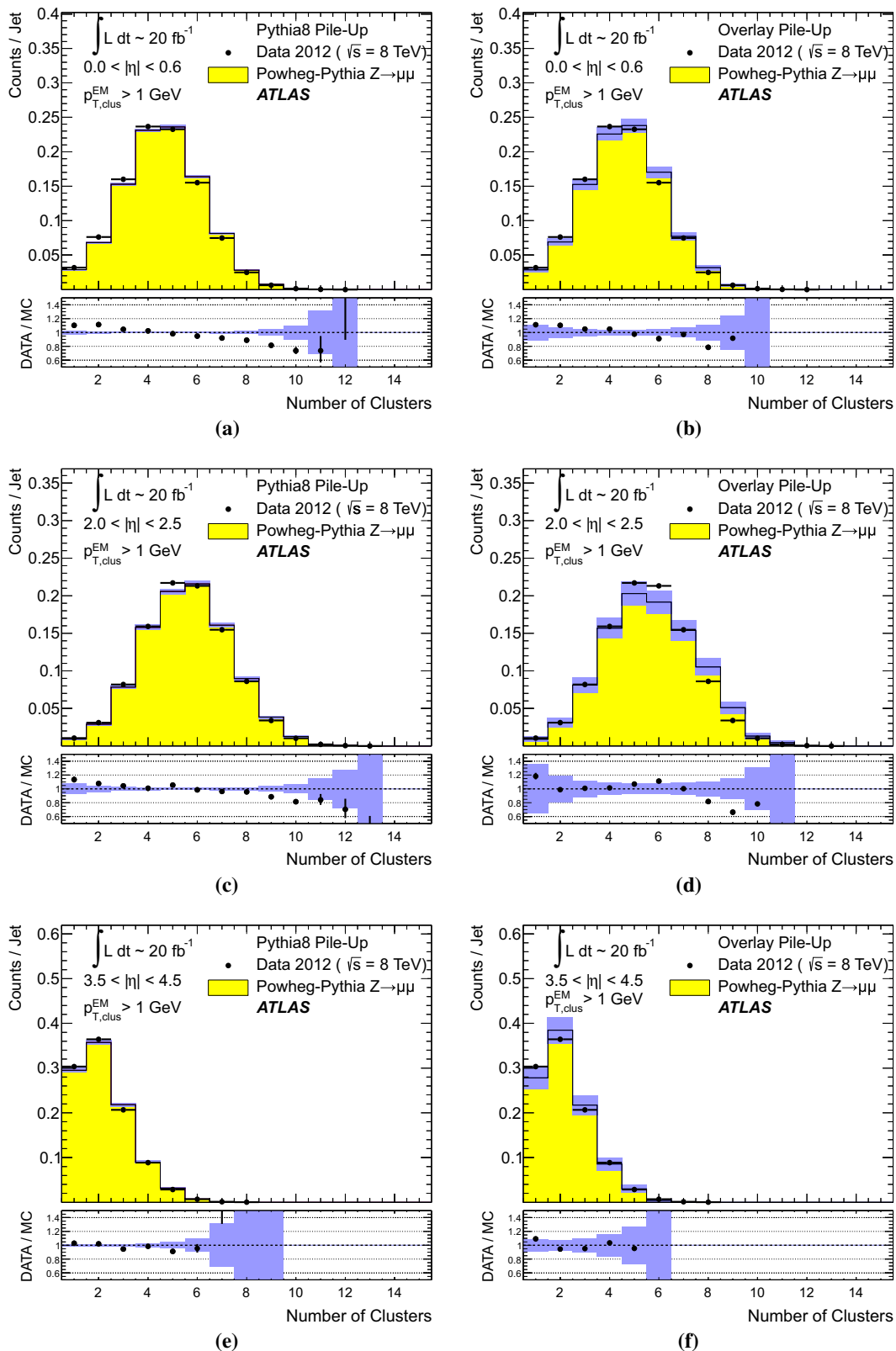
Fig. 32 The distribution of the number of topo-clusters with p_{T,clus}^{EM} > 1 GeV inside anti- k_r jets with R = 0.4 in the (a, b) central ( |\eta| < 0.6 ), the (c, d) end-cap ( 2.0 < |\eta| < 2.5 ), and the (e, f) forward detector region ( 3.5 < |\eta| < 4.5 ) of ATLAS. Shown are results from the analysis of Z \rightarrow \mu\mu events with at least one jet with 30 \text{ GeV} < p_T < 40 \text{ GeV} in 2012 data and MC simulations with fully simulated pile-up in a, c
