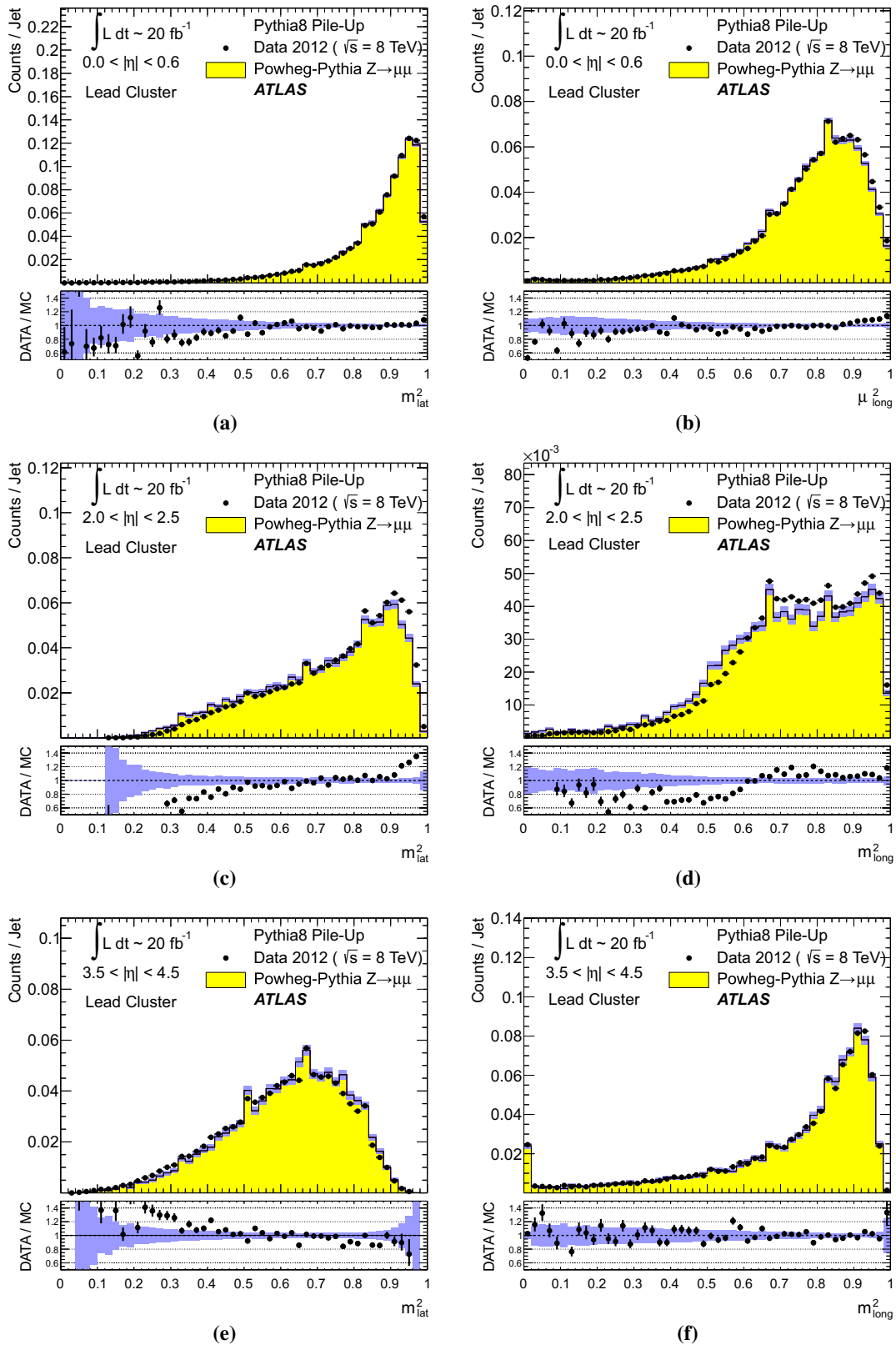
Fig. 41 The distribution of the normalised (a, c, e) lateral ( m_{lat}^2 ) and (b, d, f) longitudinal ( m_{long}^2 ) extension measures of the leading topo-cluster in fully calibrated anti- k_r jets with R = 0.4 and 30 \text{ GeV} < p_{T,jet}^{LCW+JES} < 40 \text{ GeV} in Z \rightarrow \mu\mu events in 2012 data and MC simulations with fully simulated pile-up, for jets in the (a, b) central ( |\eta| < 0.6 ), the (c, d) end-cap ( 2.0 < |\eta| < 2.5 ), and the (e, f)
