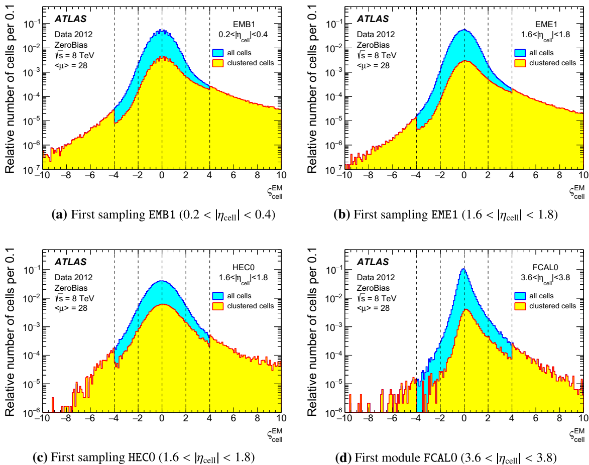
Fig. 5 Signal significance ( z_{\text{cell}}^{\text{EM}} ) distributions for all cells (blue/cyan) and for cells after the noise suppression in the topological cell clustering is applied (red/yellow), in selected sampling layers of the LAr calorimeters: a the first sampling of the central electromagnetic LAr calorimeter (EMB), b the first sampling of the electromagnetic LAr
