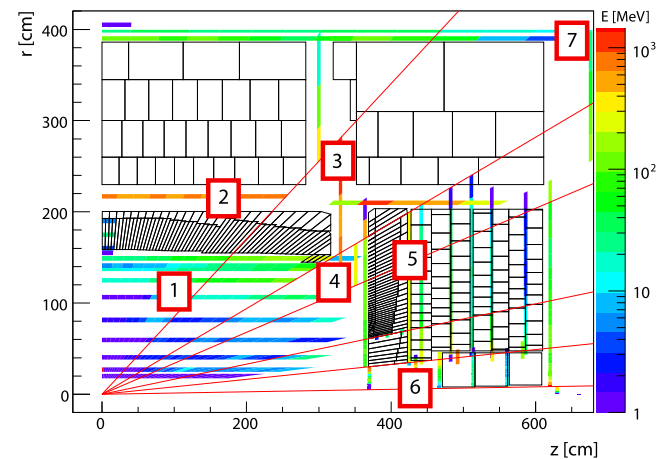
Fig. 17 The average energy loss in the virtual dead material cells for charged 100 GeV pions. The numbers 1–7 indicate the different regions, with region 8 (not displayed) being everywhere outside regions 1–7. The dead material cells are superimposed on a schematic (r, z) view showing a quarter of the ATLAS calorimeter system with its read-out segmentation
