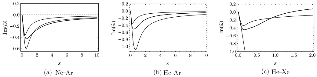
FIG. 2. Dispersion modes in different binary gas mixtures computed with the R17 equations (Eqs. (102)–(105)): (a) Ne–Ar ( x_{\text{Ne}}^{\circ} = 0.5 ), (b) He–Ar ( x_{\text{He}}^{\circ} = 0.5 ), and (c) He–Xe ( x_{\text{He}}^{\circ} = 0.5 ).
