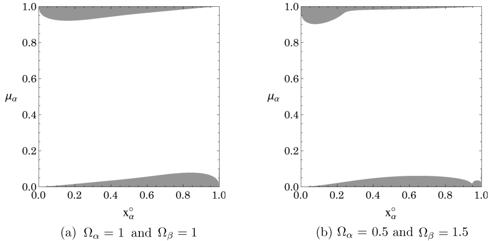
FIG. 3. Zero contours of maximum (dimensionless) damping for different mole fractions ( x_{\alpha}^{\circ} ) and different mass ratios ( \mu_{\alpha} ) with fixed values of \Omega_{\alpha} and \Omega_{\beta} : (a) \Omega_{\alpha} = 1, \Omega_{\beta} = 1 and (b) \Omega_{\alpha} = 0.5, \Omega_{\beta} = 1.5 . The Knudsen number ( \varepsilon ) varies from 0.001 to 5000. The white color represents the regions in which the R17 equations are stable while the gray color portrays the regions in which they are unstable.
