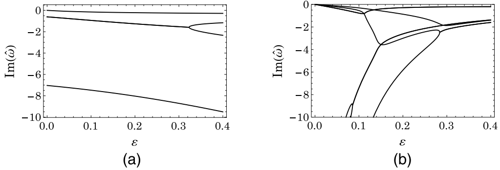
FIG. 1. Dispersion modes in He–Xe mixture with x_{\text{He}}^{\circ} = 0.75 obtained with (a) first order accurate (Fick, Navier–Stokes, and Fourier) equations (Eqs. (62) and (63)), and (b) second order accurate equations (Eqs. (73)–(76)).
