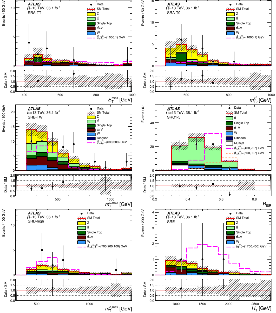
Figure 7. Distributions of E_T^{\text{miss}} for SRA-TT, m_{T2}^2 for SRA-T0, m_T^{b,\text{max}} for SRB-TW, R_{\text{ISR}} for SRC1-5, m_T^{b,\text{max}} for SRD-high and H_T for SRE after the likelihood fit. The stacked histograms show the SM prediction and the hatched uncertainty band around the SM prediction shows the MC statistical and detector-related systematic uncertainties. For each variable, the distribution for a representative signal point is shown.
