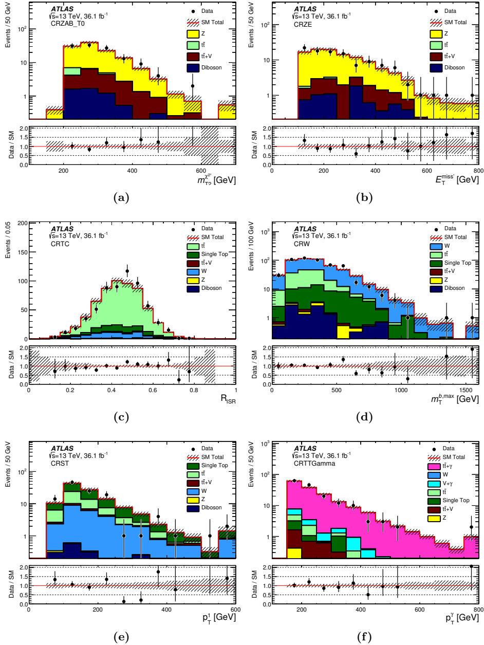
Figure 4. Distributions of (a) m_{T2}^{\chi_{2'}^0} in CRZAB-T0, (b) E_T^{\text{miss}'} in CRZE, (c) R_{\text{ISR}} in CRTC, (d) m_T^{b,\text{max}} in CRW, (e) the transverse momentum of the second-leading- p_T jet in CRST, and (f) the photon p_T in CRTTGamma. The stacked histograms show the SM prediction, normalized using scale factors derived from the simultaneous fit to all backgrounds. The “Data/SM” plots show the ratio of data events to the total SM prediction. The hatched uncertainty band around the SM prediction and in the ratio plot illustrates the combination of MC statistical and detector-related systematic uncertainties. The rightmost bin includes overflow events.
