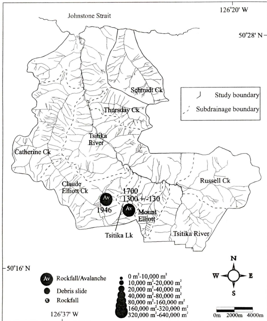
Figure 5.24: Landslides that may have been coincident to seismic events. Landslides based on minimum ages. Dates of seismic activity are beside landslide.
