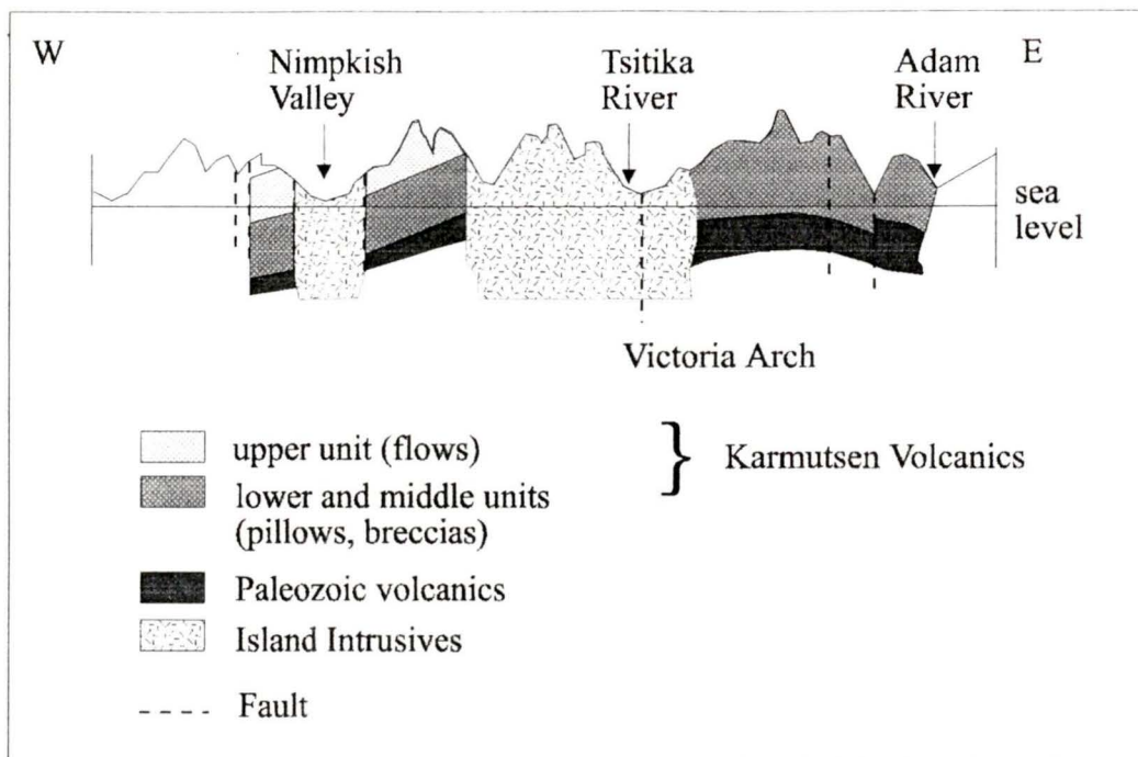
Figure 2.5: The culmination of the Victoria Arch which makes up the backbone of Vancouver Island. The layered units of the Karmutsen formation dip away from the arch on both sides. This results in a westward trending dip in the study area.
