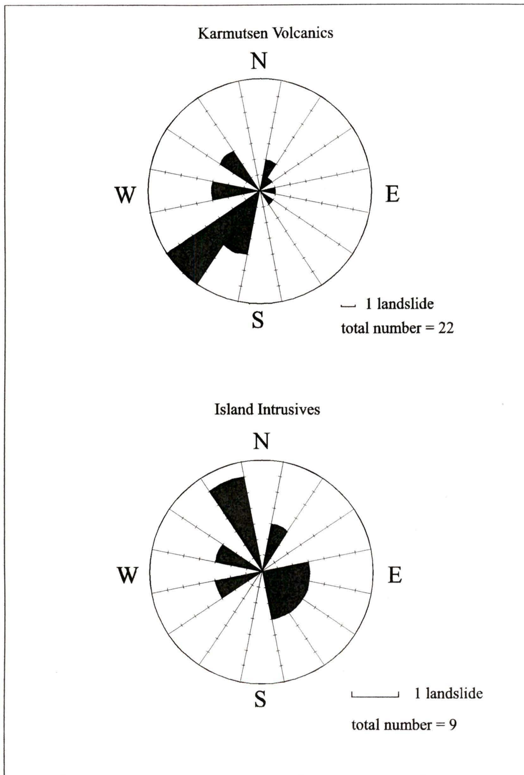
Figure 5.5: Azimuth direction of landslides in the study area compared to geology.
