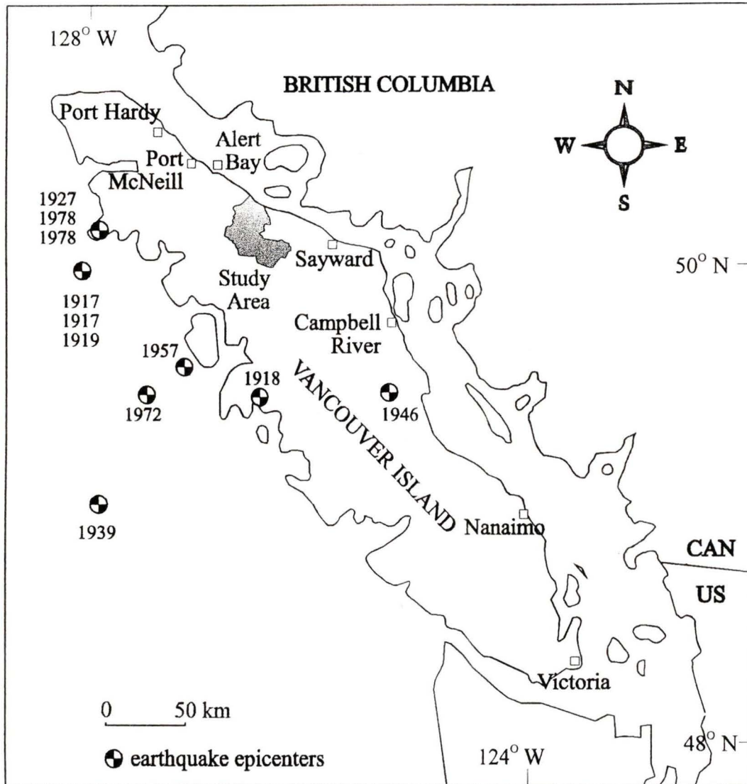
Figure 5.17: Location map of seismic events which resulted in accelerations equal to or greater than 10 \text{ cm/s}^2 in the study area (unpublished data from Horner and Weichert at the Pacific Geoscience Center, Sidney, B. C.).
