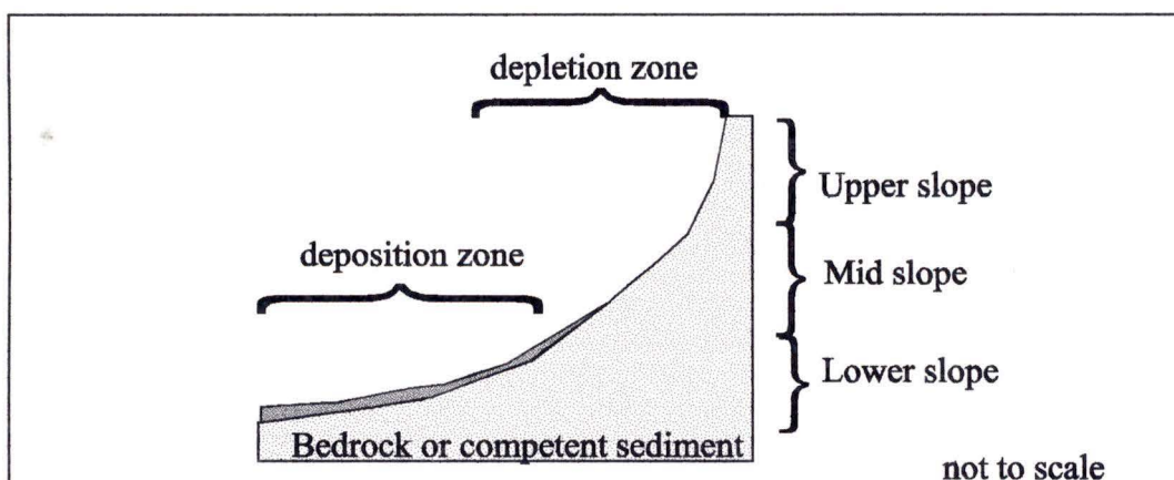
Figure 4.4: A typical profile of a debris slide.
