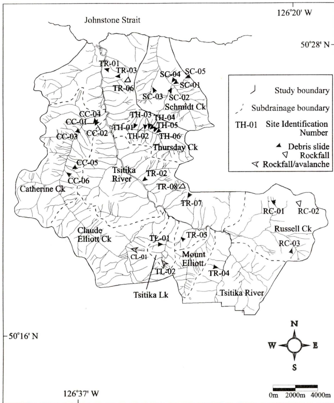
Figure 5.1: Landslide sites and identification numbers in the study area.
