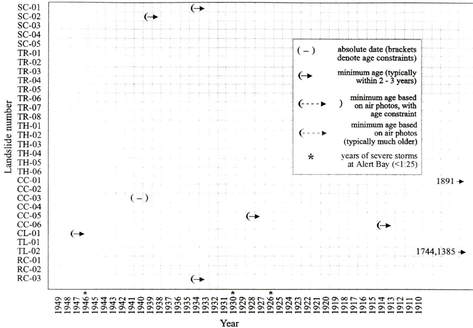
Figure 5.20: Dates of landslides in the Tsitika study area (continued from previous page).
