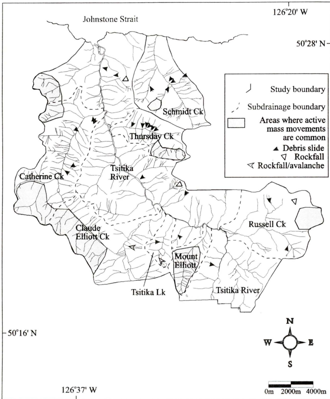
Figure 5.2: The generalized concentration of active mass movements (snow avalanching, and active rockfall) in the study area in relation to discrete events.
