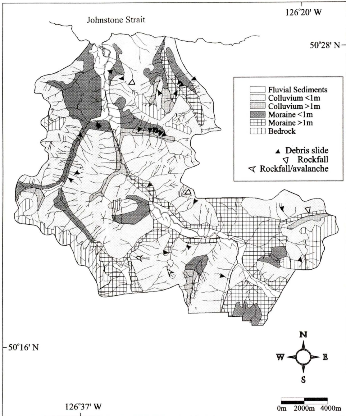
Figure 5.4: The distribution of landslides relative to surficial geology.
