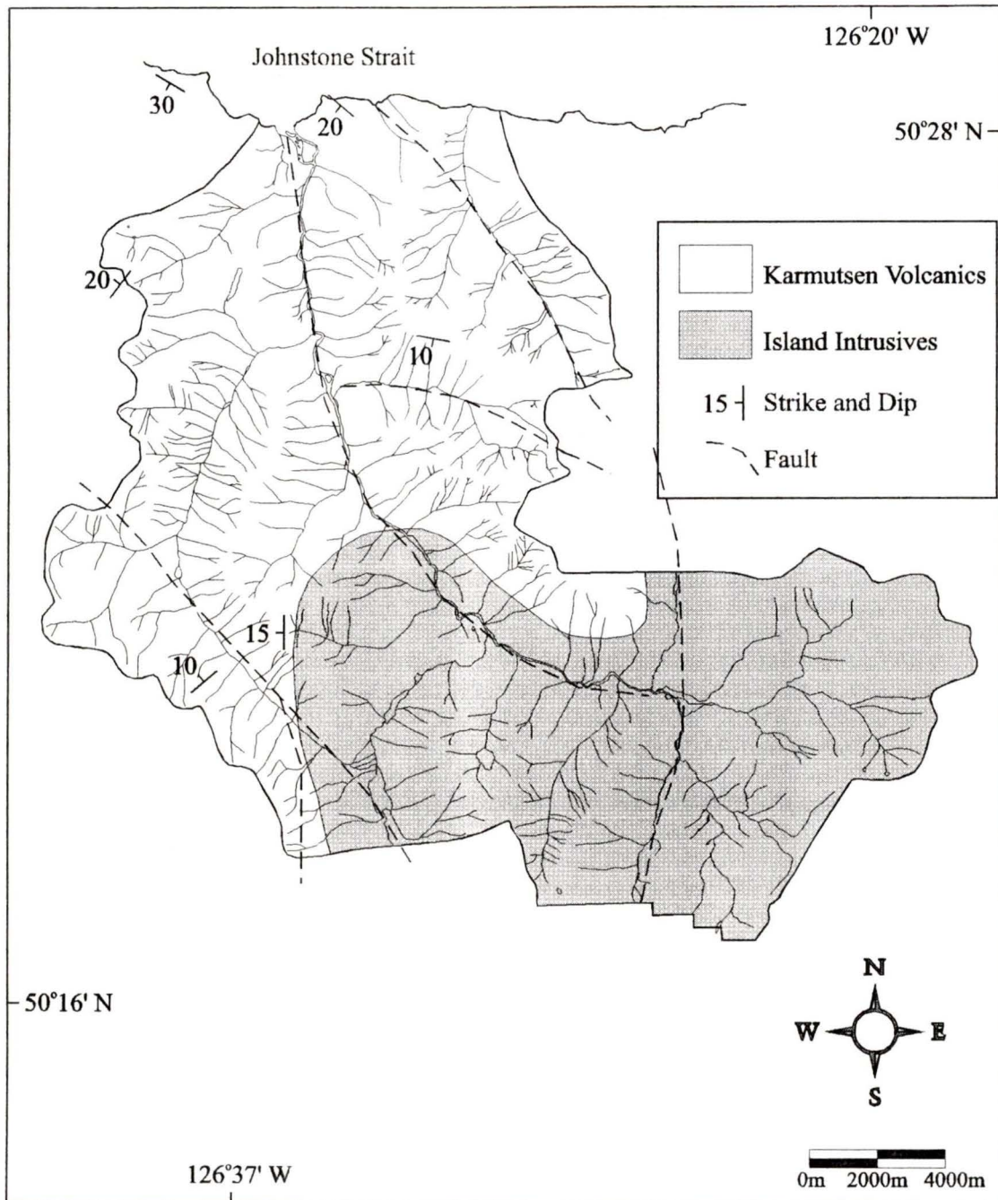
Figure 2.4: The bedrock geology of the Tsitika study area (Muller and Roddick, 1983).
