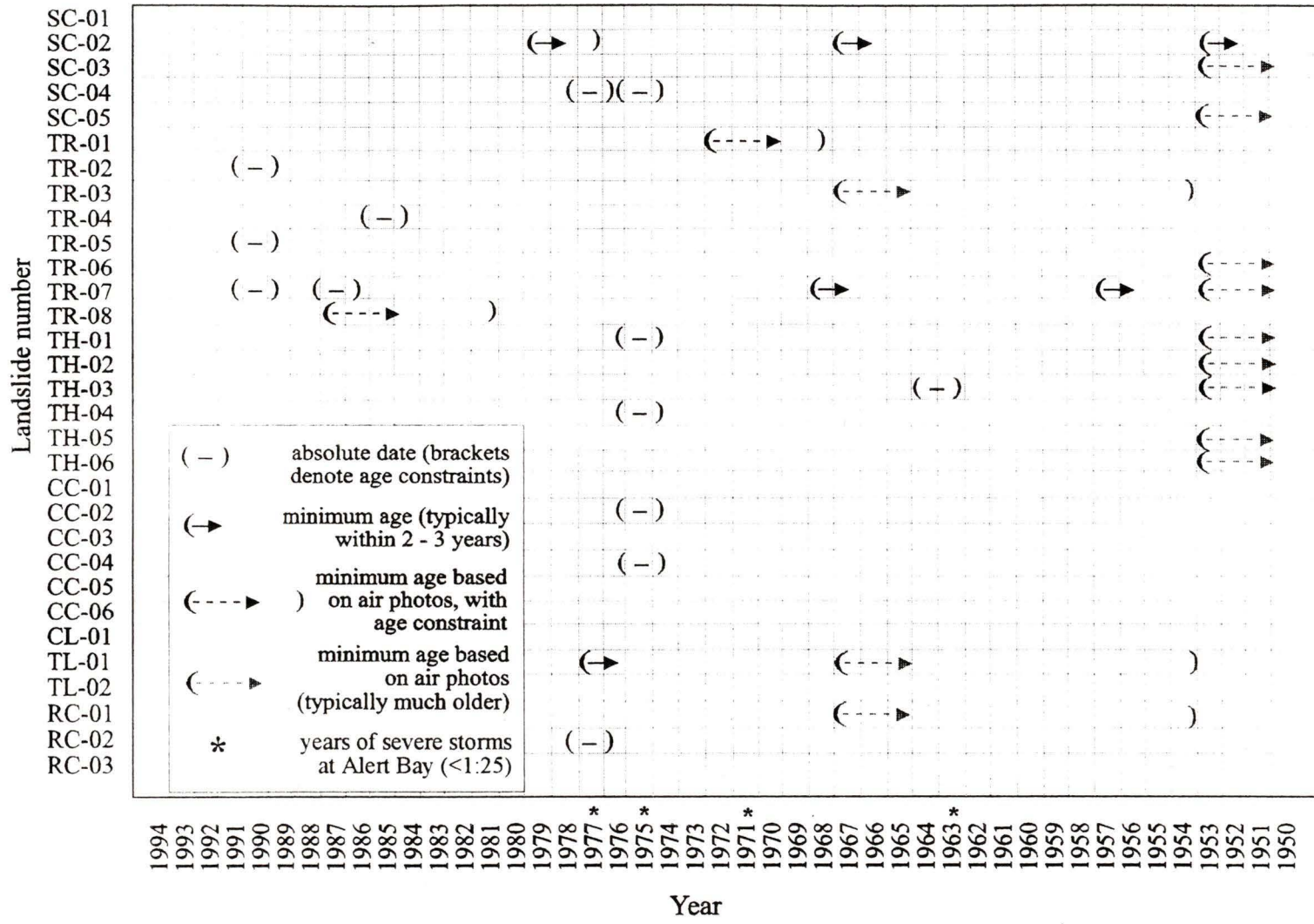
Figure 5.20: Dates of landslides in the Tsitika study area (continued next page).
