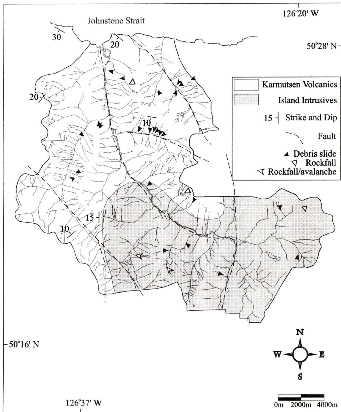
Figure 5.3: The distribution of landslides relative to bedrock geology.
