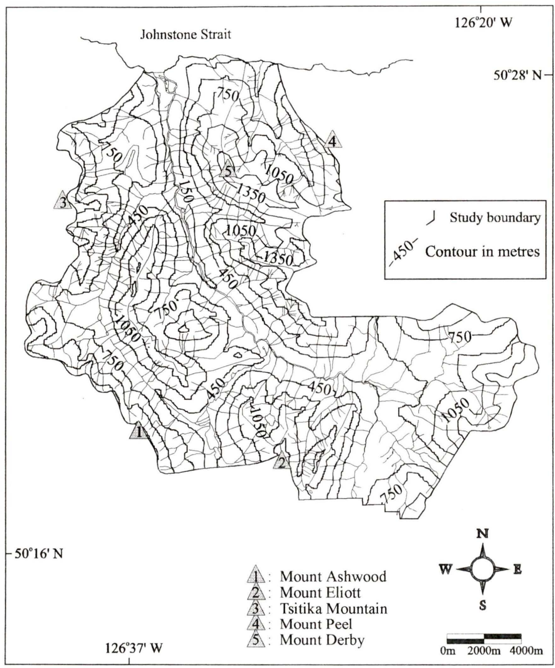
Figure 2.3: A topographic map, showing mountain peaks in and adjacent to the study area.
