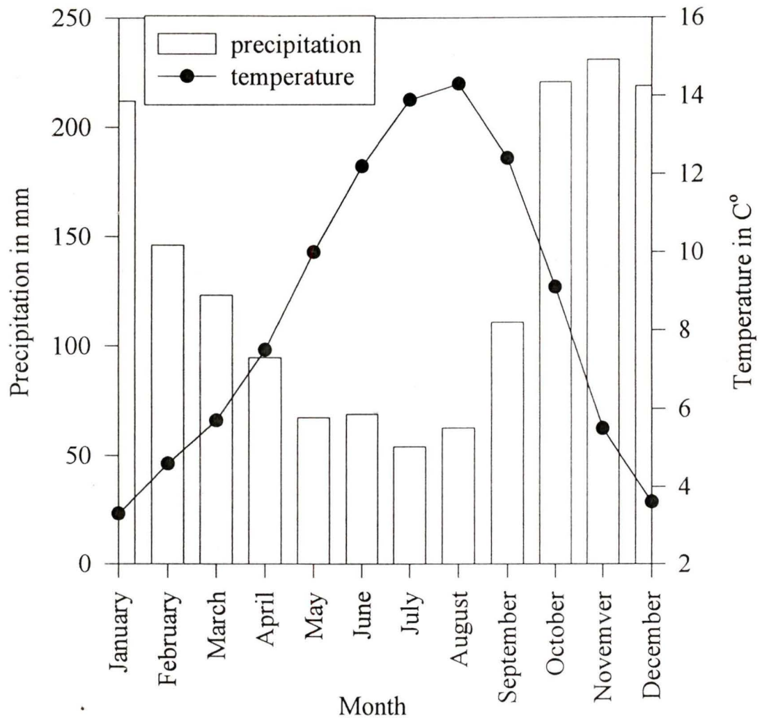
Figure 2.8: Mean monthly precipitation and temperature at Alert Bay, 1913-1990 (Environment Canada, 1993).
