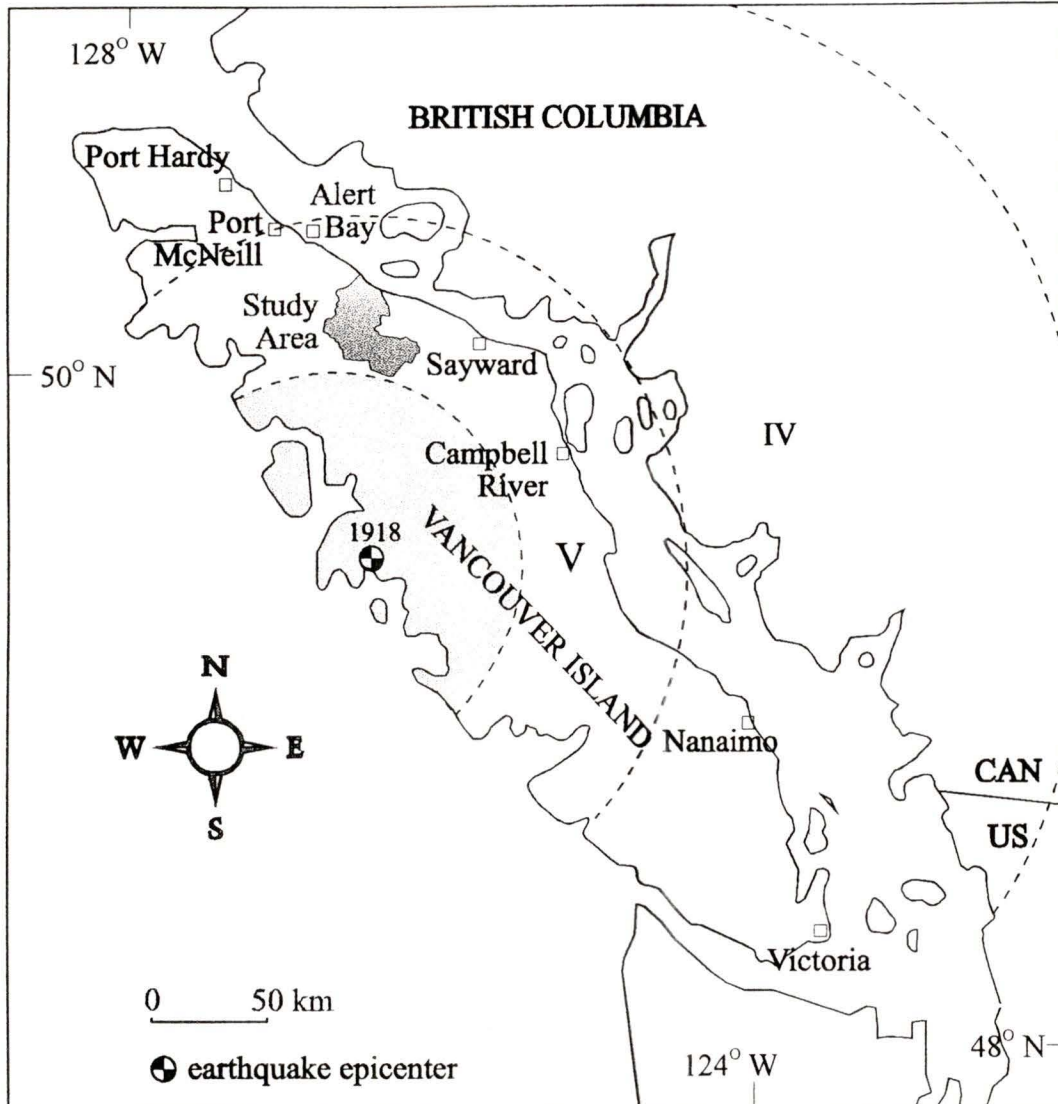
Figure 5.18: Isoseismal map of 1918 earthquake. Roman numerals represent modified Mercalli intensities. Shaded circle experienced intensities of VI and greater (from Cassidy et al. , 1988).
