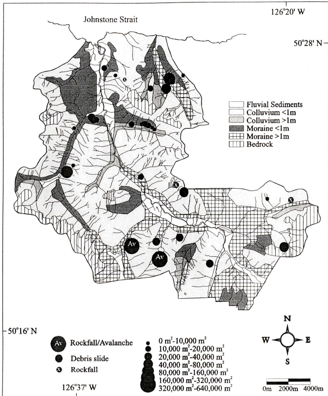
Figure 5.11: Landslide areas compared to surficial geology.
