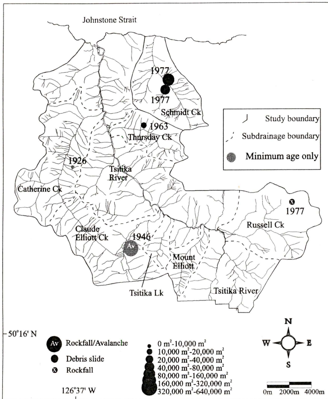
Figure 5.23: Landslides that may have been coincident to storms with return intervals from 1:25 - 1:50 years. Date of storm is beside landslide.
