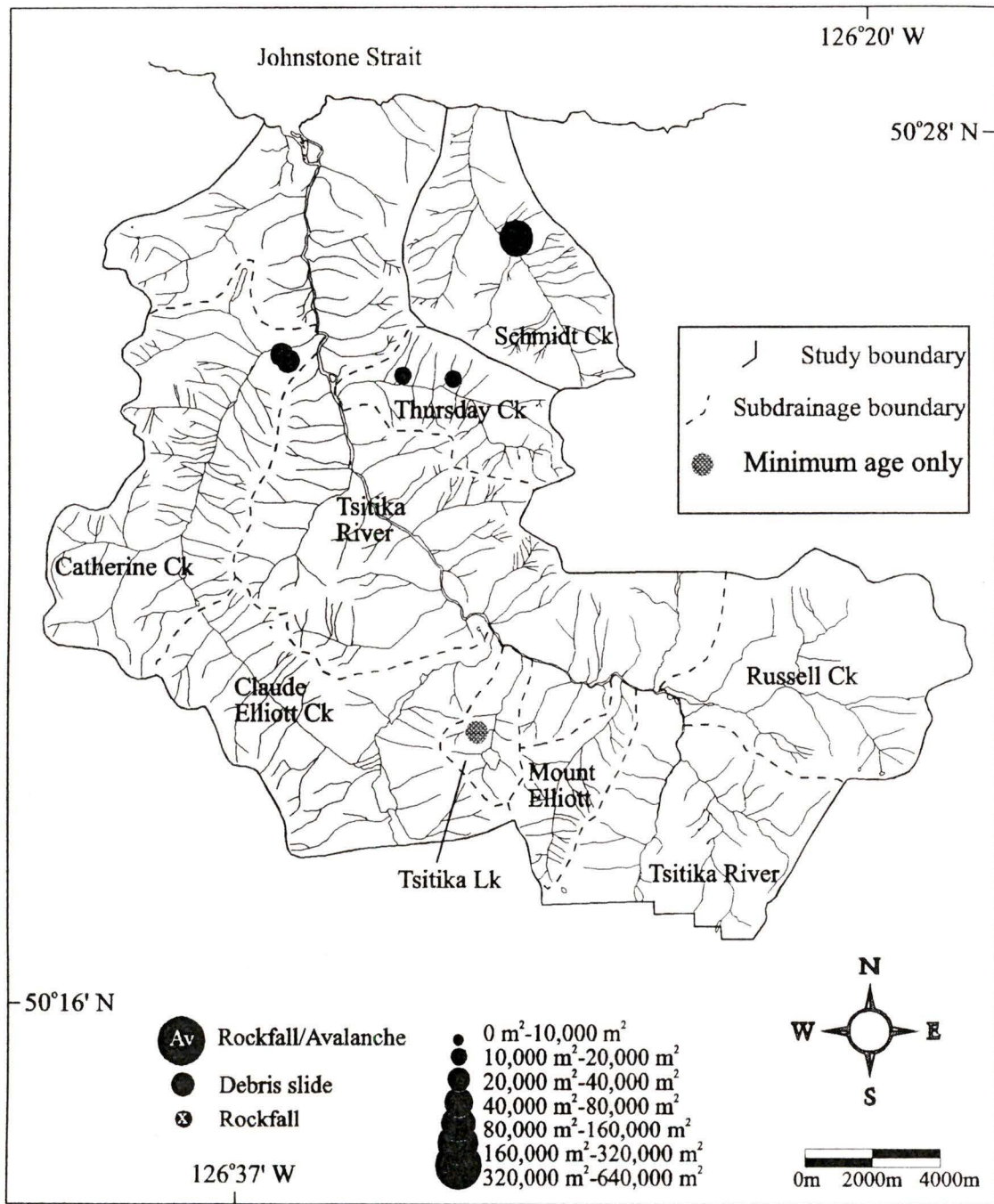
Figure 5.22: Landslides that may have been coincident to the 1975 storm (return interval < 1:50 years).
