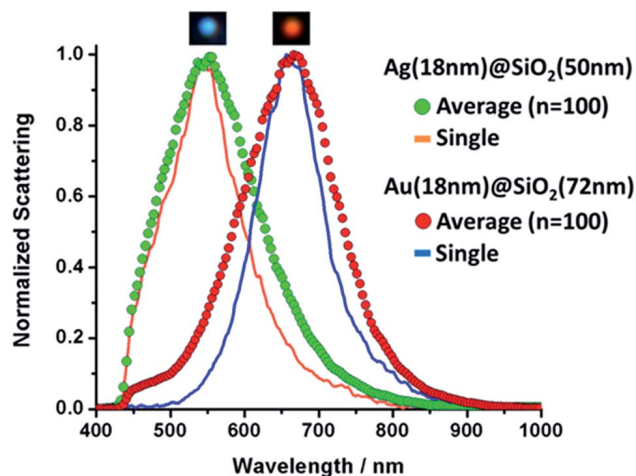
Fig. 3 Single and averaged ( n = 100 ) scattering spectra for Ag and Au nanoshells. Insets above each curve show individual nanoshells as seen under dark field illumination.
