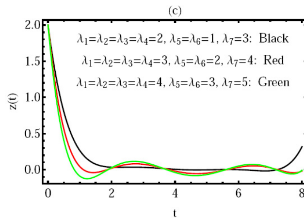
Figure 3. Behavior of the approximate solution via different values of the parameters \lambda_j ( j = 1, \dots, 7 ).
