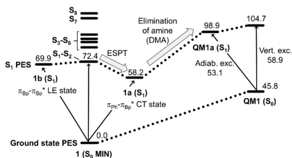
Figure 2. Energy diagram for the QM formation from 1 . Stationary points for the ground and the S_1 state were computed at the PBE0/6-311G(2d,p) level of theory. Relative energies are given in kcal mol -1 . Optimized structures ( S_0 and S_1 ) are shown in the SI.
