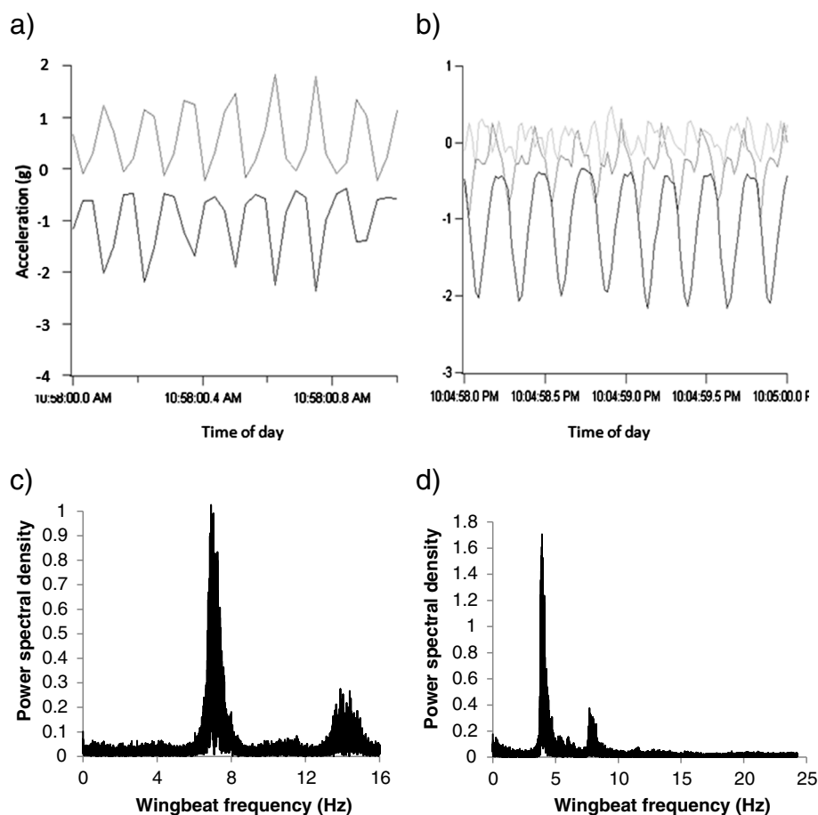
Figure 3 Representative acceleration traces (longitudinal axis, used to calculate Fourier transforms, in bold) of flying (a) murre and (b) kittiwake. Fourier spectra from the same flights in (c) murre and (d) kittiwake.
