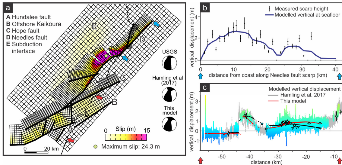
Fig. 6. (a) Best fitting slip model for the Kaikōura earthquake based on inversion of geodetic and coastal deformation data (see section 3.3 for details). Moment tensors show the USGS CMT solution and the equivalent for the Hamling et al. (2017) model and the model produced for this study. Heavy black lines denote the top edge of the fault surface. Note the Papatea fault is not included in this model, see Hamling et al. (2017) for discussion. (b) Fit between the modeled vertical displacement and vertical displacement along the 2016 rupture scarp of the Needles fault. (c) Fit between the modeled vertical displacement and compiled vertical displacement measurements (see key in Fig. 4) from the Conway River to north of Kaikōura Peninsula. This plot demonstrates improved fit using the refined dislocation model of this study compared to the model of Hamling et al. (2017) which omitted a crustal fault offshore of Kaikōura Peninsula.
