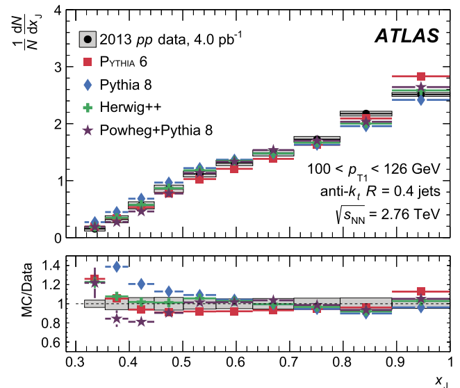
Fig. 7. The (1/N)dN/dx_j distribution for R = 0.4 jets in pp collisions for the 100 < p_{T_1} < 126 GeV interval is shown in black points with the grey shaded boxes indicating the systematic uncertainties. Also shown are results obtained from various MC event generators: PYTHIA 6 (red squares), Pythia 8 (blue diamonds), Herwig++ (green crosses) and Powheg+Pythia 8 (purple stars). The ratio of each MC result to the data is shown in the bottom panel where the systematic uncertainties of the data are indicated by a shaded band centred at unity. (For interpretation of the references to colour in this figure, the reader is referred to the web version of this article.)
