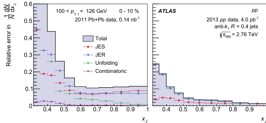
Fig. 6. The total systematic uncertainty and its various components for 100 < p_{T_1} < 126 GeV for R = 0.4 jets in Pb+Pb collisions with 0–10% centrality (left) and pp collisions (right). In the figure on the left the first two bins are off scale with bins centres of x_j = 0.34 and 0.38 and bins contents of 1.25 and 0.75, respectively.
