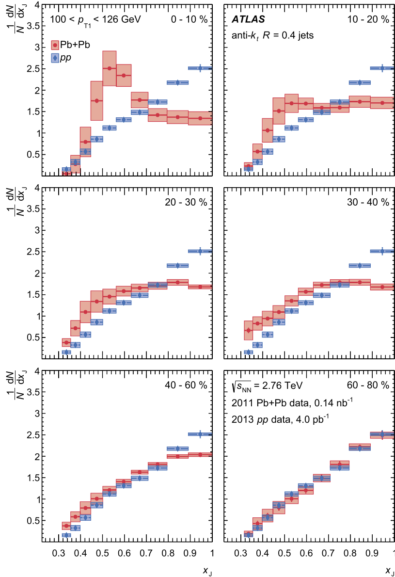
Fig. 8. The (1/N)dN/dx_j distributions for jet pairs with 100 < p_{T_1} < 126 GeV for different collision centralities for R = 0.4 jets. The Pb+Pb data are shown in red circles, while the pp distribution is shown for comparison in blue diamonds, and is the same in all panels. Statistical uncertainties are indicated by the error bars while systematic uncertainties are shown with shaded boxes. (For interpretation of the references to colour in this figure, the reader is referred to the web version of this article.)
