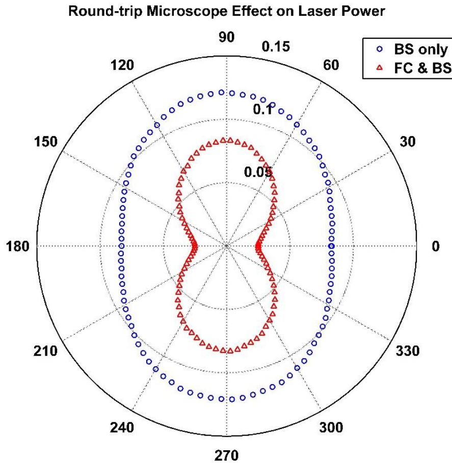
Figure 4.11 Microscope output laser power depending on a full 360^\circ range of laser polarization angles in round-trip path. Round-trip microscope effect shows a significant output power difference between perpendicular and parallel (to table surface) input laser polarizations.
