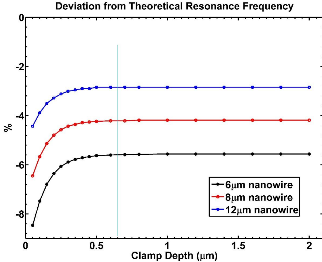
Figure 2.3 Plot showing percentage of deviation predicted by clamp model simulation, with respect to theoretical results. For the same nanowire length, for shorter clamped depths, there is a larger deviation from the theoretical resonance frequency. Beyond a threshold value of clamp depth the deviation will reach a plateau. The figure shows the plateau resonance frequencies of 12 μm nanowire is closest to the theoretical calculation, while the stiffer 6 μm nanowire plateau shows the largest gap from the theoretical value.
