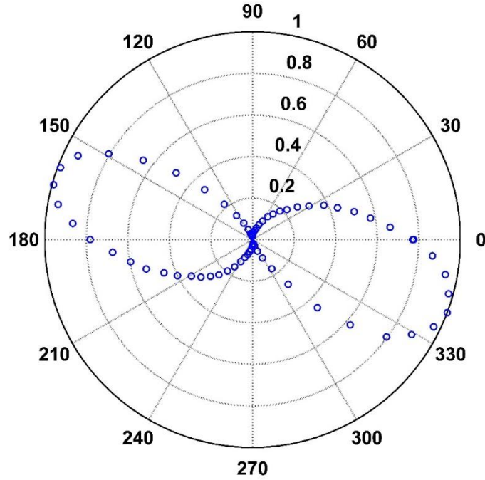
Figure 4.12 Polar plot of polarization effect factor \alpha of SiNW after correction with round-trip microscope effect (FC and BS installed) in a full range of orientation angles. Minimum \alpha is obtained at 90 °and 270 °orientation angles (laser polarized perpendicular to the nanowire axis) which makes the resonance peak amplitude only 3% of the maximum.
