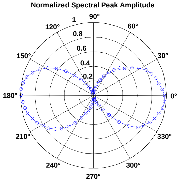
Figure 4.5 Polar plot of normalized spectral peak amplitude in an orientation angle of 360 degree. The maximum peak amplitude is attained at orientation angle of 0° and 180° in which the laser polarization is parallel to the SiNW axis. A considerable loss of 96% of signal amplitude is detected as polarization state is set perpendicular to SiNW axis (90° and 270° in the figure).
