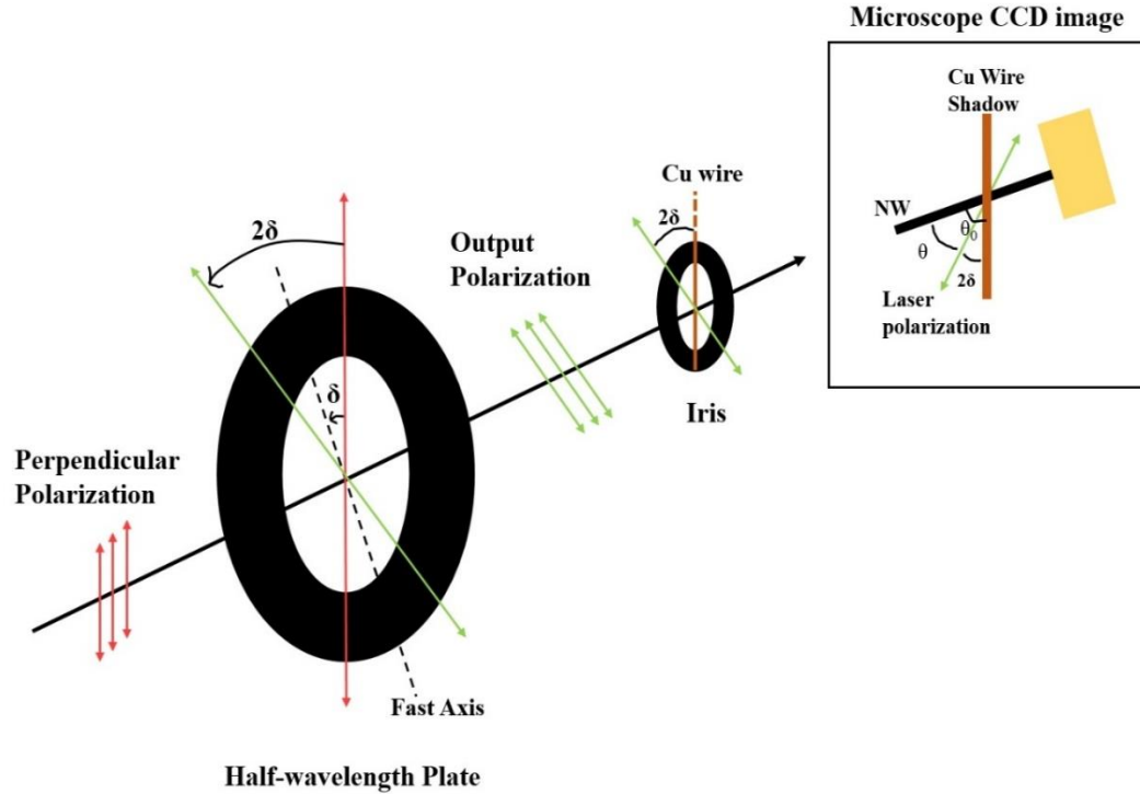
Figure 4.2 Sketch of optical components alignment for laser polarization effect experiment.
