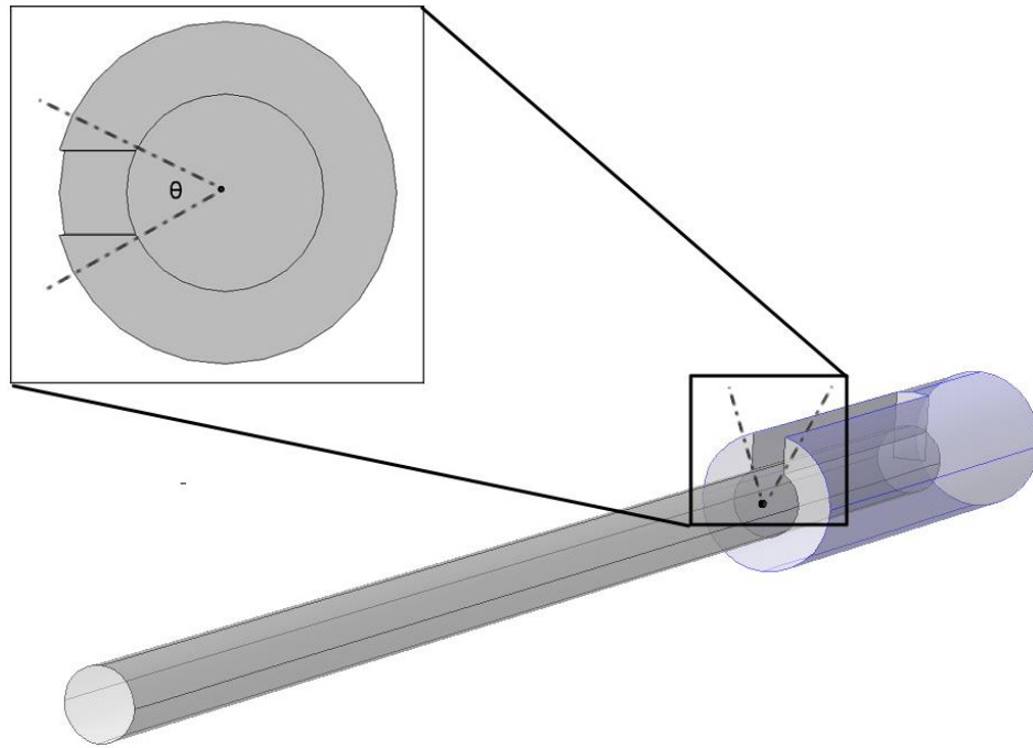
Figure 2.8 Cylinder tube clamp model designed to demonstrate the effect of defect area on resonance frequency. Constraint conditions are applied to the outer surface of cylinder clamp. The inset illustrates the definition of a size of clamp defect, which is represented by an angle of opening window.
