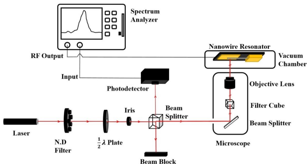
Figure 3.1 Schematic diagram of optical transduction setup
