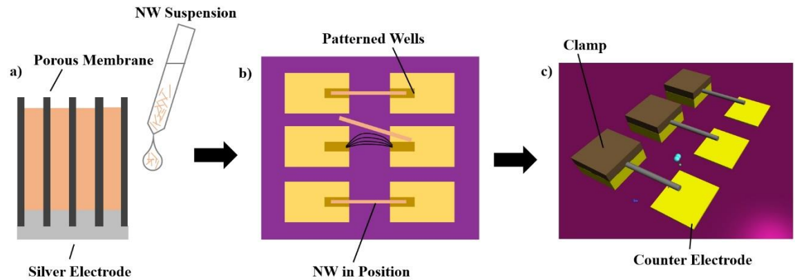
Figure 3.4 Illustrations of nanowire resonator fabrication process. a) Electrodeposition of RhNWs using nanoporous membrane with silver electrode deposited at the bottom. b) RhNW guided by the dielectrophoresis force to patterned wells. c) 3D illustration of clamped nanowire resonator arrays.
