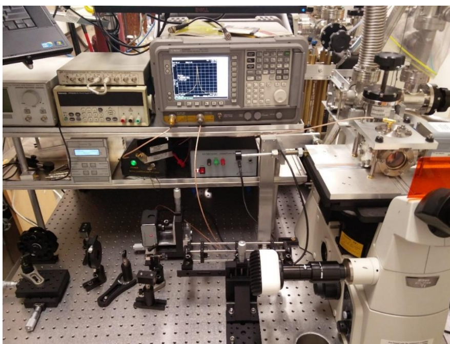
Figure 3.2 Photo of real optical components and electronic devices used in optical transduction.
