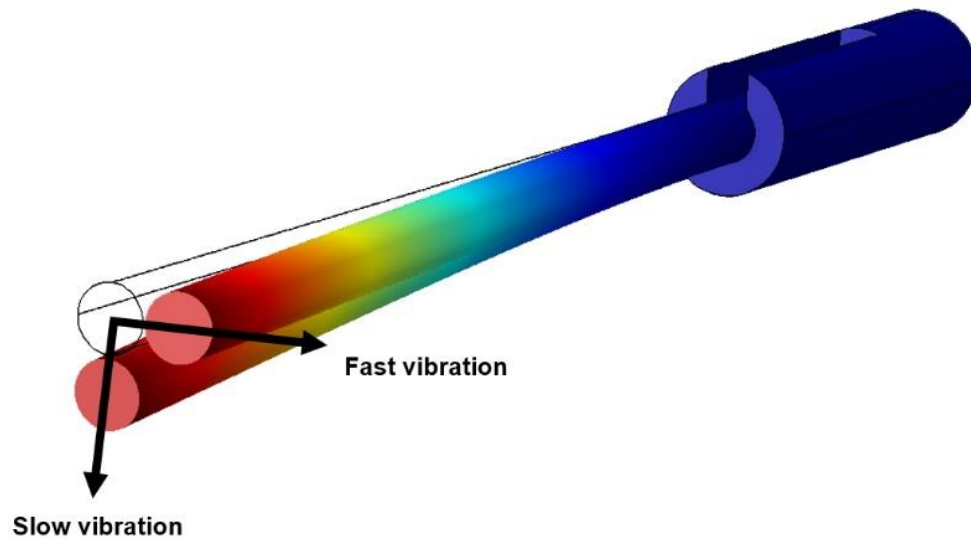
Figure 2.9 Sketch of two vibration planes with different resonance frequency. The plane of lower frequency vibration will pass through the location of the defect sector.
