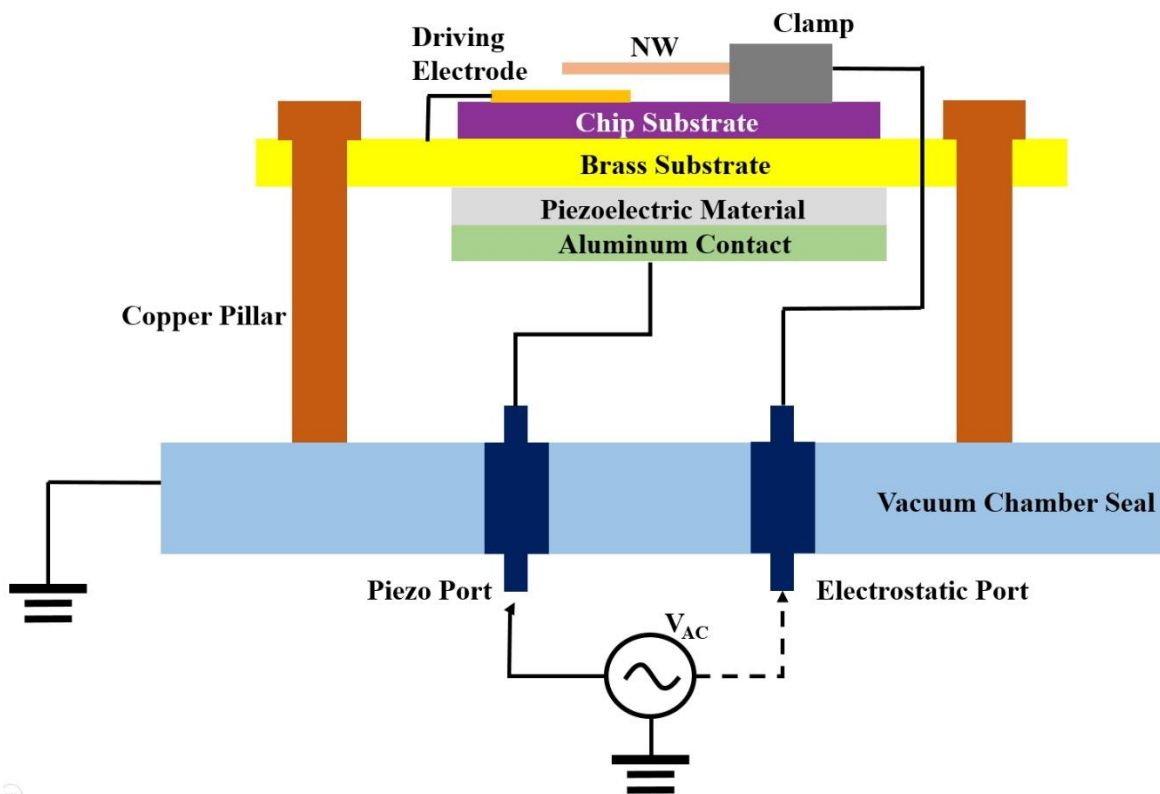
Figure 3.5 Schematic of piezo disk actuation and electrostatic actuation 2-in-1 framework. AC signal output from the spectrum analyzer can be applied either to the piezo port or the electrostatic port, giving a convenient way to switch between two different actuation methods. The piezo port is connected to the aluminum contact on the piezo disk. Clamp of nanowire resonator is wired to the electrostatic port and the driving electrode is grounded through the brass substrate.
