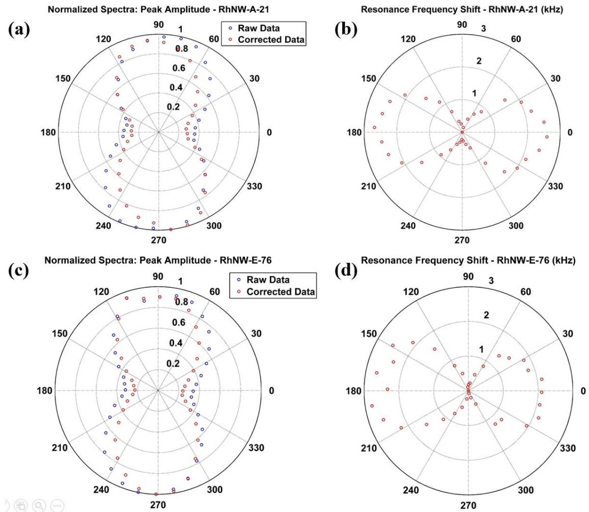
Figure 4.13 a) Normalized resonance peak amplitude for a 360-degree range of orientation angles of RhNW A-21. Blue circles represent measured data without the filter cube installed. Amplitude data shown in red circles is a correction of the round-trip microscope effect applied to the blue circle data. b) Plots of resonance frequency shift, in kHz, at different orientation angles of RhNW A-21. The shift of resonance frequency
