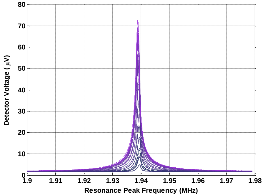
Figure 4.4 Collection of spectra at different laser polarization states. The amplitude of the spectra show a significant variation from 5\mu\text{V} to 73\mu\text{V} at the same laser power. The weakest signal was recorded when the laser polarization was perpendicular to the nanowire axis while the strongest one was achieved with laser polarization parallel to nanowire axis. A small frequency shift can be observed when comparing the peak center frequency of weakest and strongest spectra.
