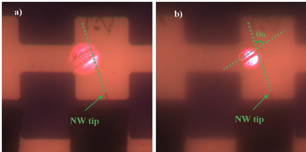
Figure 4.3 CCD images of determining initial orientation angle between nanowire and copper wire shadow. a) Microscope imaging plane is focused on the nanowire and the
