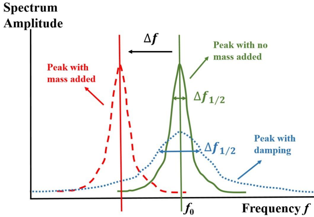
Figure 3.7 Schematic of the spectrum of nanowire resonator. Green solid peak is the natural resonance frequency spectrum. If additional mass is attached to the nanowire, the spectral peak of resonance will shift to a lower frequency as shown by the red dashed curve. Blue dot spectrum shows a low Q-factor spectrum, obtained, for example, if the nanowire resonator is operated in a high fluid damping environment.
