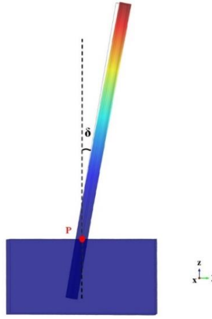
Figure 2.6 Illustration of oblique clamped nanowire resonator model. Nanowire clamped length and free length are both held constant. Clamped angle \delta is varied from 0^\circ to 45^\circ , achieved by rotating the rest position, in steps, about point P .
