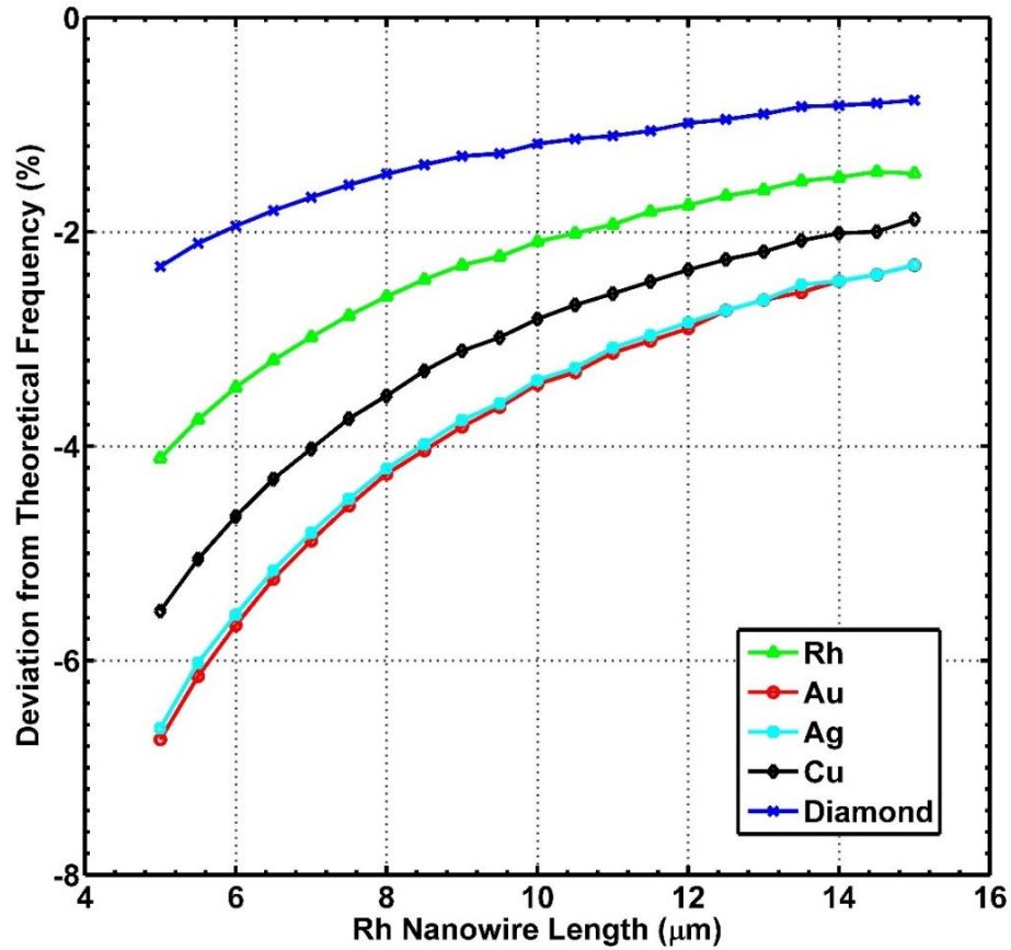
Figure 2.4 Simulation results of resonance frequency deviation from theoretical values versus nanowire length for five clamp materials. The length of the nanowires is varied from 5\mu\text{m} to 15\mu\text{m} ; the diameter is 400\text{nm} and clamp depth is 2\mu\text{m} . The diamond clamp, with highest Young's modulus and lowest Poisson Ratio, shows the least resonance frequency deviation from the ideal situation. Effects of gold and silver clamps on resonance frequency are similar. For all the materials, with increase in the nanowire length, resonance frequency tends to approach the ideal result.
