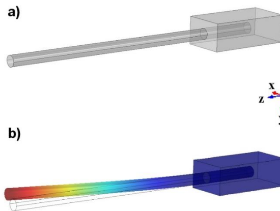
Figure 2.1 a) Three-dimensional model of the clamp for a nanowire resonator in COMSOL simulation. b) Simulation result representing displacement of each part of nanowire resonator with colors.
