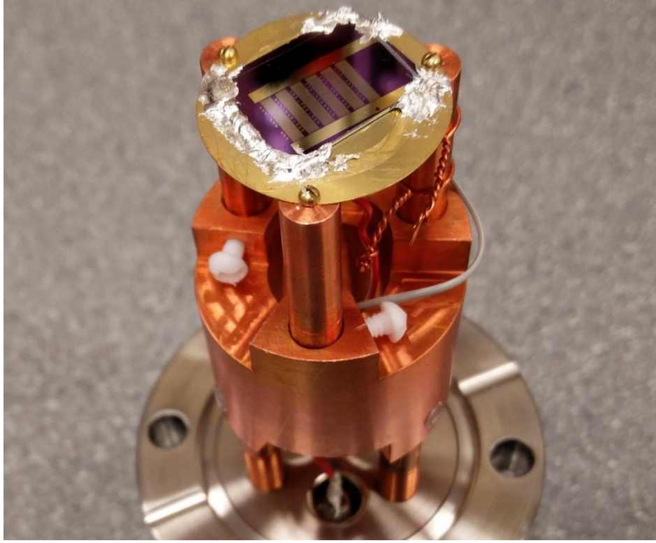
Figure 3.6 Photo of nanowire resonator actuation assembly mounted on the vacuum chamber flange. Piezo disk actuation is used in this setting. Since short circuit would occur on this type of chip, electrostatic actuation was not used for this chip.
