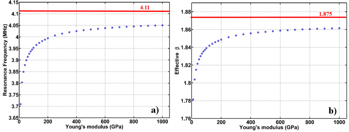
Figure 2.5 a) Resonance frequency as a function of Young's modulus of clamp material; b) Effective \beta_n as a function of Young's modulus calculated from the resonance frequency values in plot a). As the increase of Young's modulus, \beta_n gradually approaches the theoretical value 1.875.
