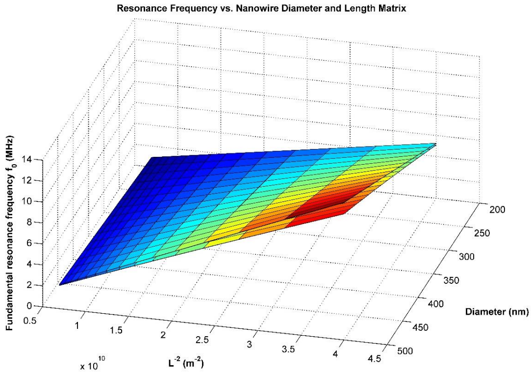
Figure 2.2 3D surface plot of nanowire resonance frequency as a function of nanowire diameter and length. The strongest deviation between the theoretical solution (upper surface) and clamp model simulation (lower surface) in the figure occurs at shorter nanowire length and larger diameter.
