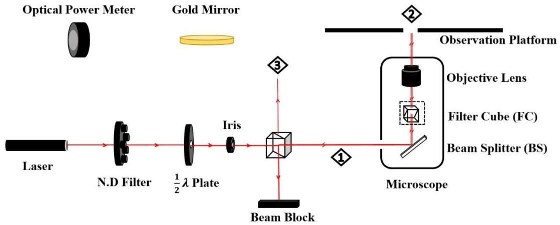
Figure 4.9 Schematic of single-trip and round-trip paths setup for evaluating filter cube and beamsplitter dependencies on input laser polarization. Position 1 is where input laser power measured. For a single-trip path, the laser beam only crosses the microscope once and output laser power is measured at position 2, using the optical power meter. For the round-trip path setup, a gold mirror is fixed at position 2, reflecting the laser back to the microscope and the output laser power is measured at position 3.
