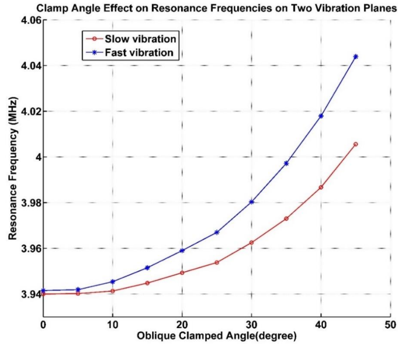
Figure 2.7 Resonance frequencies of two vibration modes for different clamped angles. Symmetry of two vibration modes is reduced with the increase of clamped angle as shown. The final asymmetry approaches 40kHz resonance frequency difference between fast and slow vibration modes, at 45^\circ .
