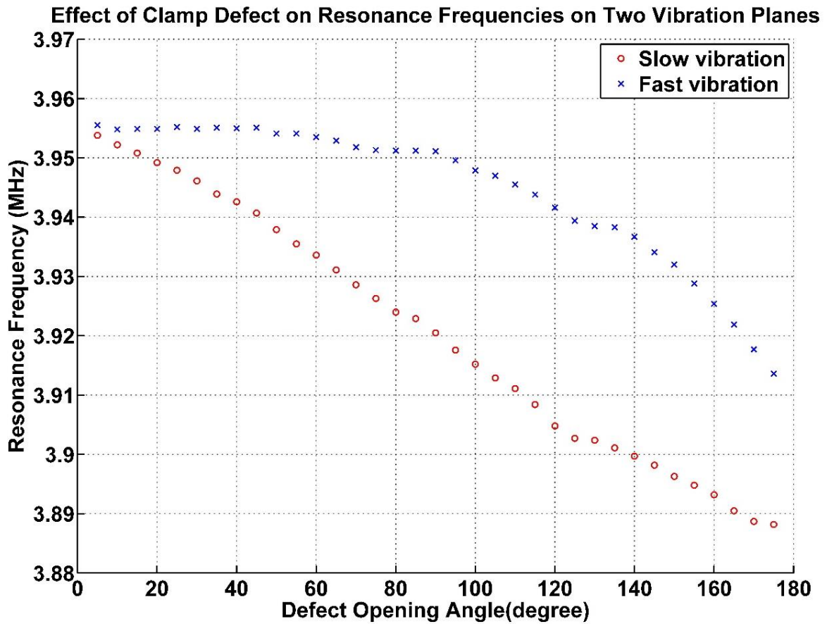
Figure 2.10 Resonance frequencies of fast and slow vibration modes. For a clamp with no defects, resonance frequency values of the fast vibration and slow vibration modes are identical. With increasing defect magnitude, resonance frequencies of the two vibration states diverge significantly.
