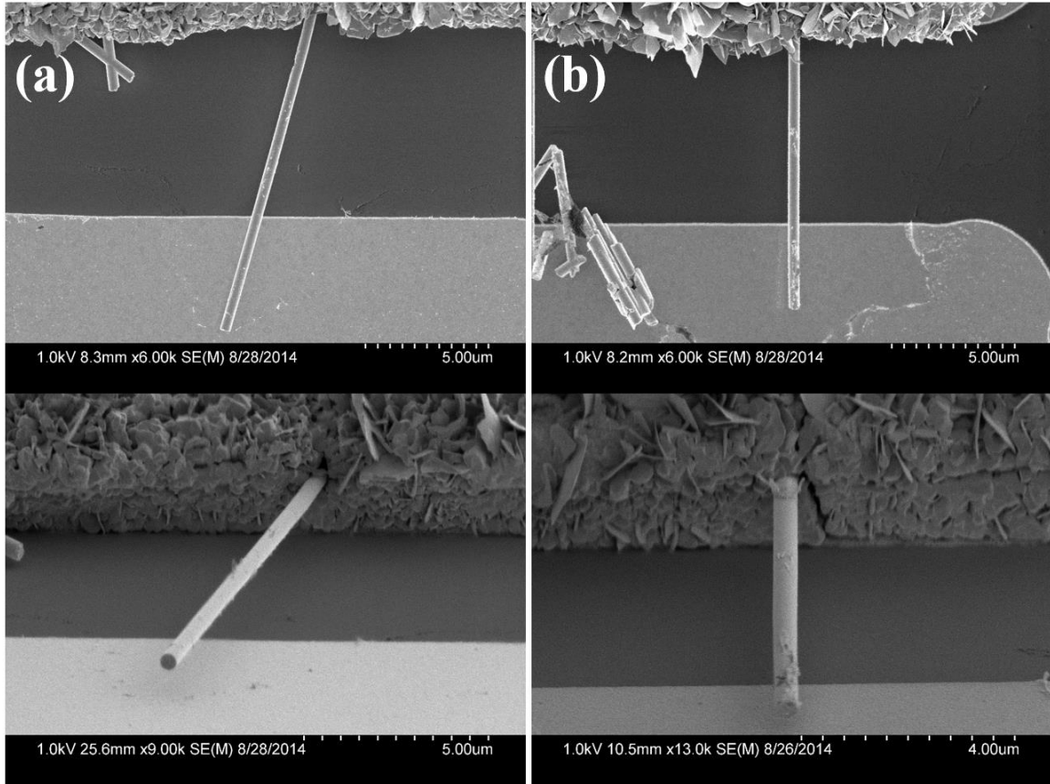
Figure 4.7 SEM images of nanowire's top-view and side-view: a) RhNW A-21; b) RhNW E-76. Both of the nanowires have smooth surface and good clamping condition.
