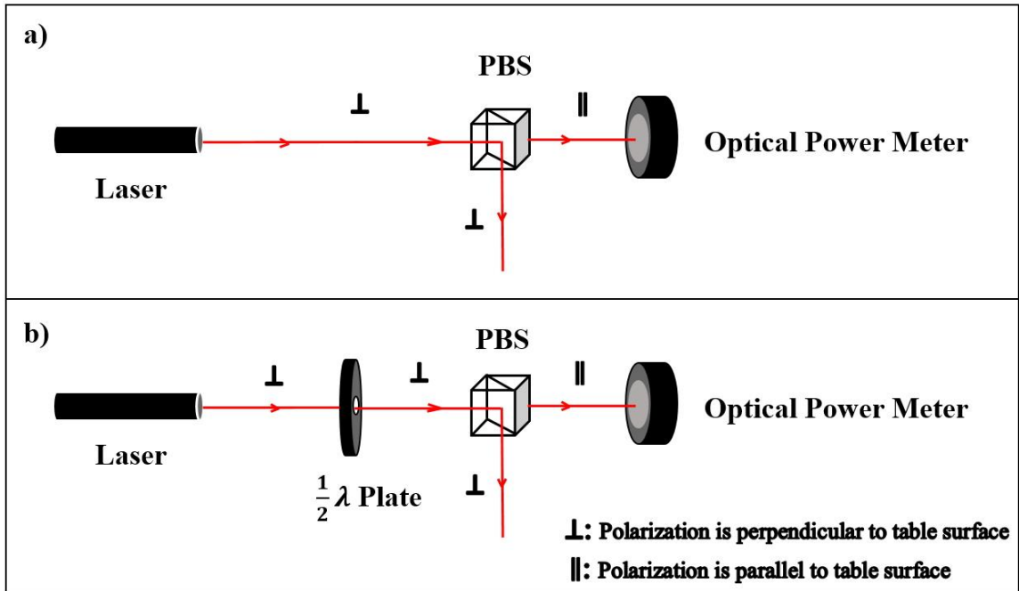
Figure 4.1 a) Alignment of the polarization coming out of laser tube perpendicular to the table surface. Polarizing beamsplitter (PBS) cube only allows the polarization component parallel to the table surface to be transmitted. Therefore, by rotating the laser tube, when polarization is perpendicular to the table surface, minimum power value would be read on power meter. b) Alignment of half-wave plate with its scale. Half-wave plate is rotated until minimum power reading is obtained. Then we set the scale that marks the rotation angle of the half-wave plate to zero.
