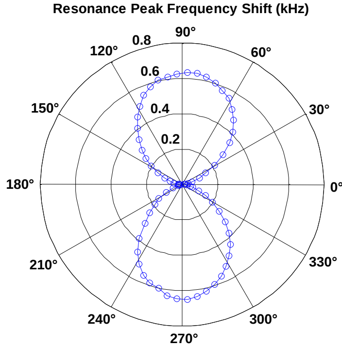
Figure 4.6 Polar plot of resonance frequency shift with an orientation angle variation of 360^\circ . The resonance frequency measured with polarization state parallel to SiNW axis shows the minimum value. Electric field perpendicular to SiNW axis increases the detected resonance frequency about 0.63\text{kHz} .
