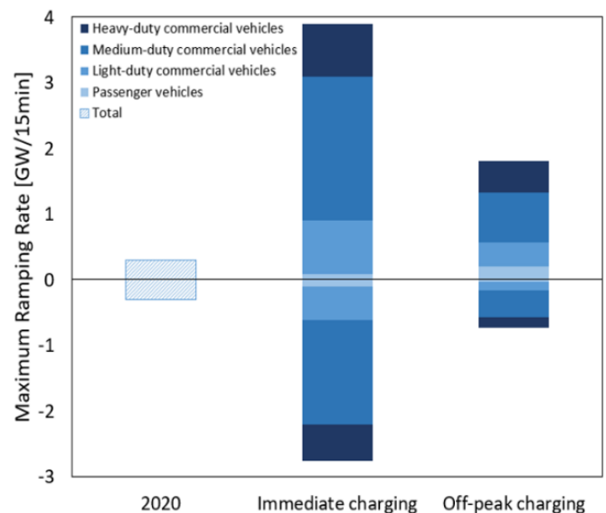
Figure 1: Maximum positive and negative system ramping rates by vehicle weight class in 2050 as compared to historical 2020 ramping rates.
