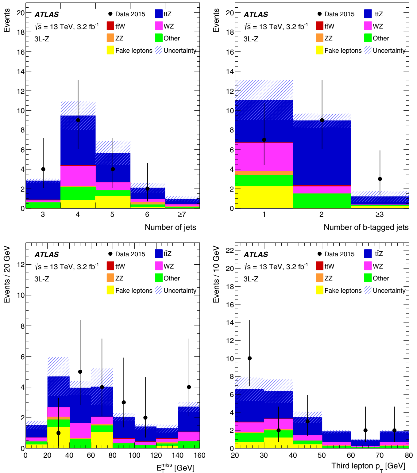
Fig. 4 Distributions of (top left) the number of jets, (top right) the number of b -tagged jets, (bottom left) the missing transverse momentum and (bottom right) the third-lepton p_T , for events contained in any of the three signal regions 3\ell -Z-1b4j, 3\ell -Z-2b3j or 3\ell -Z-2b4j. The distribu-
