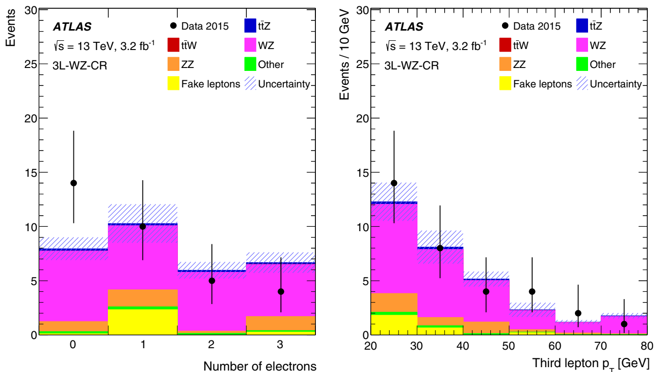
Fig. 2 Distributions of (left) the number of electrons and (right) the third-lepton p_T in the 3\ell -WZ-CR control region before the fit. The background denoted ‘Other’ contains other SM processes producing
