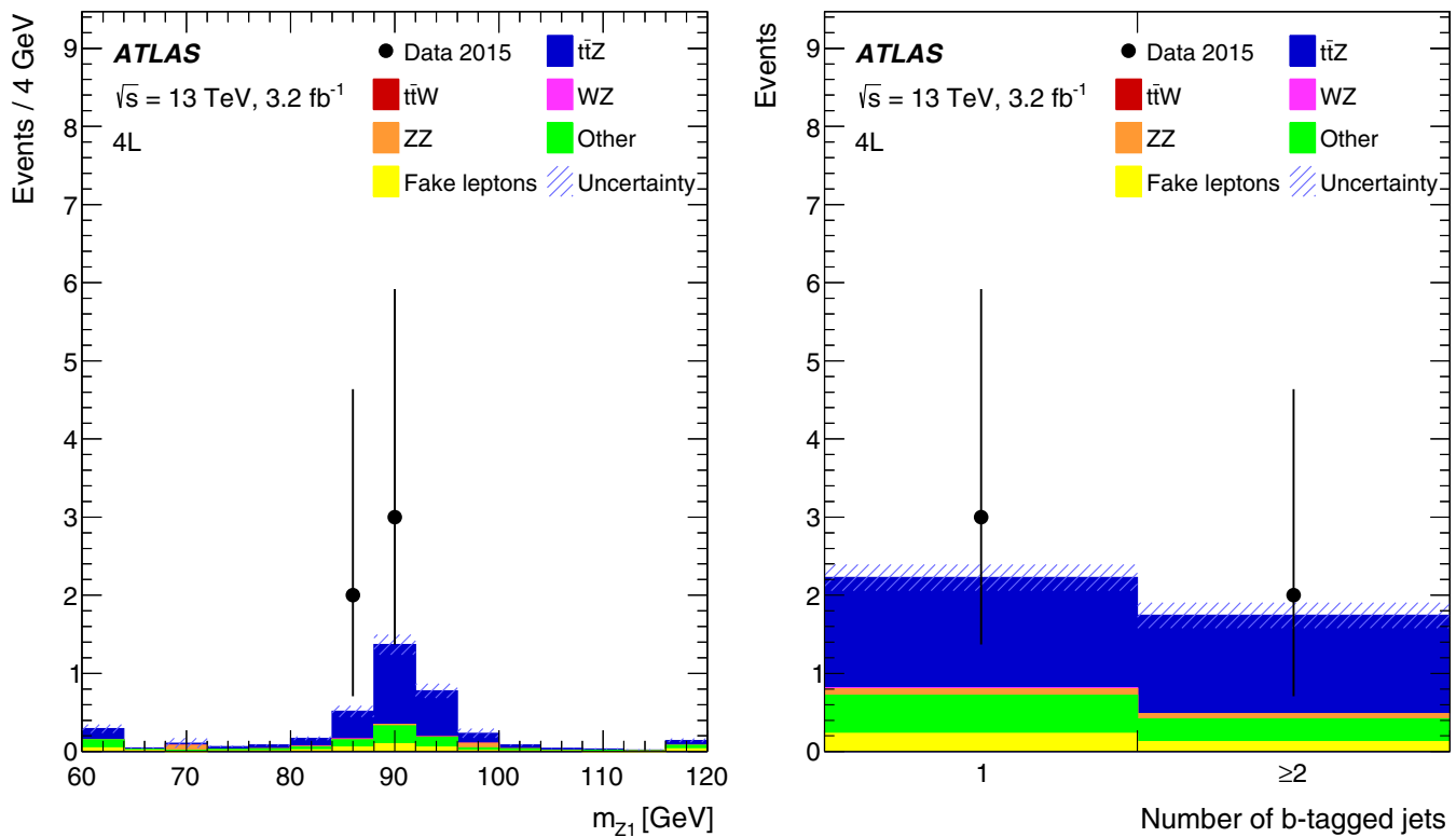
Fig. 6 Distributions (left) of the invariant mass of the OSSF lepton pair closest to the Z boson mass, m_{Z1} , and (right) of the number of b -tagged jets, for events in the tetralepton signal regions. The distributions are shown before the fit. The background denoted ‘Other’ contains
