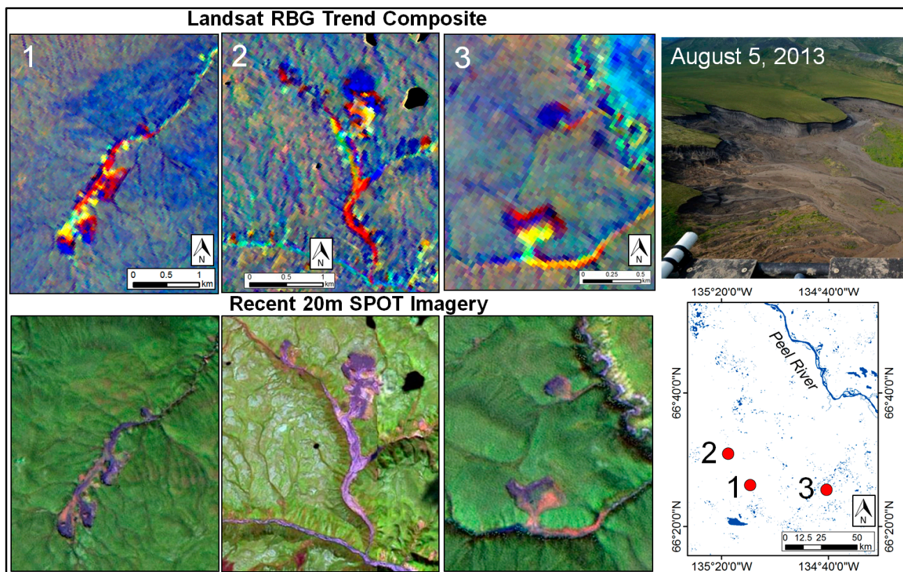
Figure 11. Example TC trend images for three retrogressive thaw slumps within the Peel Plateau region ( top ) with recent SPOT imagery ( bottom ) and an air photo (top right) shown for reference.
