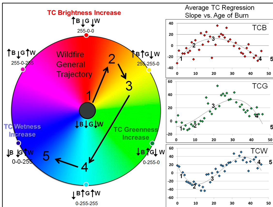
Figure 5. General trajectory of regenerating wildfires in RGB trend space from recently burned forest (1), expanding broadleaf cover (2–3) and succession towards needleleaf species (4–5). Also shown are the linear regression TC slopes averaged by age of burn with third-order polynomial curves overlaid to show the shape of the trajectories. The three TC slope values on the graphs are combined to generate the RGB colour trajectory (left) labelled as 1–5.
