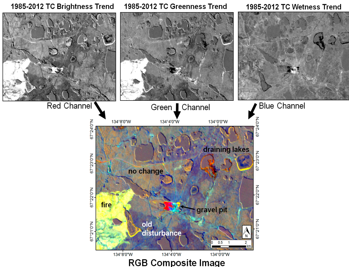
Figure 2. Tasseled Cap (TC) trend compositing method used by LARCH. Individual trend (slope) images from linear regression analysis of the Landsat image stack are composited as an RGB image to yield unique colors representing the three-dimensional TC trajectory.
