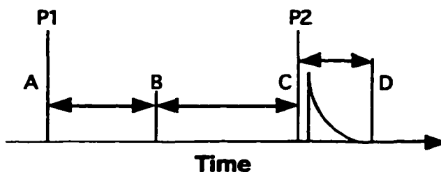
Figure 2.2 Timing diagram for the picosecond fluorescence system.
