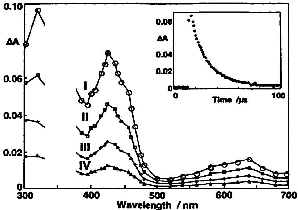
Figure 3.6 Transient absorption spectra of fluorenone in acetonitrile at several delays after the laser pulse: 7 (I), 17 (II), 34 (III), and 43 \mu\text{s} (IV). The inset shows the decay of the triplet excited state monitored at 425 nm. Transient absorption data was not collected in the region of the laser excitation wavelength ( 355 \pm 15 nm).
