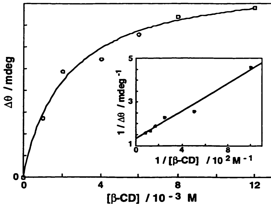
Figure 4.8 Nonlinear fit of the ICD signal at 320 nm for fluorenone in the presence of various \beta -CD concentrations. The solid line corresponds to the fit obtained from using Equation 1.20. The inset shows the double reciprocal plot for the same data.
