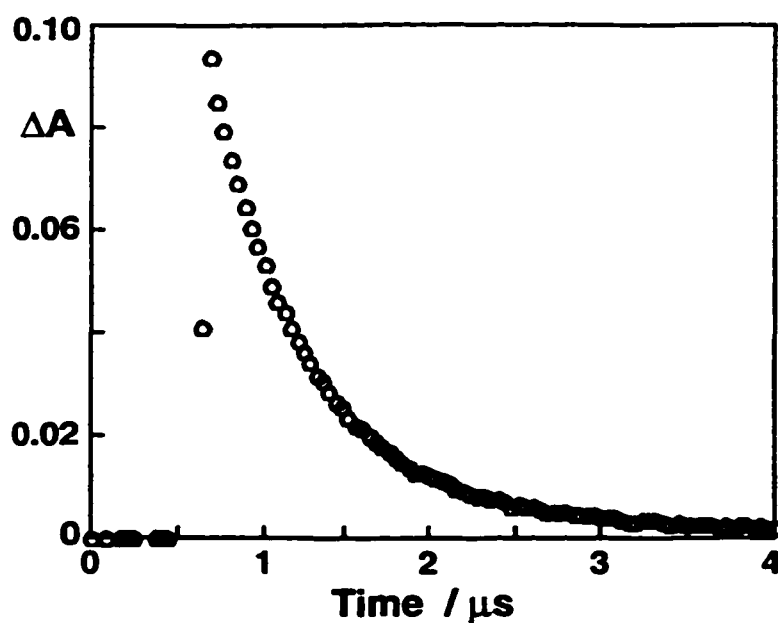
Figure 5.9 Decay of the radical cation of 4-VA in water purged with N_2O . The kinetic trace was monitored at 600 nm.
