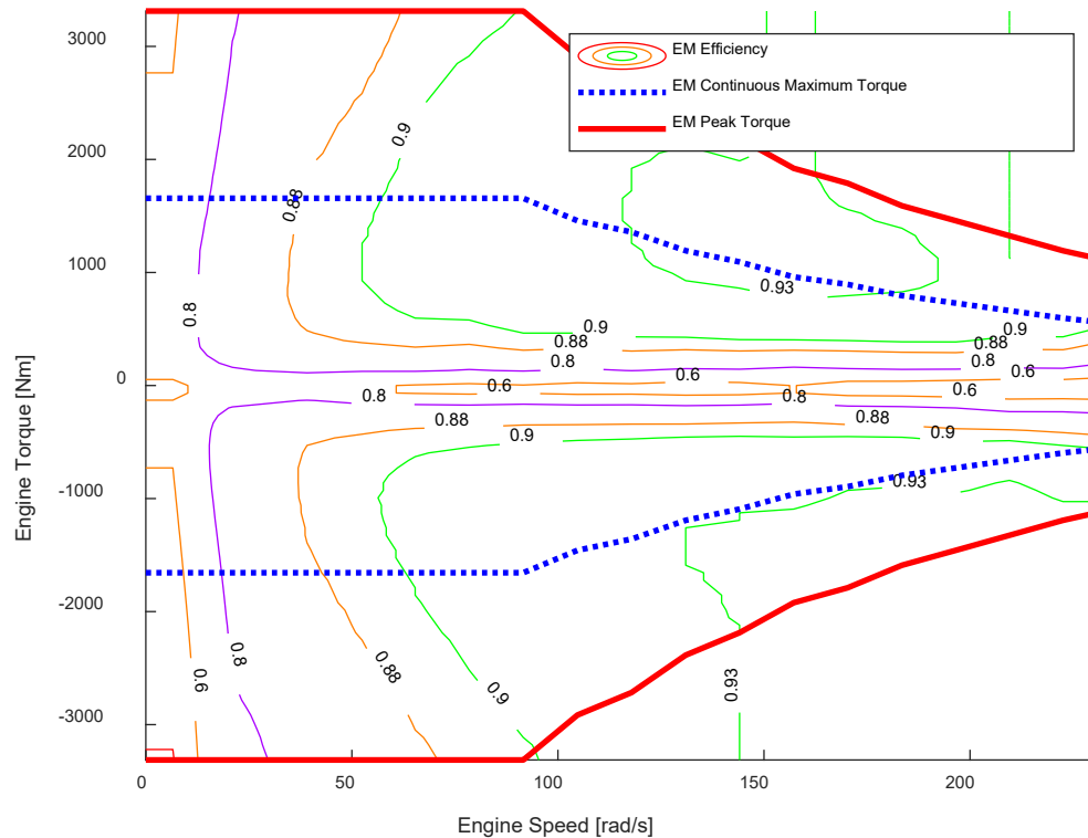
Figure 15 Electric machine combined efficiency map
