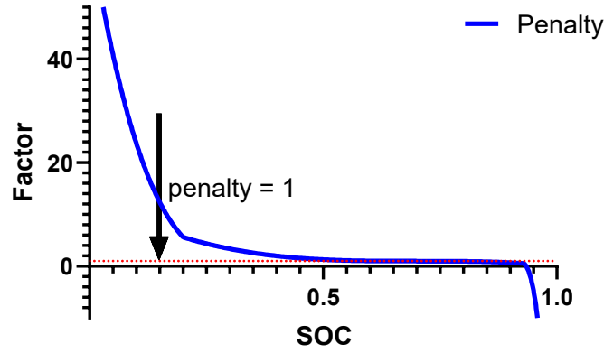
Figure 41 Penalty Function
