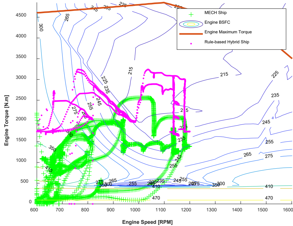
Figure 37 Engine 1 Operation Points
