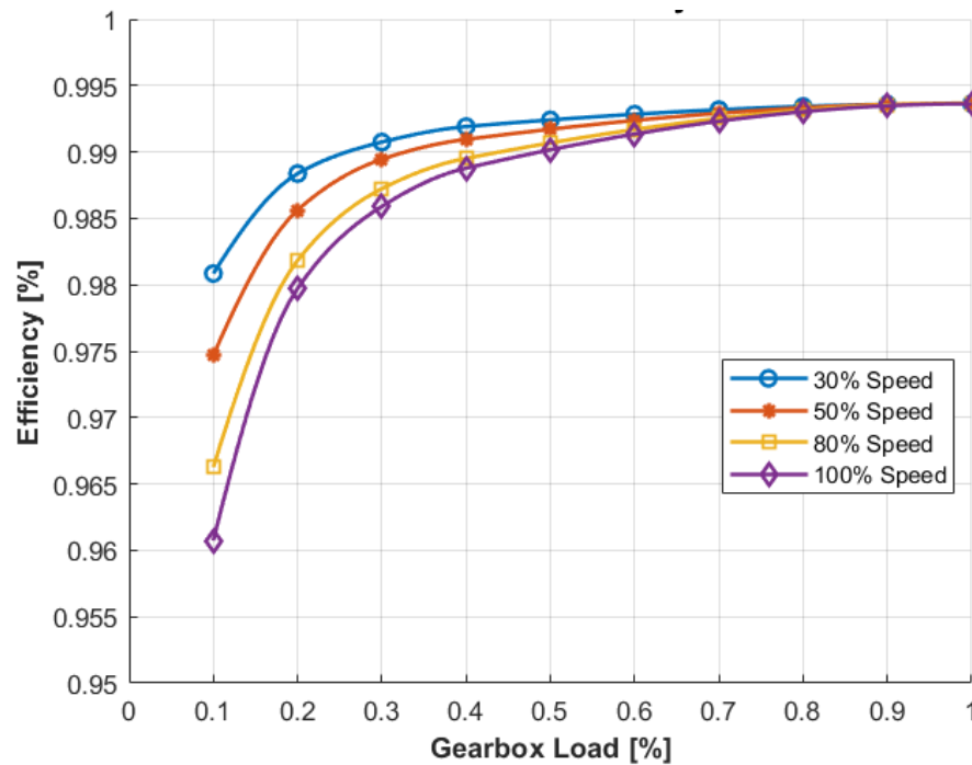
Figure 16 Gearbox Efficiency
