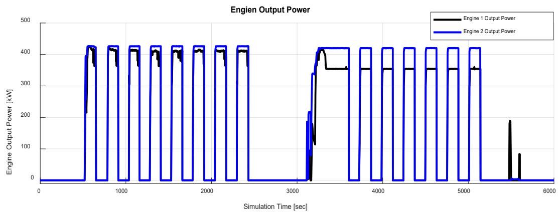
Figure 55 Engines' Power
