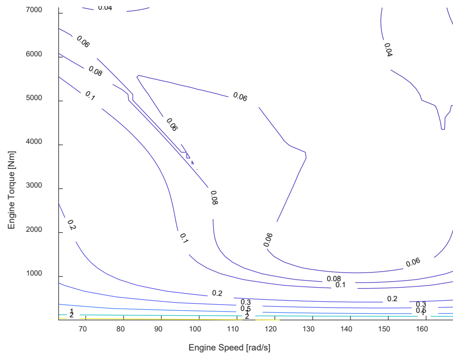
Figure 12 Engine HC map
