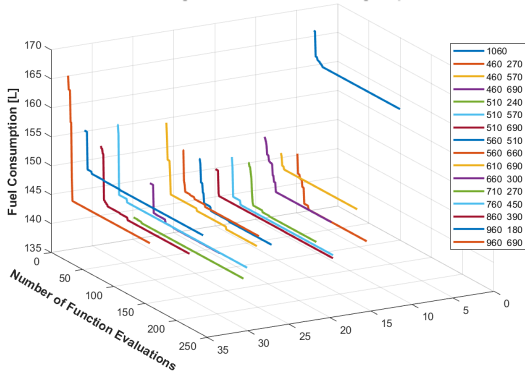
Figure 59 MSSR Inner Loop Searching Process (Multi-Component Sizes)
