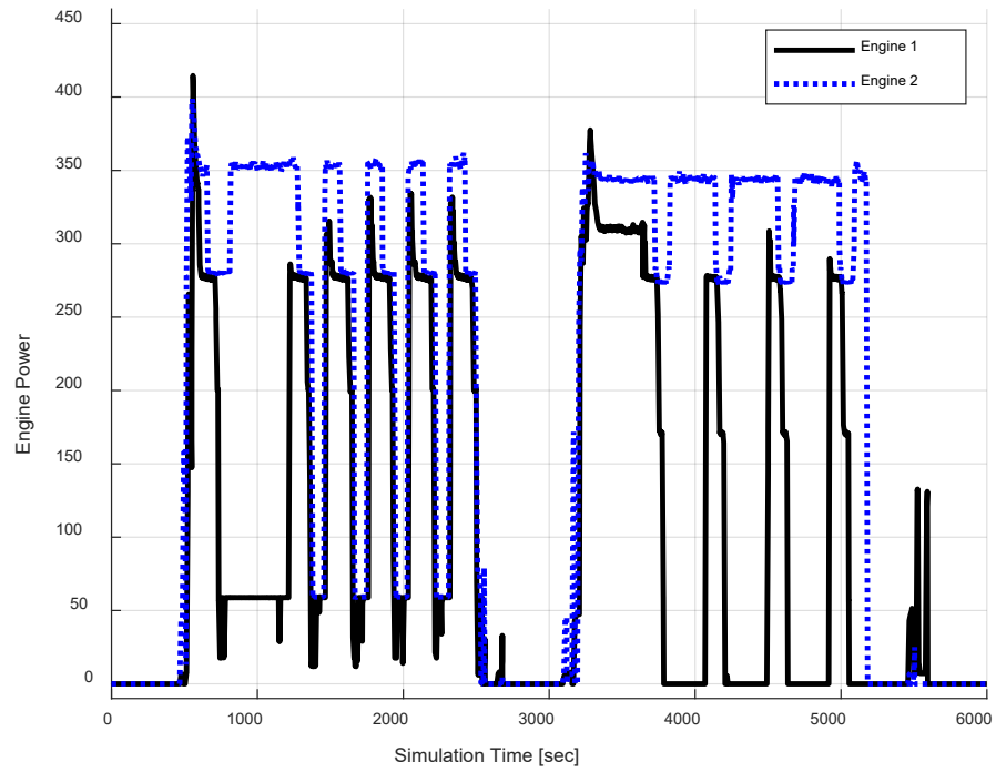
Figure 43 Engines' Power
