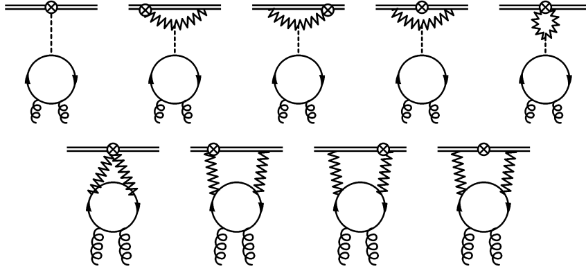
Fig. 3. Diagrams contributing to 1/M gluon matching, with the same notation as in Fig. 1. Curly lines denote gluons. Diagrams with both gluons attached to the upper quark line or with one gluon attached to each of the upper and lower quark lines are not shown.
