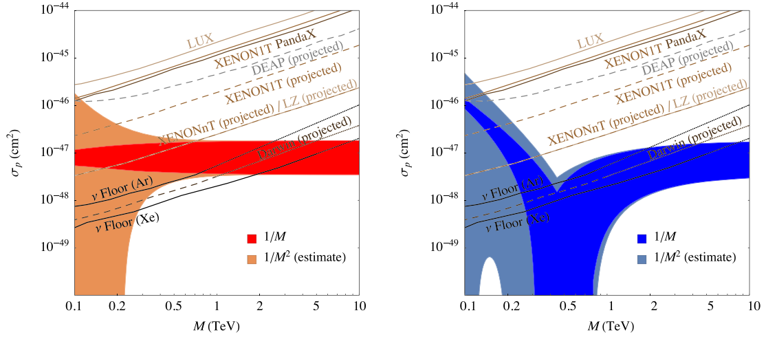
Fig. 4. The WIMP-proton scattering cross section as a function of WIMP mass M for a Majorana WIMP (left panel) and a scalar WIMP (right panel), which correspond to the c_H values in Eqs. (3) and (5), respectively. The inner band is the cross section obtained from the scalar and tensor amplitudes computed through \mathcal{O}(1/M) . The outer band includes an estimate for the \mathcal{O}(1/M^2) contributions. The neutrino floor for both Argon and Xenon direct detection experiments are from Ref. [48], and are shown by black solid lines; our extrapolation to larger masses is denoted with black dashed lines. Also shown with solid lines are the current bounds from LUX [49], XENON1T [50], and PandaX-II [51]. Projected sensitivities of future experiments are shown with dotted lines: DEAP-3600 [52], XENON1T and XENONnT [53], LZ [54], and DARWIN [55].
