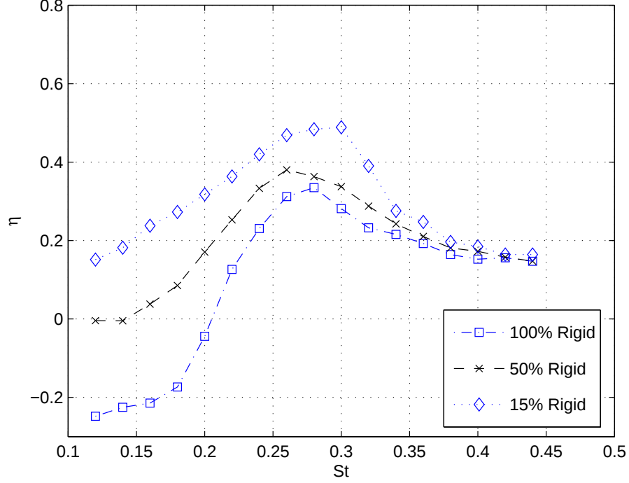
Figure 3.5: Experimentally measured efficiency \eta as a functions of Strouhal number St for three types of flexible plates, 1 : 0 ratio: h = 17cm , r = 20cm , f = 10cm , \alpha_{max} = 8^\circ , h_0 \in [6.4cm, 23.6cm] , \varphi = 90^\circ ; 1 : 1 ratio: h = 17cm , r = 10cm , f = 0cm , \alpha_{max} = 8^\circ , h_0 \in [7.3cm, 26.9cm] , \varphi = 90^\circ ; 1 : 6 ratio: h = 17cm , r = 3cm , f = 17cm , \alpha_{max} = 8^\circ , h_0 \in [6.8cm, 24.8cm] , \varphi = 90^\circ .
