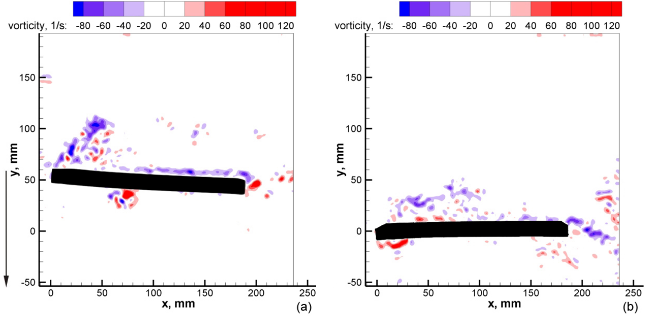
Figure 3.10: PIV vorticity patterns(frames 338 and 389) for the case C for 1 : 6-ratio plate: h = 17\text{cm} , r = 3\text{cm} , f = 17\text{cm} , \alpha_{\max} = 8^\circ , h_0 = 8\text{cm} , \varphi = 90^\circ , St = 0.26 , f_{osc} = 0.36\text{Hz} , T = 2.8\text{s}
