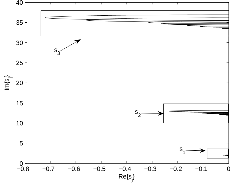
Figure 5.1: Root-locus of complex natural frequencies s_1, s_2, s_3 obtained for 12 different positions of the PZT patches and with increasing damping coefficients.
