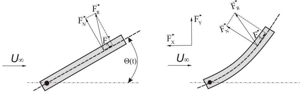
Figure A.1: Force distribution at the center of pressure of the rigid and flexible plates.
