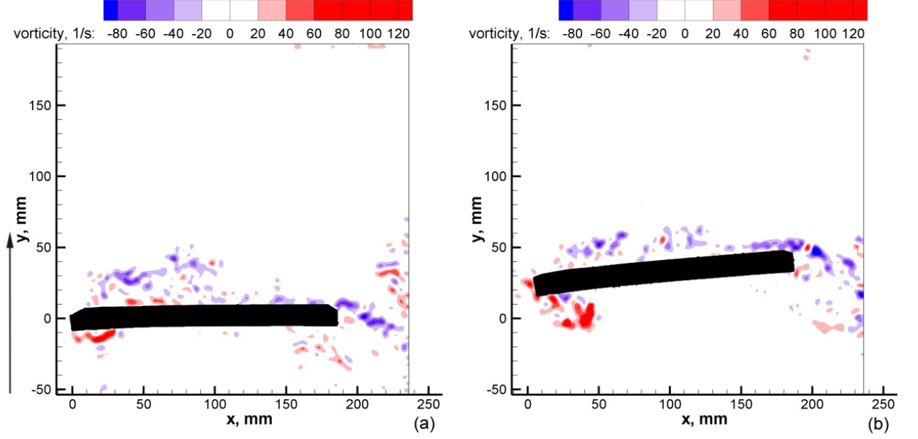
Figure 3.11: PIV vorticity patterns(frames 572 and 656) for the case C for 1 : 6-ratio plate: h = 17\text{cm} , r = 3\text{cm} , f = 17\text{cm} , \alpha_{\max} = 8^\circ , h_0 = 8\text{cm} , \varphi = 90^\circ , St = 0.26 , f_{osc} = 0.36\text{Hz} , T = 2.8\text{s}
