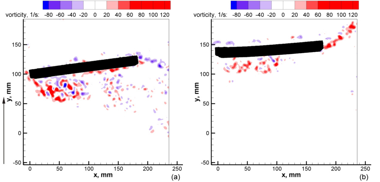
Figure 3.12: PIV vorticity patterns(frames 795 and 960) for the case C for 1 : 6-ratio plate: h = 17\text{cm} , r = 3\text{cm} , f = 17\text{cm} , \alpha_{\max} = 8^\circ , h_0 = 8\text{cm} , \varphi = 90^\circ , St = 0.26 , f_{osc} = 0.36\text{Hz} , T = 2.8\text{s}
