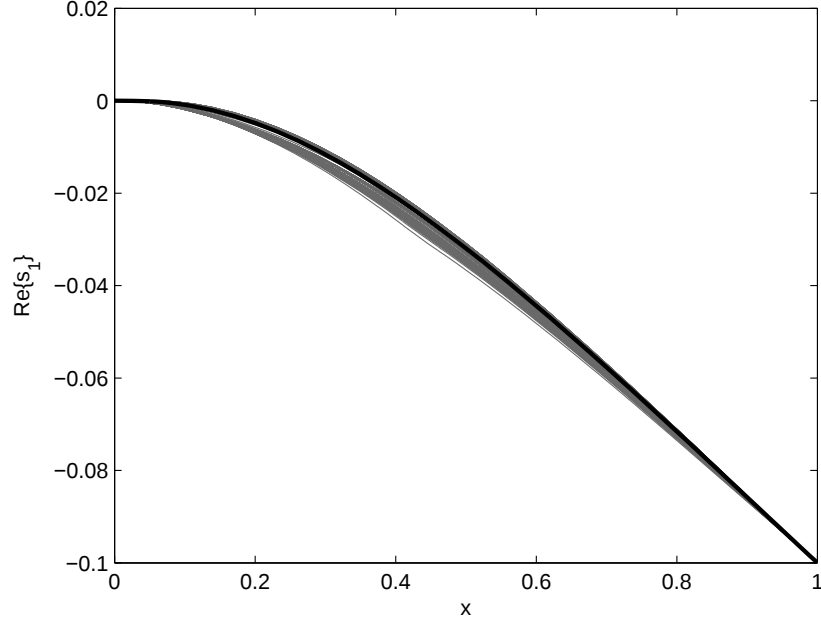
Figure 5.5: Envelope of the first mode shapes obtained at each of the 12 PZT locations considered in this study.
