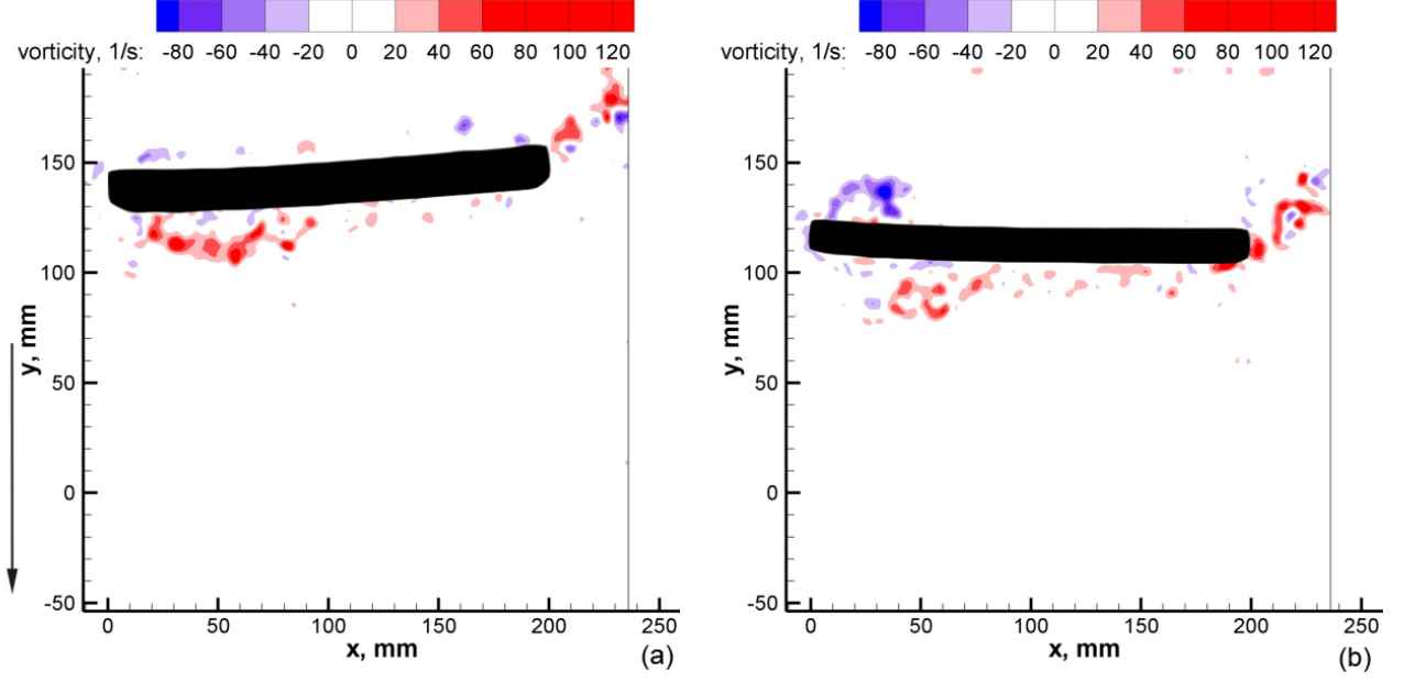
Figure 3.9: PIV vorticity patterns(frames 120 and 227) for the case C for 1 : 6-ratio plate: h = 17\text{cm} , r = 3\text{cm} , f = 17\text{cm} , \alpha_{\max} = 8^\circ , h_0 = 8\text{cm} , \varphi = 90^\circ , St = 0.26 , f_{osc} = 0.36\text{Hz} , T = 2.8\text{s}
