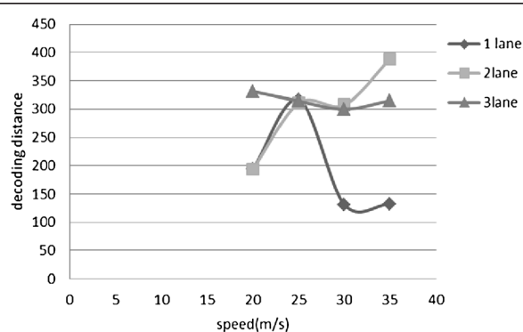
Figure 16 Effect of increased vehicle speed on the decoding distance for different numbers of road lanes.
