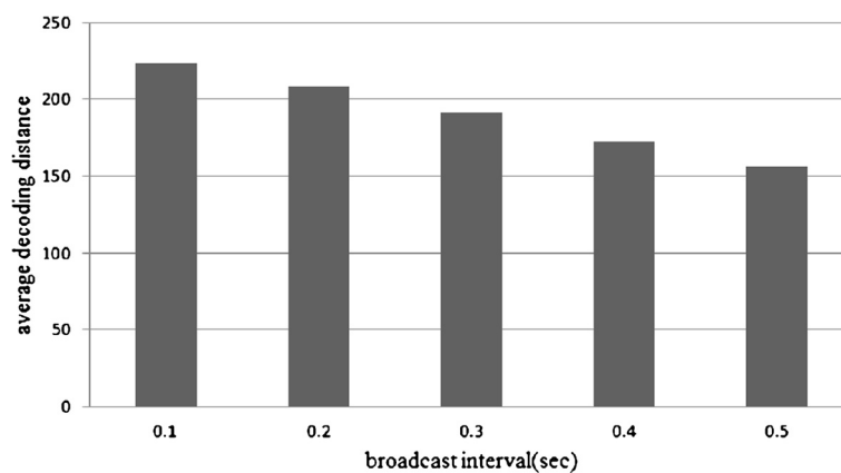
Figure 19 The effect of changing the time interval between two successive broadcasts on the decoding distance. Increasing the broadcast interval decreases the average decoding distance.
