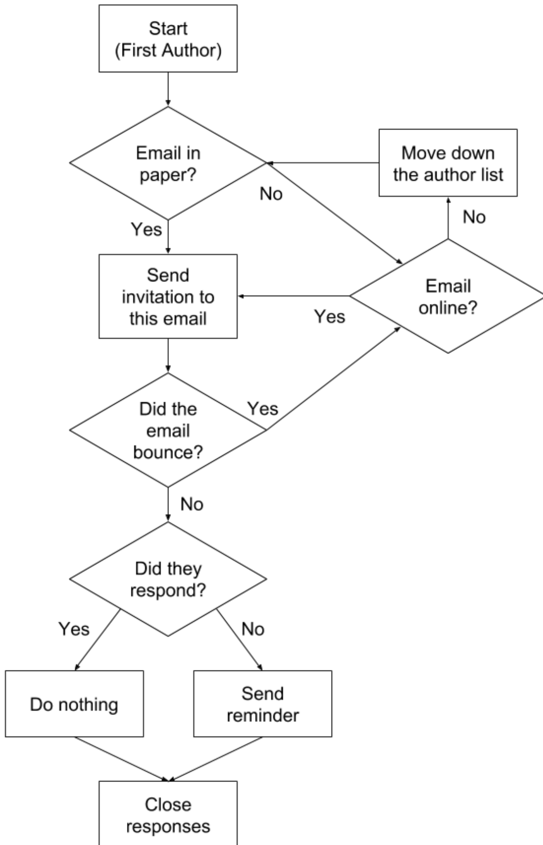
Figure 5.3: The survey dissemination process
