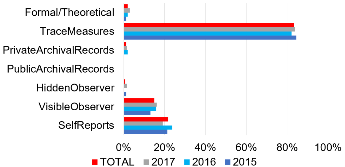
Figure 6.2: Data sources included in ICSE papers before systematic mapping study validation.
