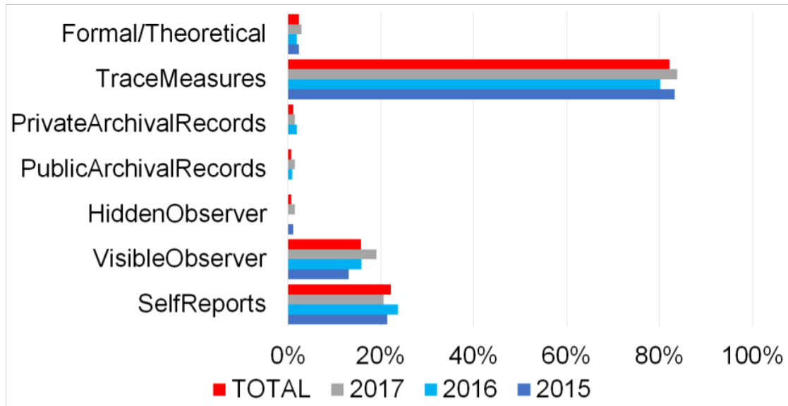
Figure 6.4: Data sources included in ICSE papers, corrected after member checking.
