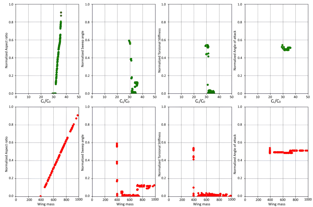
Figure 4. Distribution of optimization solutions along design variable boundaries for both objectives: C_L/C_D maximization (above, in green) and mass minimization (below, in red). Units of mass are given in kg.
