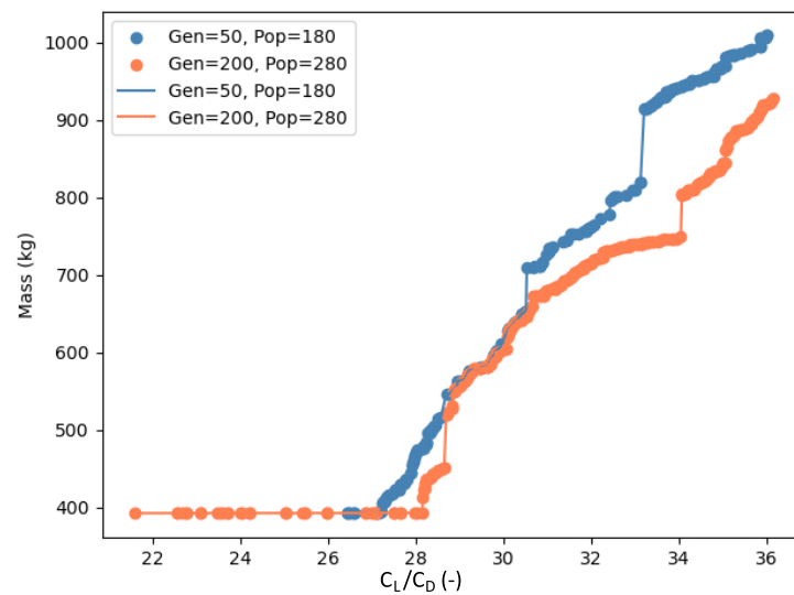
Figure 6. Pareto fronts for Case 2 (cruise speed of 60 m/s).
