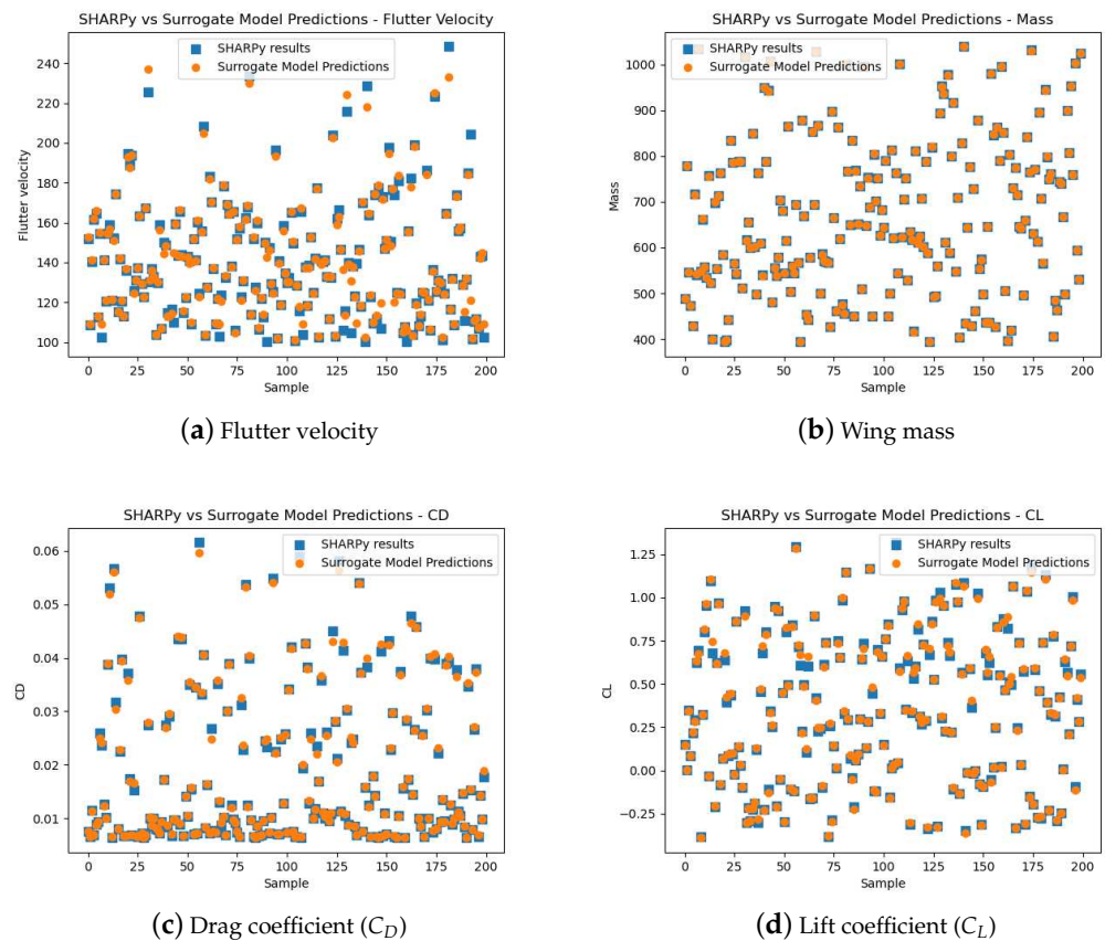
Figure 2. Visual comparison of the results obtained using the SHARPy simulations (in blue) and the surrogate model (in orange) in the testing phase of the SMs.
