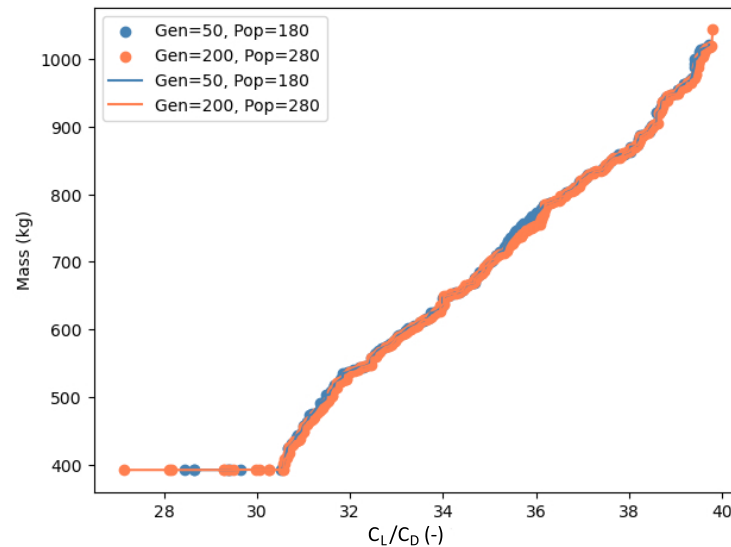
Figure 5. Pareto fronts for Case 1 (cruise speed of 30 m/s).
