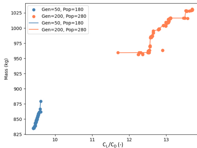
Figure 7. Pareto fronts for Case 3 (cruise speed of 130 m/s).
