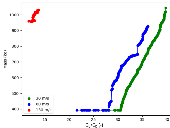
Figure 8. Pareto fronts across analyzed cruise speeds.
