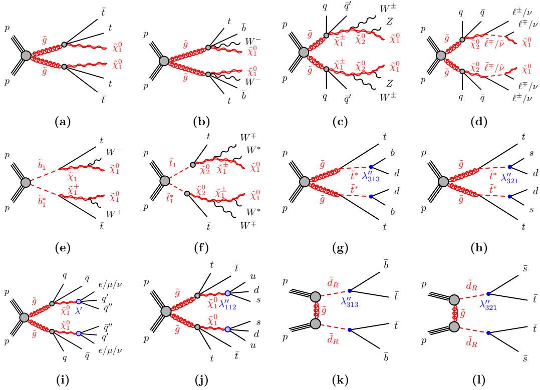
Figure 1. RPC SUSY processes featuring gluino ((a), (b), (c), (d)) or third-generation squark ((e), (f)) pair production studied in this analysis. RPV SUSY models considered are gluino pair production ((g), (h), (i), (j)) and t-channel production of down squark-rights ((k), (l)) which decay via baryon- or lepton-number violating couplings \lambda'' and \lambda' respectively. In the diagrams, q \equiv u, d, c, s and \ell \equiv e, \mu, \tau . In figure 1d, \tilde{\ell} \equiv \tilde{e}, \tilde{\mu}, \tilde{\tau} and \tilde{\nu} \equiv \tilde{\nu}_e, \tilde{\nu}_\mu, \tilde{\nu}_\tau . In figure 1f, the W^* labels indicate largely off-shell W bosons — the mass difference between \tilde{\chi}_1^\pm and \tilde{\chi}_1^0 is around 1 GeV.
