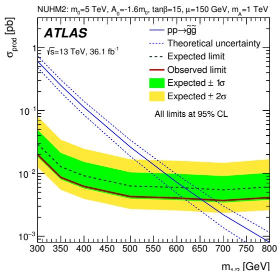
Figure 6. Observed and expected exclusion limits as a function of m_{1/2} in the NUHM2 model [31, 32]. The signal region R pc 2L2bH is used to obtain the limits. The contours of the green (yellow) band around the expected limit are the \pm 1\sigma ( \pm 2\sigma ) results, including all uncertainties. The limits are computed at 95% CL.
