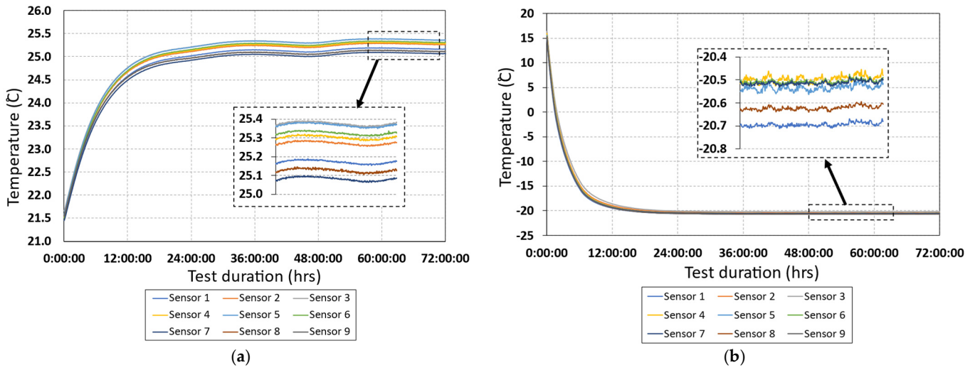
Figure 6. Air curtain temperature profile of: (a) metering chamber; (b) climate chamber.
