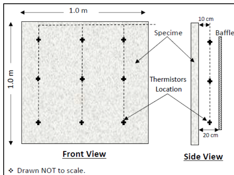
Figure 5. Scheme of temperature sensors' layout.
