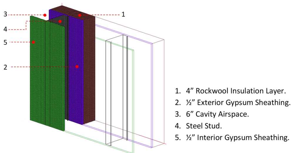
Figure 11. Sketch of the tested wall assembly.
