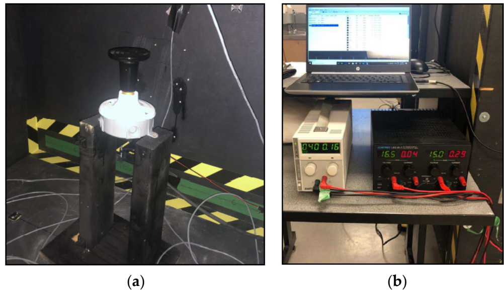
Figure 3. (a) Ceramic heat bulb; (b) DC power supply regulator.
