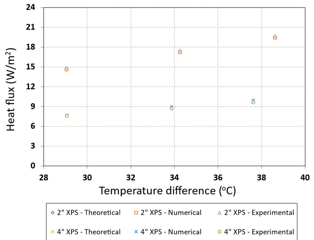
Figure 8. Comparison between theoretical, numerical, and experimental heat flow rates.
