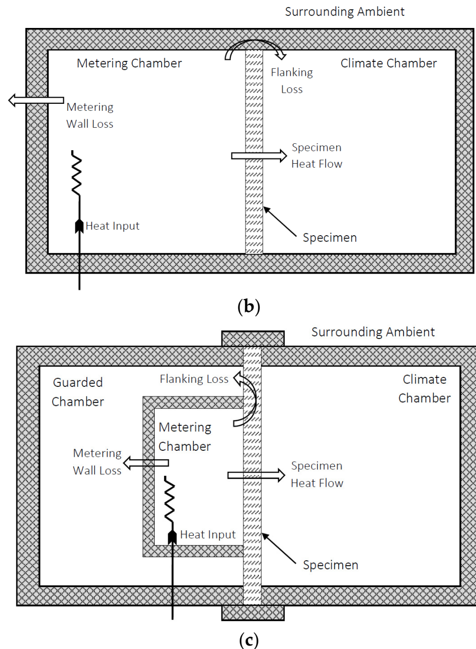
Figure 1. Schematics of: (a) guarded hot plate; (b) calibrated hot box; (c) guarded hot box.
