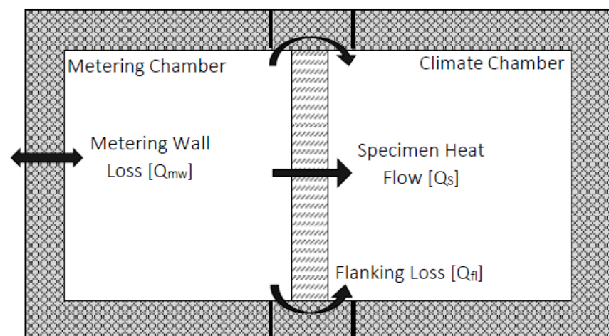
Figure 9. Scheme of heat flow paths.
