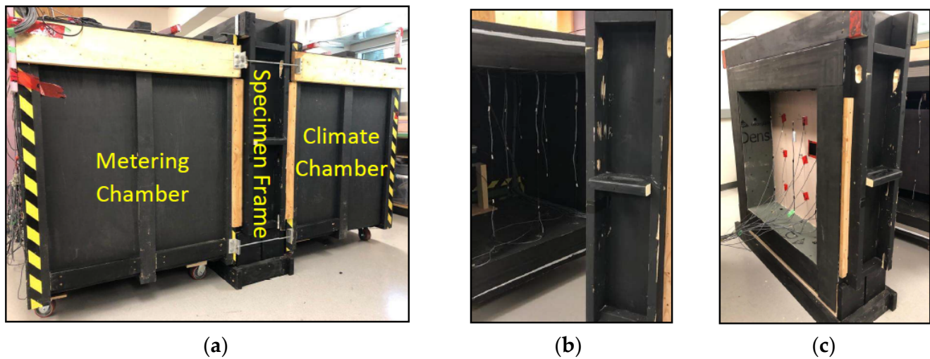
Figure 2. (a) Environment chamber; (b) interior view of the chamber; (c) specimen frame.
