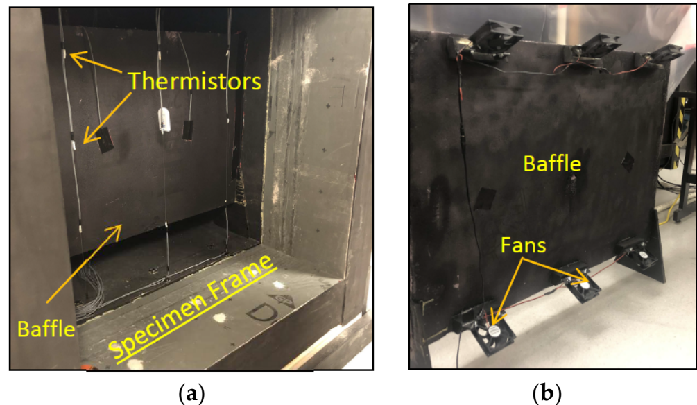
Figure 4. (a) Radiation baffle element; (b) fans attached to the baffle.
