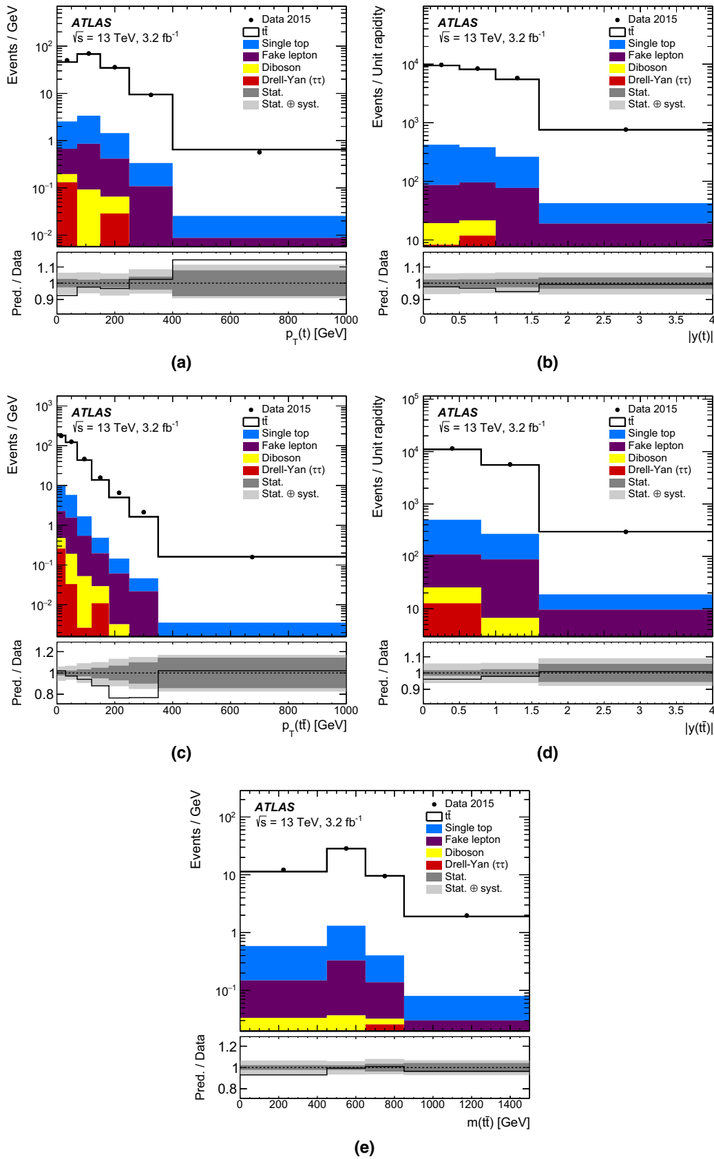
Fig. 2 Kinematic distributions for the p_T(t) (a), |y(t)| (b), p_T(t\bar{t}) (c), t\bar{t} |y_{t\bar{t}}| (d), and m(t\bar{t}) (e) after reconstruction of the t\bar{t} system. In all figures, the rightmost bin also contains events that are above the x -axis range. The uncertainty bands represent the statistical uncertainties
