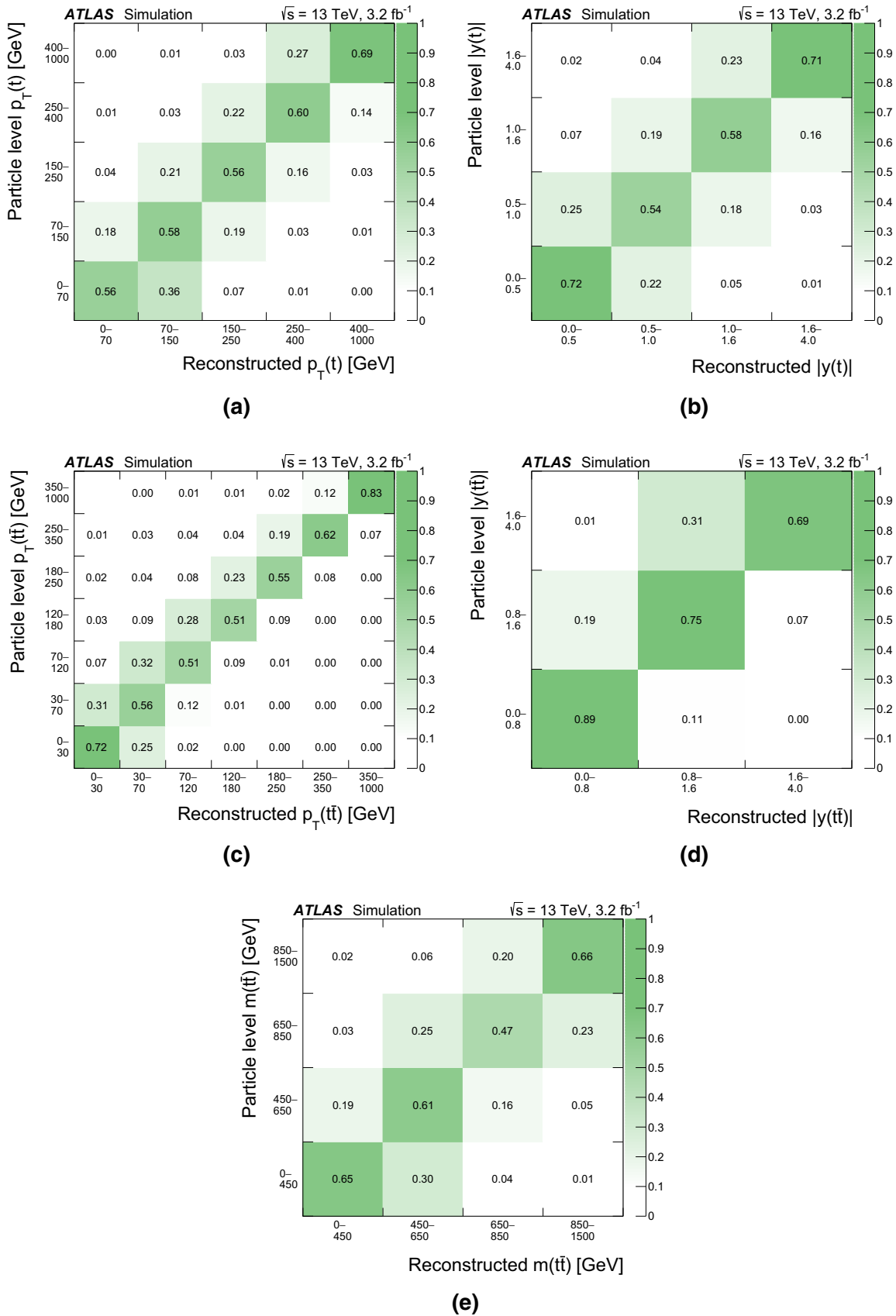
Fig. 3 The response matrices for the observables from the nominal t\bar{t} MC, normalised by row to unity. Each bin shows the probability for a particle-level event in bin i to be observed in a reconstruction-
