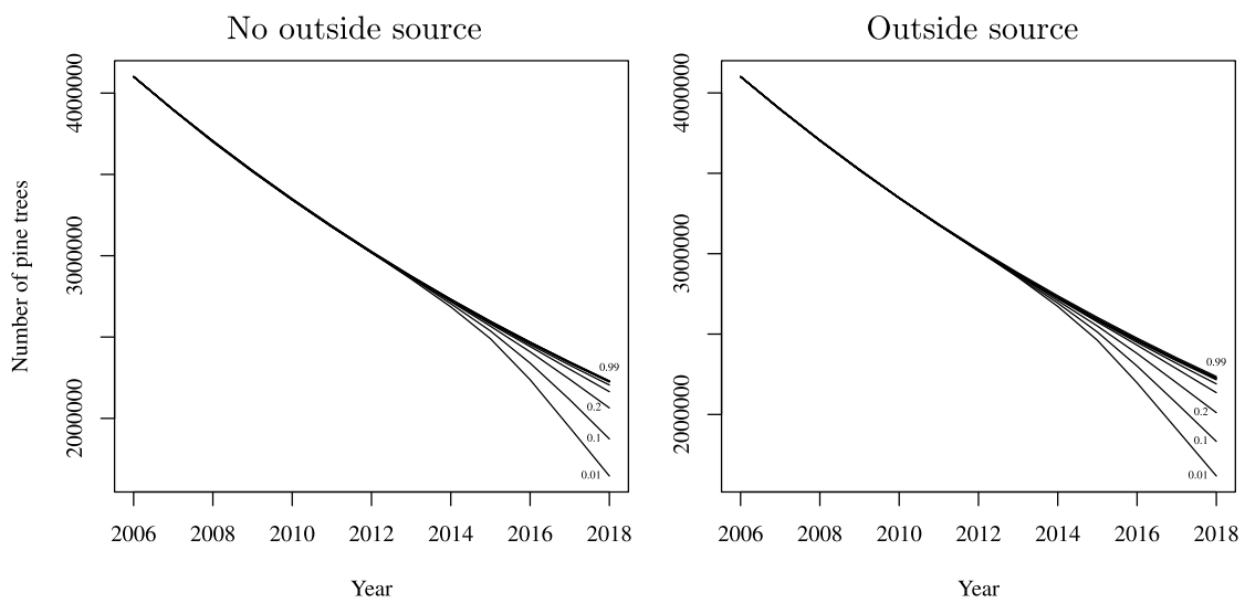
Fig. 5. Total number of pine trees in the domain \sum_x H_x^t without (left) or with (right) outside source of beetles for control rates between 0.01 and 0.99. Each line represents the average over 1000 simulations for a control rate.
