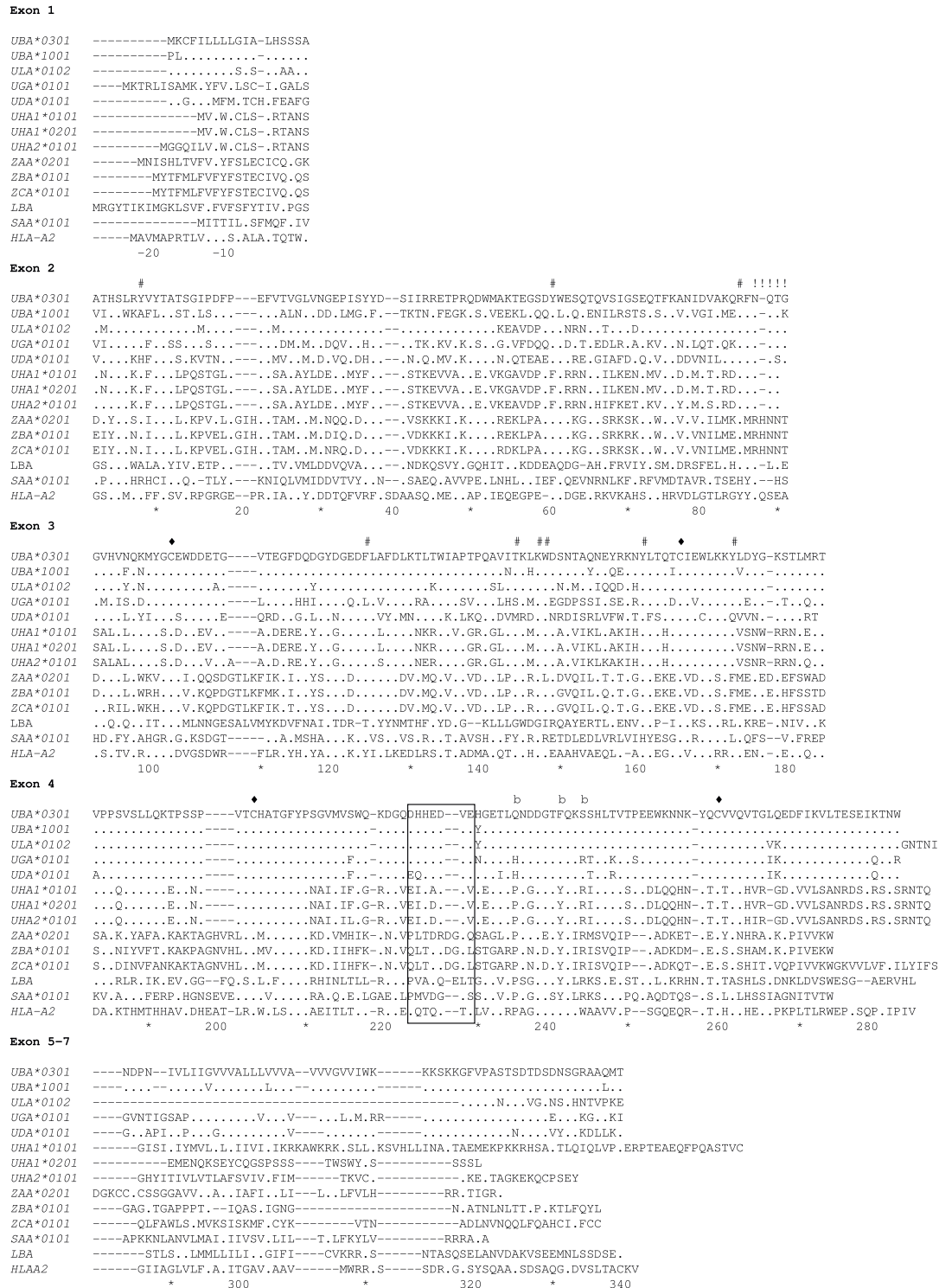
Figure 5 Alignment of Atlantic salmon MHC class I sequences. Comparison of Atlantic Salmon UBA*0301 [Genbank: AAN75116], UBA*1001 [Genbank: AAN75118], ULA [Genbank: ABQ59666], UGA, UDA, UHA1, UHA2, ZAA, ZBA, ZCA, SAA (described in this paper), LBA [Genbank: DY733800 and GO062643] and HLA-A2 [Genbank: AAA76608]. Dots indicate identities, dashes indicate gaps or missing sequence information. Cysteine residues involved in putative Ig fold are marked ♦ above sequences. Anchor residues known to bind the ends of peptide are marked # based on mammalian positions. Unique N-linked glycosylation sites are marked ! and CD8 binding site are boxed based on the acidic stretch from mammalian. b defines Z, S, L and UHA residues potentially involved in interactions with a different beta2-microglobulin. Individual domains/exon for LBA are based on the Sasa -UBA*0301 sequence.
