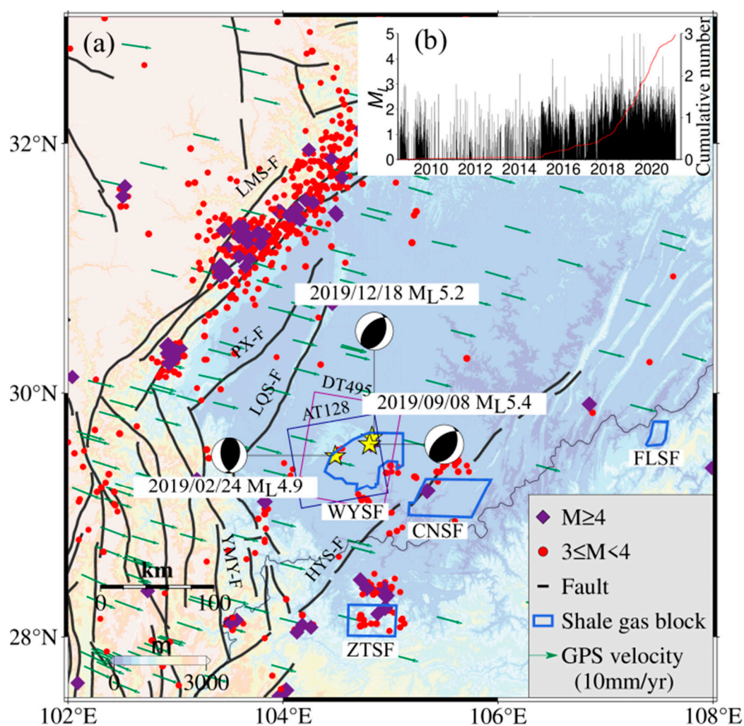
Figure 1. (a) Structural background of Sichuan Basin; (b) seismic activity distribution in the Weiyuan-Rongxian shale gas field.
