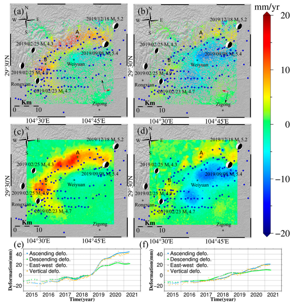
Figure 3. (a) Ascending LOS deformation velocity of the Weiyuan-Rongxian shale gas field over 2015–2021. (b) Descending LOS deformation velocity of the Weiyuan-Rongxian shale gas field over 2015–2021. (c) Vertical deformation velocity of the Weiyuan-Rongxian shale gas field over 2015–2021. (d) East-west LOS deformation velocity of the Weiyuan-Rongxian shale gas field over 2015–2021. (e) Deformation time series at point A. (f) Deformation time series at point B (blue dots in (a–d) represent the position of the shale gas production well platforms).
