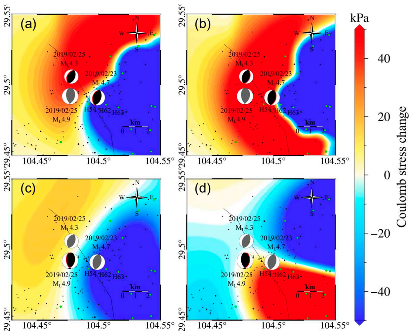
Figure 6. (a) Coulomb stress changes on Rongxian M_L 4.9 two pre-shocks source mechanism plane 1 (strike = 190^\circ , dip = 42^\circ , rake = 83^\circ ) due to reservoir volume changes. (b) Coulomb stress changes on Rongxian M_L 4.9 two pre-shocks source mechanism plane 2 (strike = 19^\circ , dip = 48^\circ , rake = 96^\circ ) due to reservoir volume changes. (c) Coulomb stress changes on Rongxian M_L 4.9 earthquake source mechanism plane 1 (strike = 170^\circ , dip = 51^\circ , rake = 72^\circ ) due to reservoir volume changes. (d) Coulomb stress changes on Rongxian M_L 4.9 earthquake source mechanism plane 2 (strike = 17^\circ , dip = 42^\circ , rake = 11^\circ ) due to reservoir volume changes. Green dots in the figure represent the position of the shale gas production well platforms, and black dots represent the position of the shale gas production well platforms.
