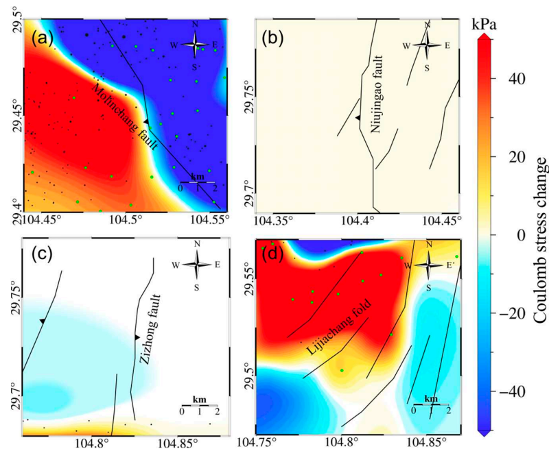
Figure 8. (a) Coulomb stress changes on the Molinchang fault (strike = 150^\circ , dip = 40^\circ , rake = 90^\circ ) due to reservoir volume changes. (b) Coulomb stress changes on the Niujingao fault (strike = 0^\circ , dip = 30^\circ , rake = 90^\circ ) due to reservoir volume changes. (c) Coulomb stress changes on the Zizhong fault (strike = 10^\circ , dip = 20^\circ , rake = 90^\circ ) due to reservoir volume changes. (d) Coulomb stress changes on the Lijiachang fold (strike angle = 45^\circ , dip = 10^\circ , rake = 90^\circ ) due to reservoir volume changes (green dots in the figure represent the position of the shale gas production well platforms, and black dots represent the position of the shale gas production well platforms).
