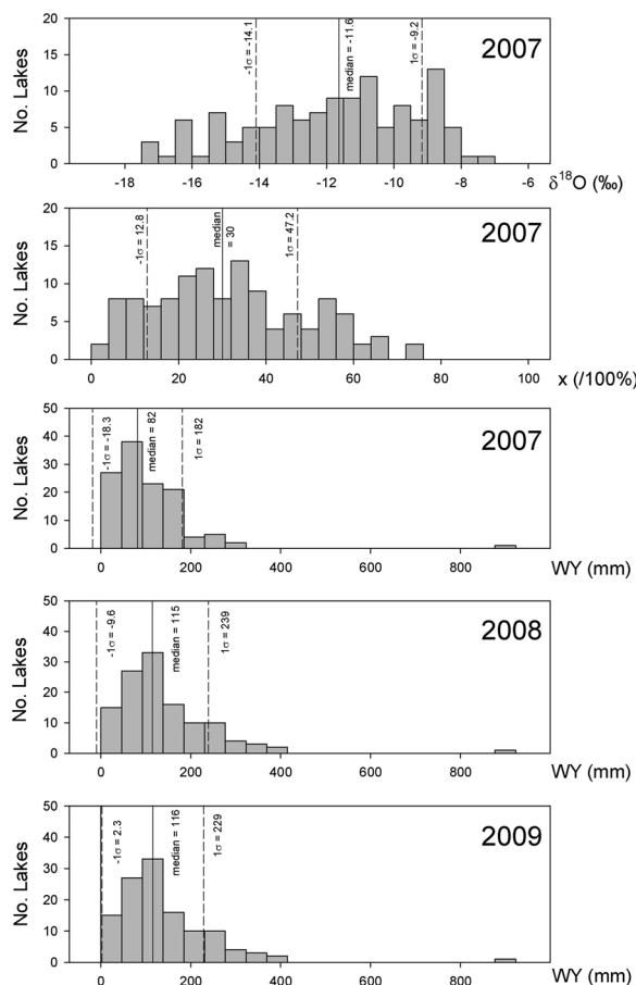
Fig. 4. Histograms of isotope data and selected isotope mass balance outputs, 2007–2009.
