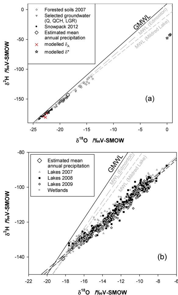
Fig. 2. \delta^{18}O - \delta^2H signatures in (a) measured and modelled parameters, and (b) lakes and fens. Estimated isotopic composition of precipitation is also shown. Global Meteoric Water Line (GMWL) is after Craig (1961); Local Meteoric Water Lines (MWL) for Edmonton and Mildred Lake are after Baer et al. (2016). Q is Quaternary aquifers, QCH is Quaternary channels, LGR is Lower Grand Rapids Fm.
