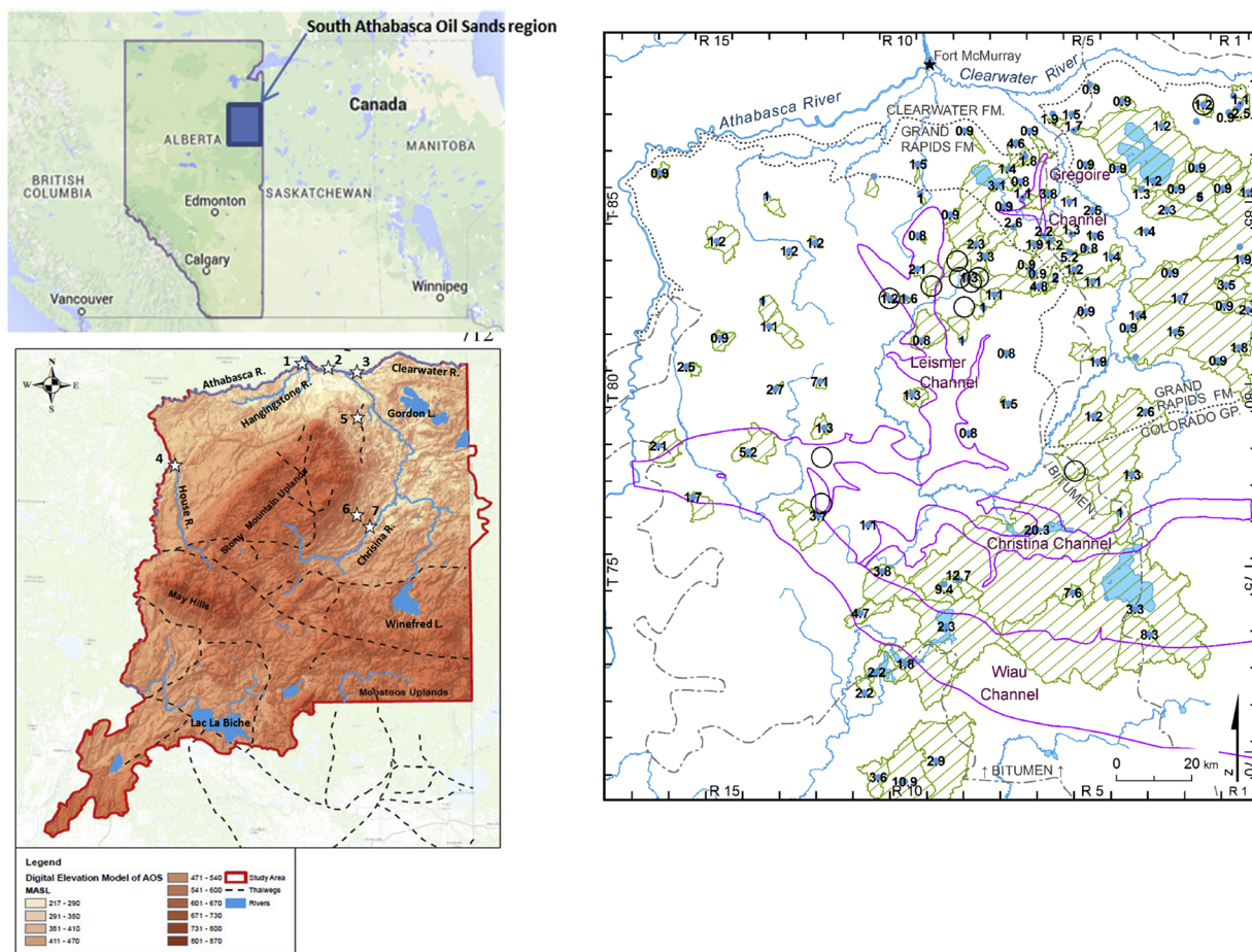
Fig. 1. (a)(top left panel) Location of South Athabasca Oil Sands region, (b) (bottom left panel) elevations and geographical features including gauging stations referred to in the text, (c) (right panel) Location of study lakes within SAOS showing delineated watershed areas and water depth measured during the 2009 sampling campaign. The location of detailed study lakes are indicated with open circles.
