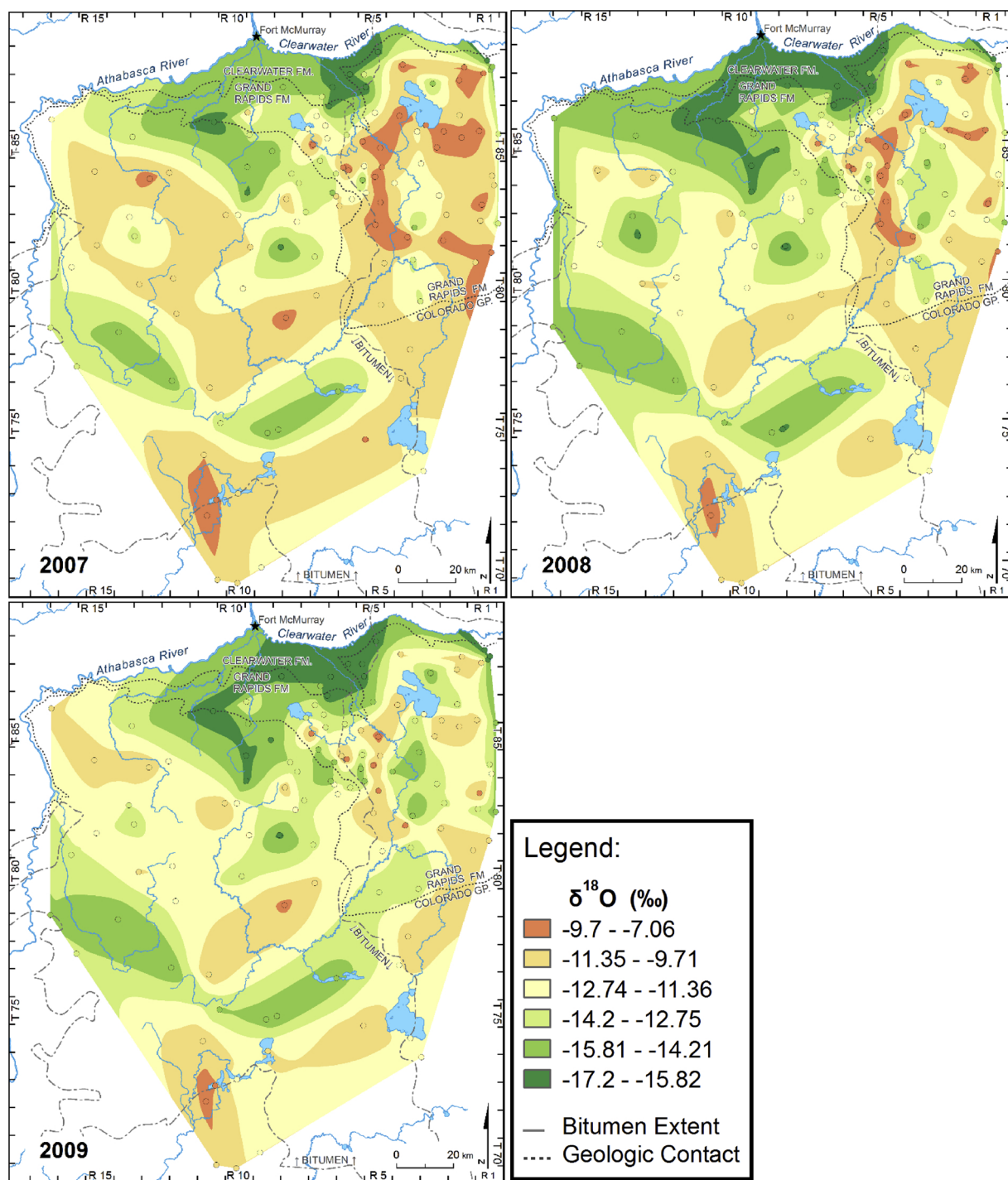
Fig. 3. Spatial distribution of isotopic composition ( \delta^{18}\text{O} , ‰VSMOW) in lakes across the SAOS.2007–2009.
