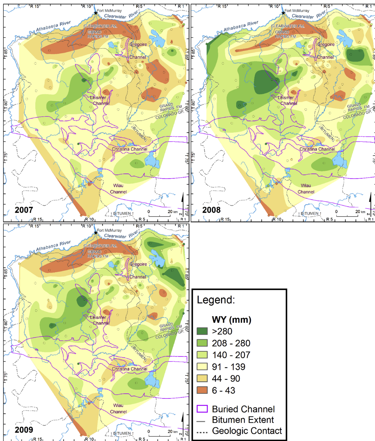
Fig. 5. Spatial distribution of water yield (mm) derived from isotope mass balance of lakes, 2007 to 2009.
