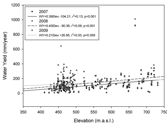
Fig. 6. Weak relationship between water yield and elevation in SAOS.
