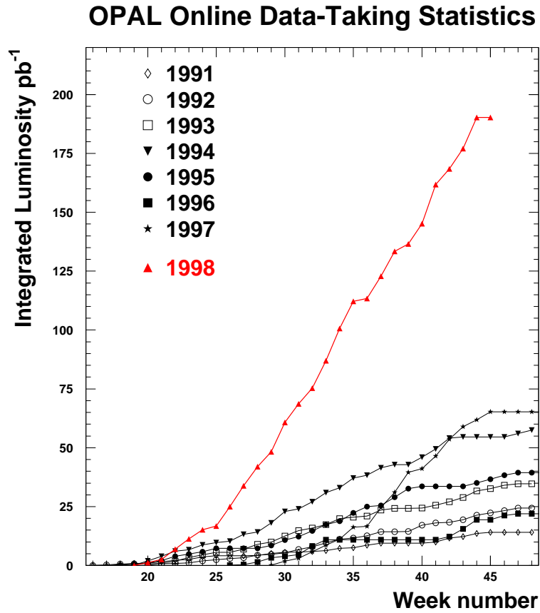
Figure 3.5: The integrated luminosity collected by the OPAL detector as a function of time. The week number is referenced to the LEP start date each year.
