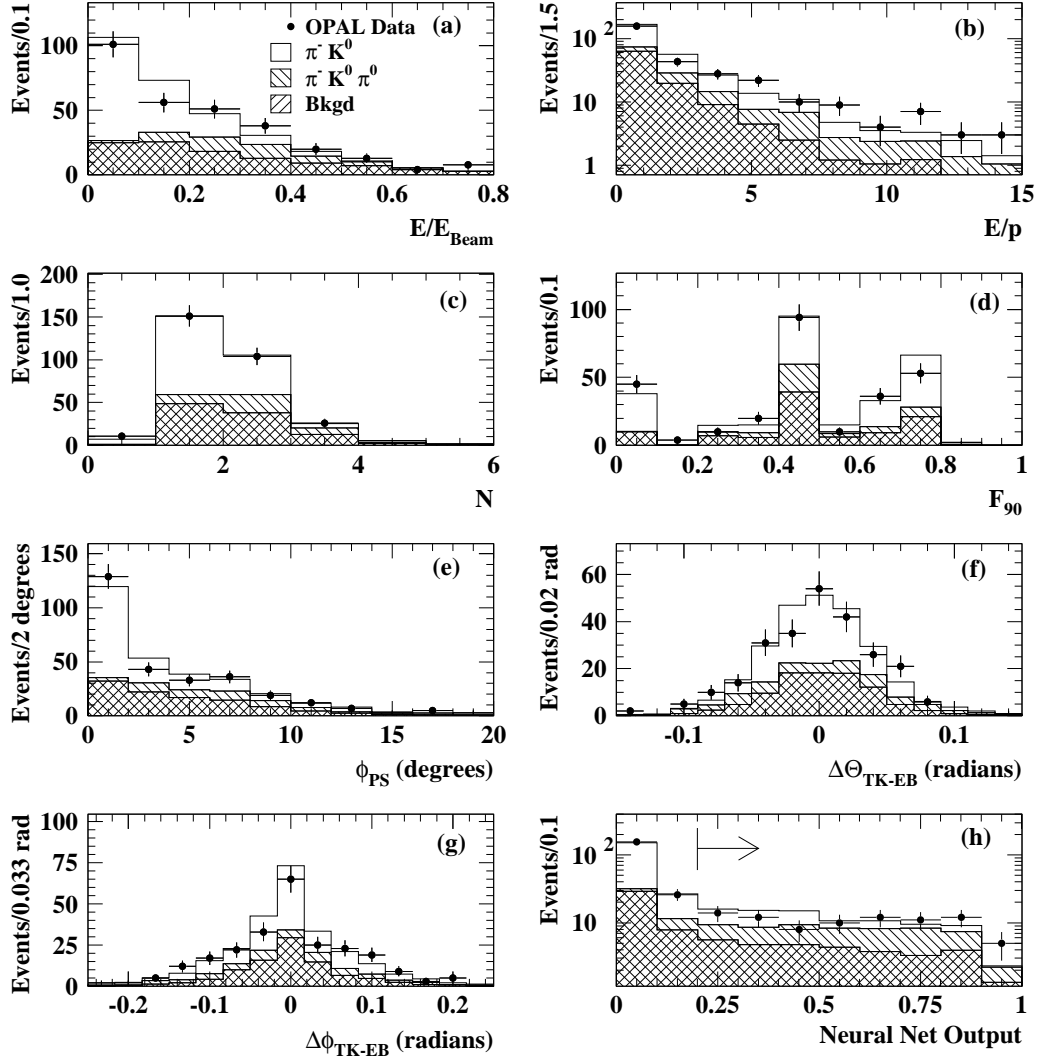
Figure 6.5: The variables used in the neural network routine for identifying \pi^0 mesons in the K_{\text{L}}^0 selection: Histogram (a) shows the electromagnetic energy divided by the beam energy; plot (b) shows the ratio of the electromagnetic cluster energy ( E ) with the momentum of the track ( p ); plot (c) shows the number of electromagnetic calorimeter clusters ( N ); plot (d) shows the fraction of lead glass blocks in the electromagnetic calorimeter with over 90% of the energy in the jet; plot (e) shows angle between the position of the track at the presampler and the presampler cluster furthest away from the jet axis; plots (f) and (g) show the difference in theta ( \Delta\theta ) and phi ( \Delta\phi ) between the track and the vector obtained by adding all the clusters in the electromagnetic calorimeter; and plot (h) shows the output of the neural network.
