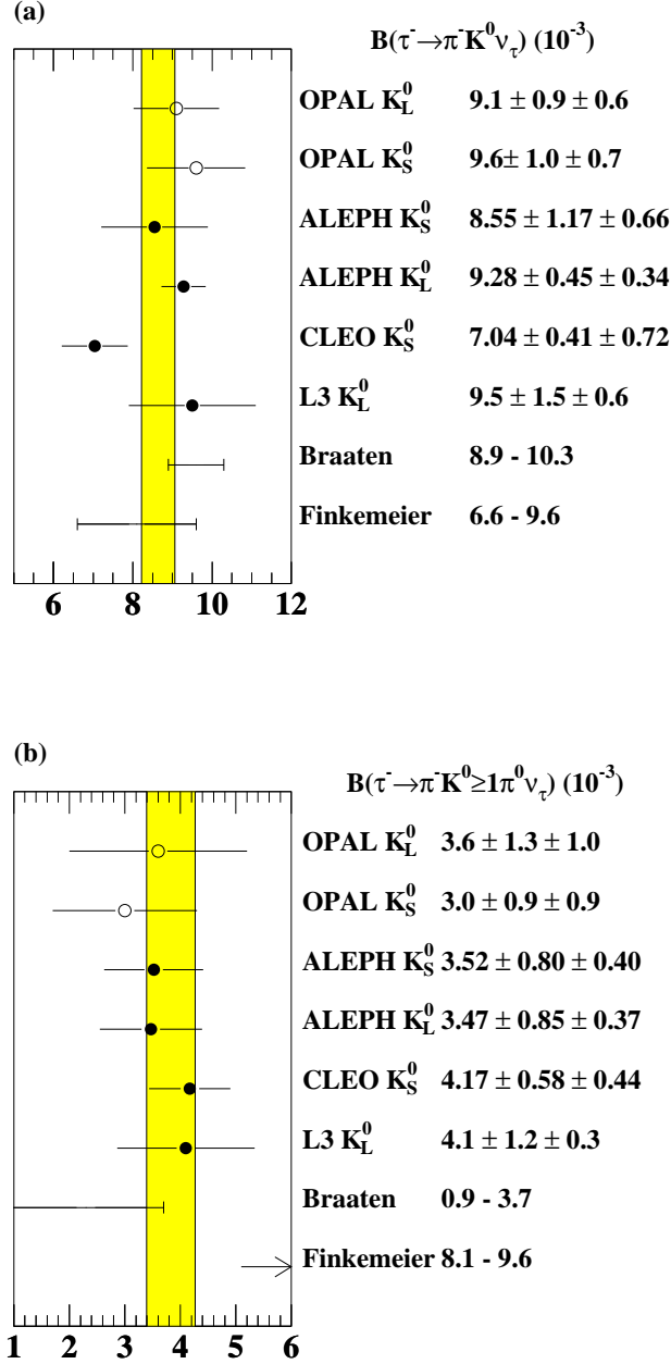
Figure 8.2: Branching ratios of the \tau^- \rightarrow \pi^- \bar{K}^0 \nu_\tau and \tau^- \rightarrow \pi^- \bar{K}^0 \geq 1\pi^0 \nu_\tau decays measured and predicted to date. The solid band is the average branching ratio of the previous measurements. The \tau^- \rightarrow \pi^- \bar{K}^0 \geq 1\pi^0 \nu_\tau results include both the \tau^- \rightarrow \pi^- \bar{K}^0 \pi^0 \nu_\tau and \tau^- \rightarrow \pi^- \bar{K}^0 \pi^0 \pi^0 \nu_\tau measurements. The theoretical estimates are shown for the \tau^- \rightarrow \pi^- \bar{K}^0 \pi^0 \nu_\tau decay mode only. The open points show the new OPAL results, the solid points show other experimental results and the bounded region shows the theoretical predictions of the branching fractions.
