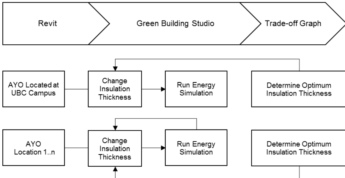
Figure 1: Roadmap diagram
