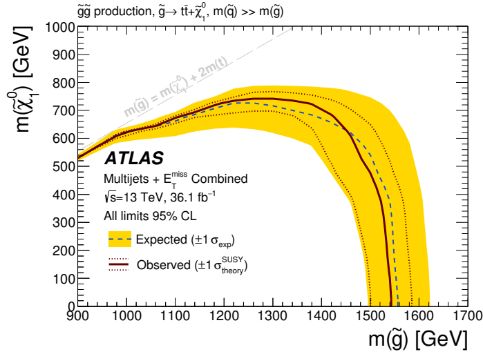
(a) Off-shell top squarks
