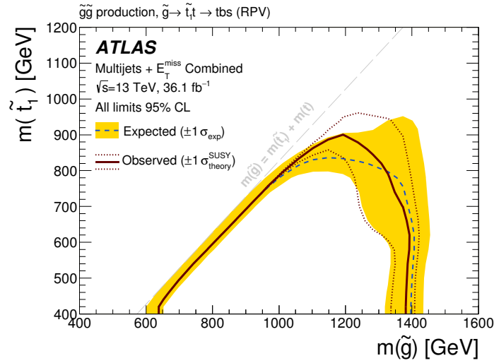
(b) RPV
