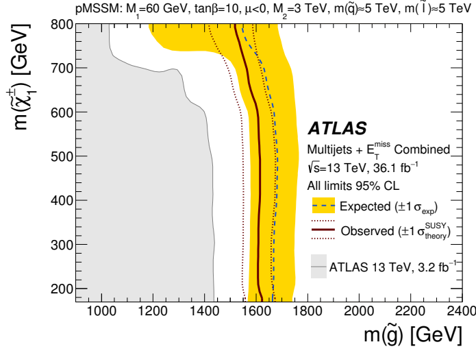
(a) pMSSM
