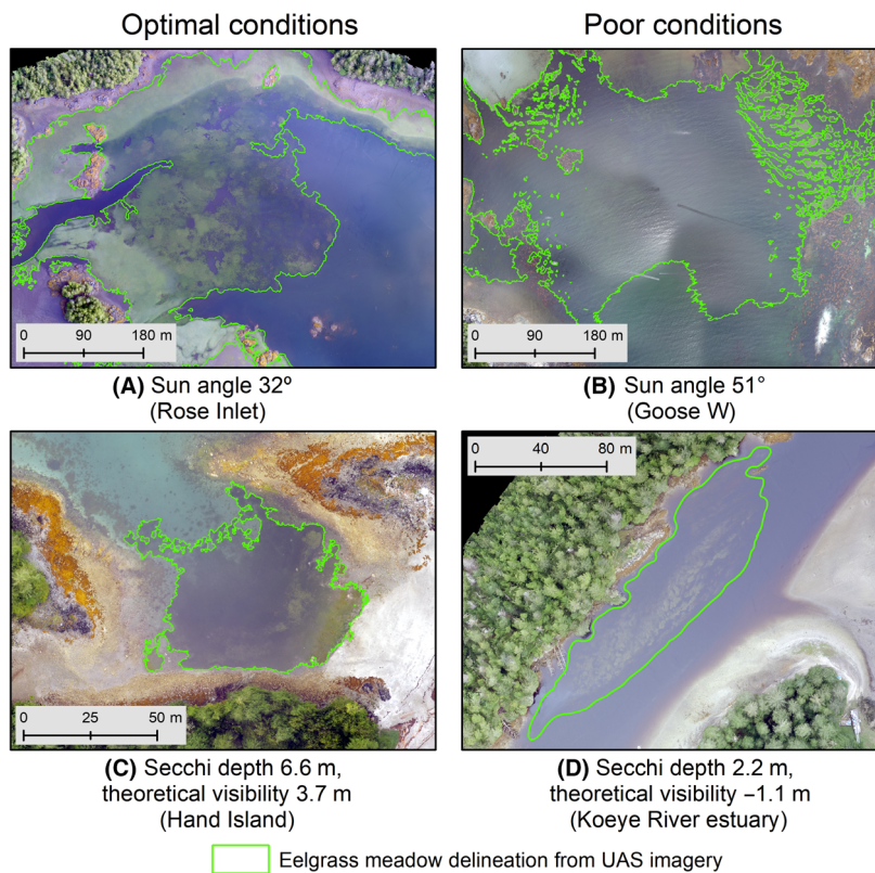
Figure 7. Visual comparisons of sites with optimal and poor sun angle (A and B) and water clarity (C and D) conditions.
