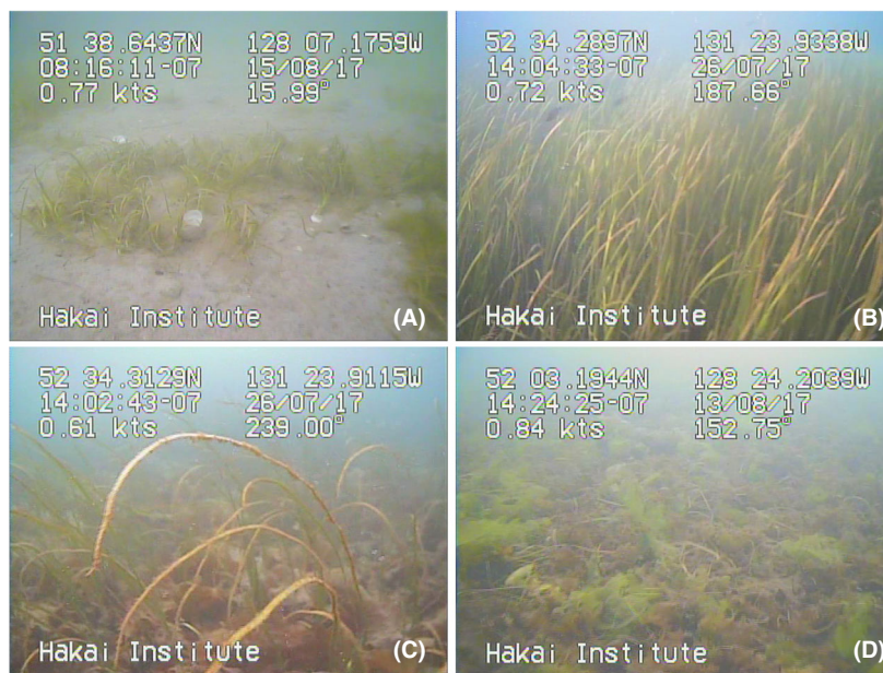
Figure 2. Examples of seagrass and non-seagrass SAV classifications from towed underwater video frames: (A) sparse eelgrass; (B) dense eelgrass; (C) mixed eelgrass with SAV; (D) dense SAV. Imagery is labeled with location, time, date, and speed information at time of acquisition.
