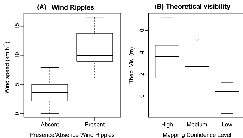
Figure 5. Additional variables, (A) presence or absence of wind ripples; (B) calculated theoretical visibility.
