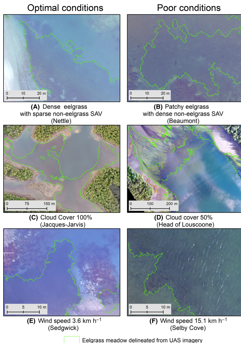
Figure 8. Visual comparisons of sites with optimal and poor conditions in terms of eelgrass density and non-eelgrass SAV presence (A and B), cloud cover (C and D), and wind speed (E and F) conditions.
