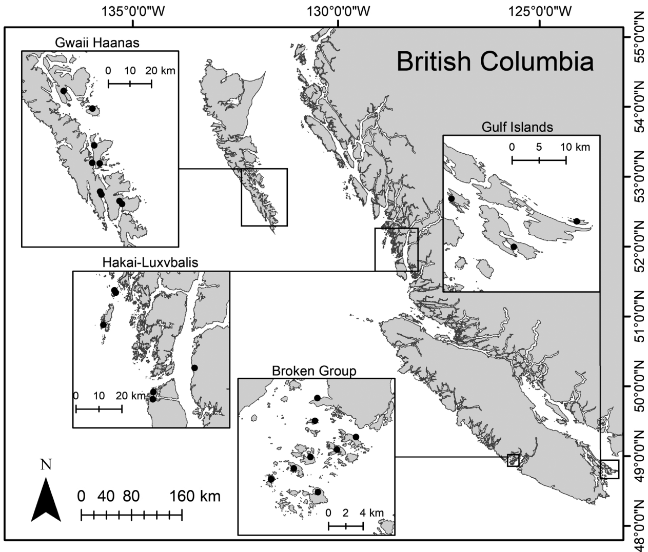
Figure 1. Location of eelgrass mapping sites in each of four study regions in British Columbia: Gwaii Haanas, Haida Gwaii, north coast; Hakai-Luxvbalis, central coast; Gulf Islands, south-east coast; Broken Group, Pacific Rim National Park and south-west coast
