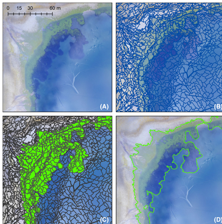
Figure 3. Example of eelgrass delineation process (site: Bag Harbour, GHNMCA): (A) original orthomosaic; (B) orthomosaic segmented into image objects; (C) image objects representing eelgrass manually selected based on photointerpretive characteristics; (D) classified image objects exported and merged to create final eelgrass delineation.
