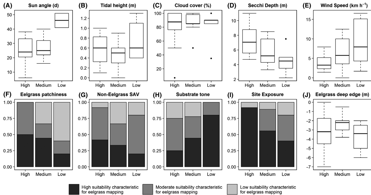
Figure 4. Environmental conditions (A–E) and site characteristics (F–J) plotted on the y-axis against Mapping Confidence Level across all x-axes (High, Medium, or Low confidence in eelgrass mapping output). For quantitative environmental or site characteristics, the center line of the boxplot represents the median, and the whiskers extend 1.5 times the interquartile range above and below the upper and lower quartile. For qualitative site characteristics, the right-hand y-axis represents the proportion of sites in each confidence level category. Raw data is provided in Appendix A1.
