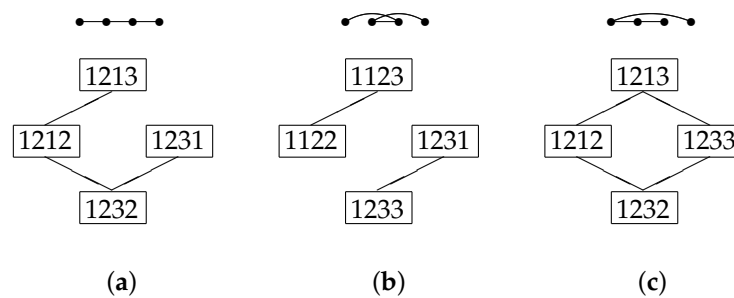
Figure 1. Three different vertex orderings of P_4 with associated \text{Can}_3^\pi(P_4) . In each case the colourings are canonical with respect to the given vertex ordering from left to right.
