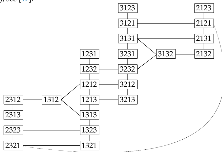
Figure 2. \mathcal{C}_3(P_4) , the 3-Colouring Graph of P_4 . The vertices are labeled by the colourings of the path.
