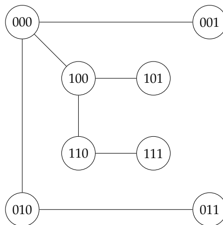
Figure 4. The tree \text{Can}_6^\pi(T_{6,3})
