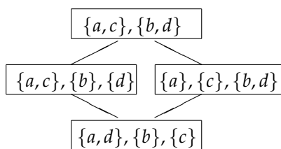
Figure 3. \mathcal{B}_3(P_4) , the 3-Bell colouring graph of P_4 . The vertices are labeled by the partition of the path abcd .
