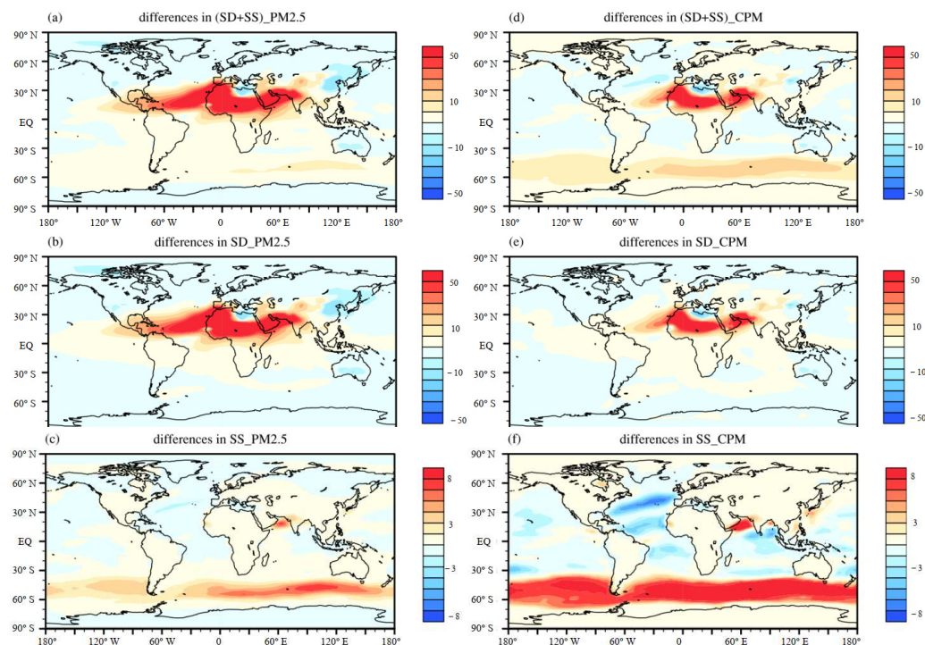
Figure 6. Global distributions of changes in annual mean column concentrations of natural \text{PM}_{2.5} and CPM in JJA, caused by 4 \times \text{CO}_2 -induced global warming (units: \text{mg m}^{-2} ). Plots in the left column represent changes in the annual mean column concentrations of natural \text{PM}_{2.5} , SD ( \text{PM}_{2.5} ), and SS ( \text{PM}_{2.5} ), respectively; plots in the right column represent those of natural CPM, SD (CPM), and SS (CPM), respectively.
