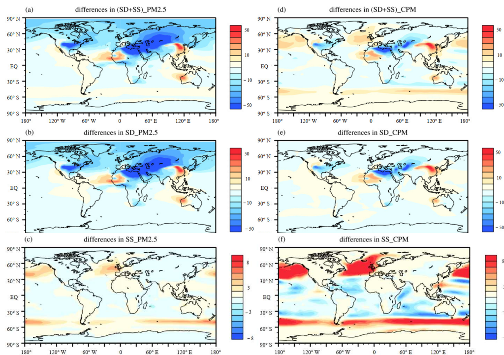
Figure 7. As described for Figure 6, but showing changes in the annual mean column concentrations of natural \text{PM}_{2.5} and CPM in DJF, caused by 4 \times \text{CO}_2 -induced global warming (units: \text{mg m}^{-2} ).
