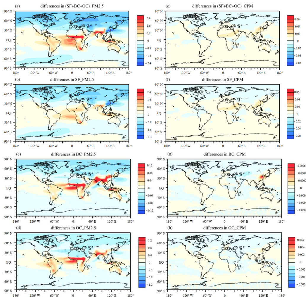
Figure 5. As described for Figure 4, but showing changes in the annual mean column concentrations of anthropogenic PM 2.5 and CPM in DJF, caused by 4 \times \text{CO}_2 -induced global warming (units: \text{mg m}^{-2} ).
