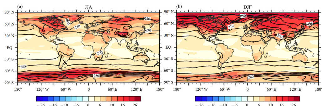
Figure 1. Color contours on the maps indicate the changes in the spatial distributions of annual mean surface air temperature (SAT, units: K) in (a) summer (JJA) and (b) winter (DJF), caused by 4 \times \text{CO}_2 -induced global warming; plots in the left column are simulated results during JJA, whereas plots in the right column are those during DJF; the solid line contours show SAT in the experiment of 1 \times \text{CO}_2 .
