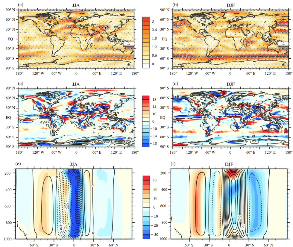
Figure 2. Color contours on the maps show changes in surface horizontal wind (a,b) (the shaded areas representing the wind speed, units: \text{m s}^{-1} ), horizontal divergence of surface wind (c,d) (units: \text{m s}^{-2} ), and stream function of vertical atmospheric circulation (e,f) (units: 10^{-11} \text{ kg s}^{-1} ) during both JJA and DJF, respectively, caused by 4 \times \text{CO}_2 -induced global warming; plots in the left column are simulated results during JJA, whereas plots in the right column are those during DJF; the solid line contours show horizontal divergence of surface wind (c,d) and stream function of vertical atmospheric circulation (e,f) in the experiment of 1 \times \text{CO}_2 .
